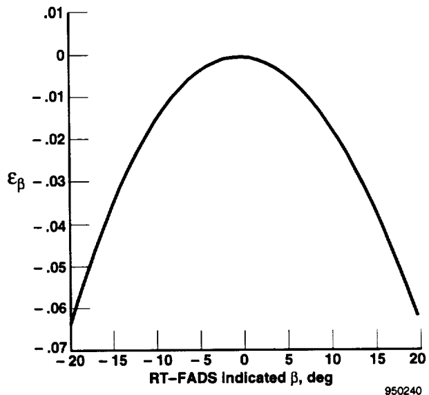
(c) Variation with angle of sideslip.
