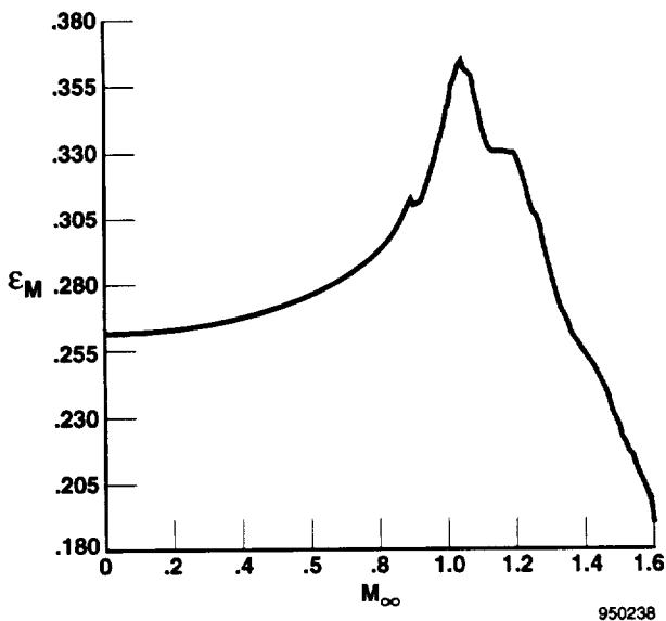
(a) Variation with Mach number.
