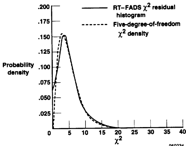
(b) Normalized residual sum.
