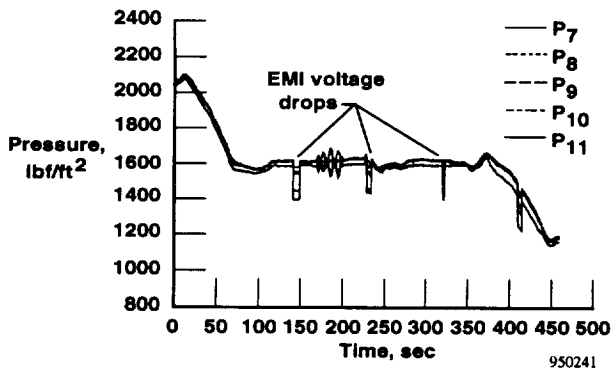
(a) Corrupted pressure data.
