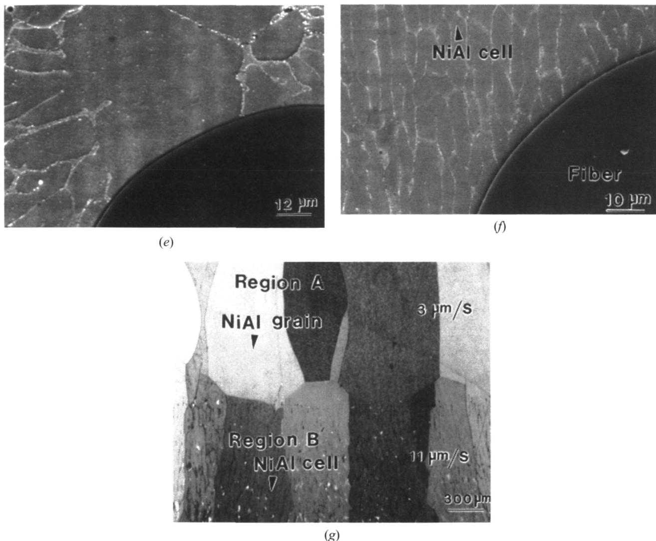
Fig 1.—(continued): Fiber-matrix interface in (a) AC sapphire-NiAl(Cr); (b) fiber-matrix interface in the DS sapphire-NiAl(Cr); (c) microstructure of DS NiAl(Cr) showing intercellular Cr eutectic and Cr precipitates within NiAl cells; (d) high magnification view of the interface region in the DS sapphire-NiAl(Cr) showing the two types of fiber surroundings (marked C and D) and the excellent bonding between eutectic chromium and sapphire. (e) AC sapphire-NiAl(W) and (f) DS sapphire-NiAl(W) showing cellular matrix structure and absence of preferential deposition of W-rich phases on sapphire; and (g) typical longitudinal view of a DS NiAl(W) specimen showing columnar NiAl grains and cellular microstructure, corresponding to two different growth speeds.
