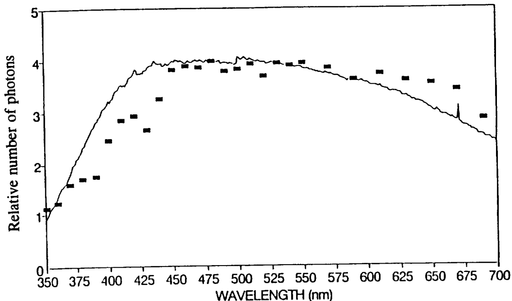
Fig. 7. Sulfur flux X in (continuous line) compared with the sun (discrete points). The ordinate is proportional to the number of photons per second.
