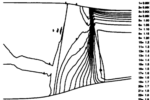
Body Forces Updated in Throughflow Analysis Conforming to Streamsurface from 3-D Solution
