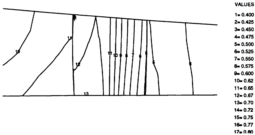
Figure 7.8: The Mach number contours from the converged TADS analysis and the axisymmetric average of the full 3-D solution are in good agreement both inside and outside the bladed region.
