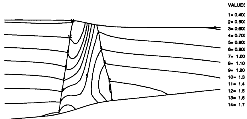
Axisymmetric Average of Full 3-D Euler Solution
