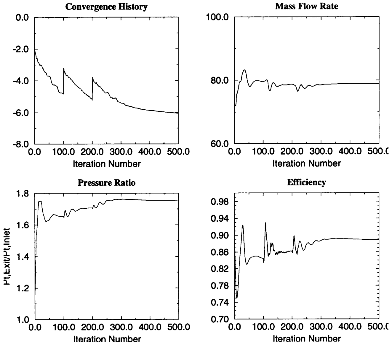
Figure 4.11: Convergence history for ADPAC based throughflow analysis applied to NASA Rotor 67.
