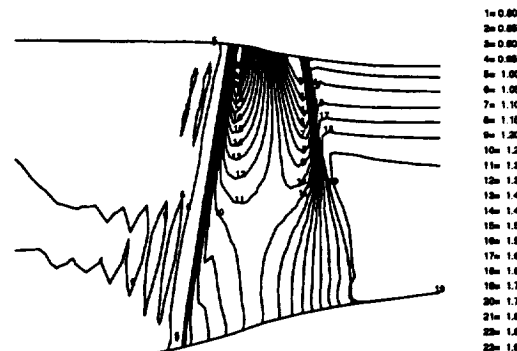
Body Forces Updated in Throughflow Analysis Conforming to Streamsurface from Mean Camber Line and Carter's Rule
