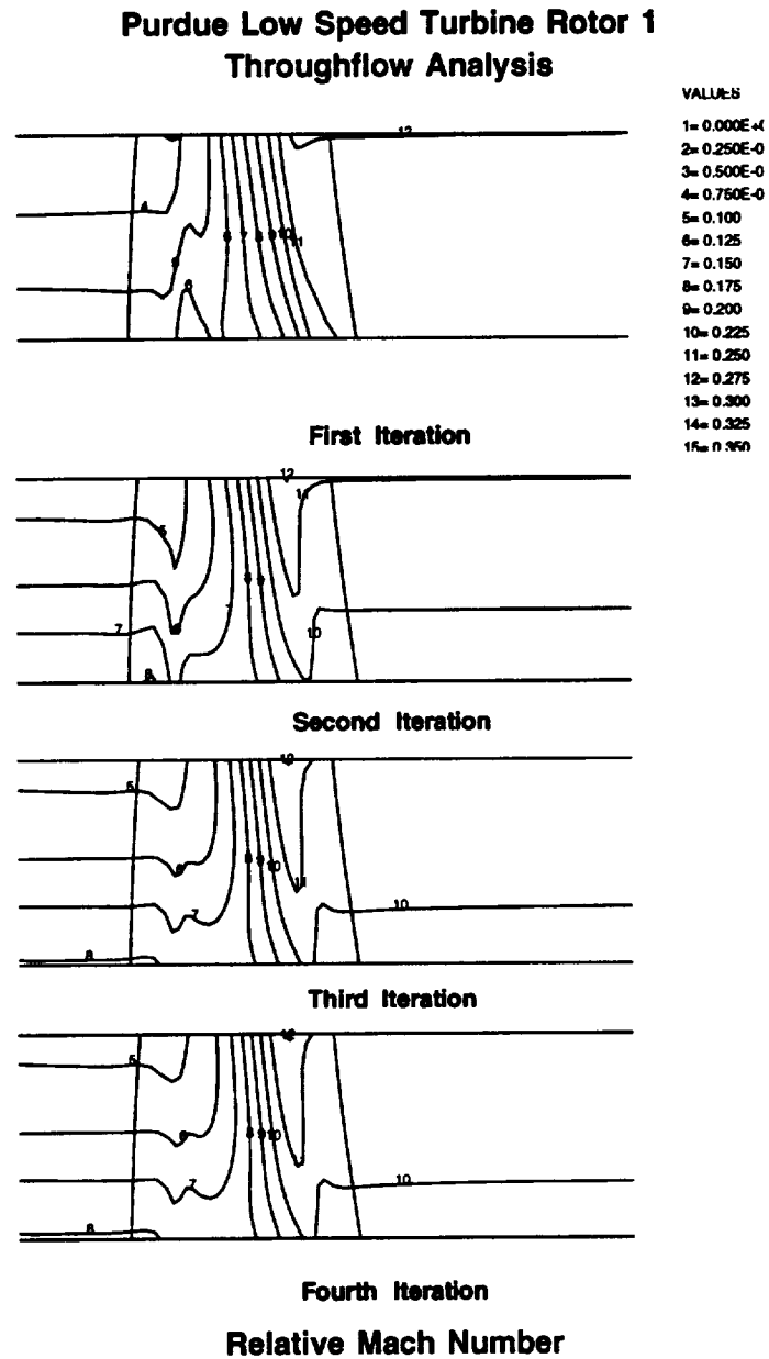
Figure 7.13: The relative Mach number contours from each iteration show that the TADS system is converged after three iterations.
