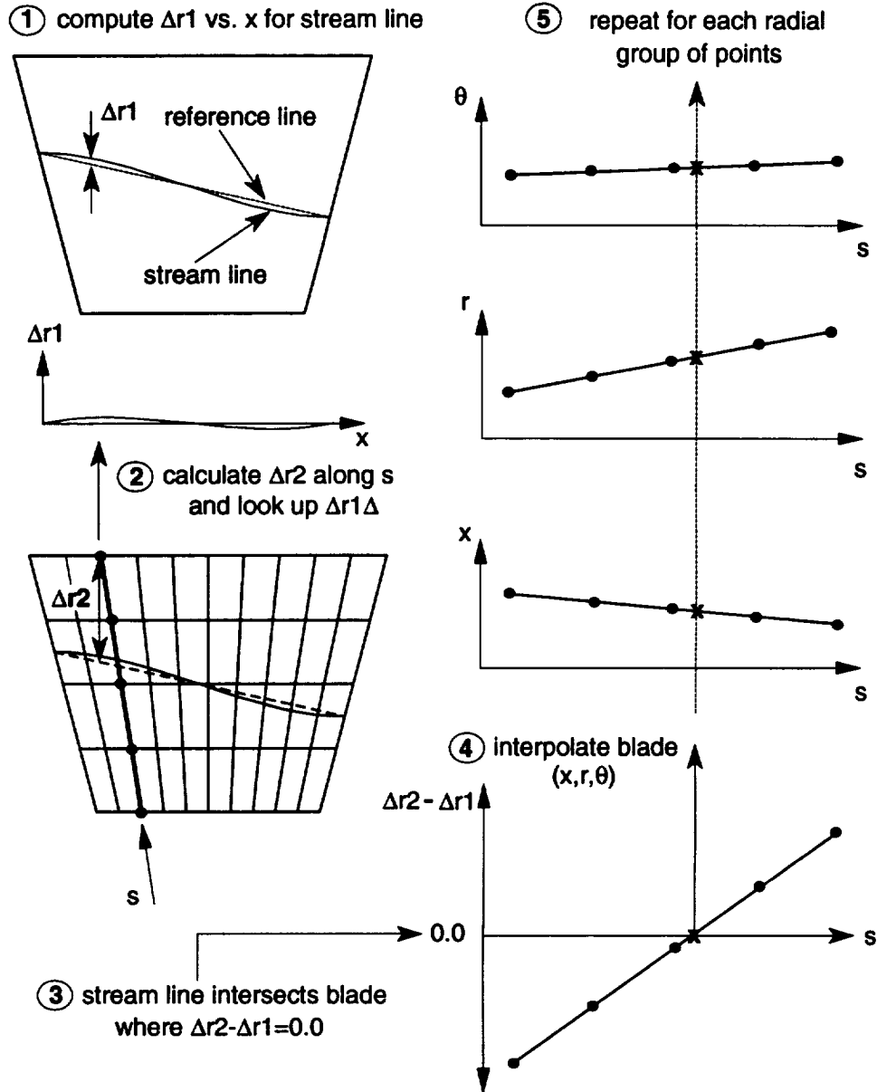
Figure 4.4: The airfoil thickness is determined by an interpolation procedure which handles differences in airfoil descriptions.
