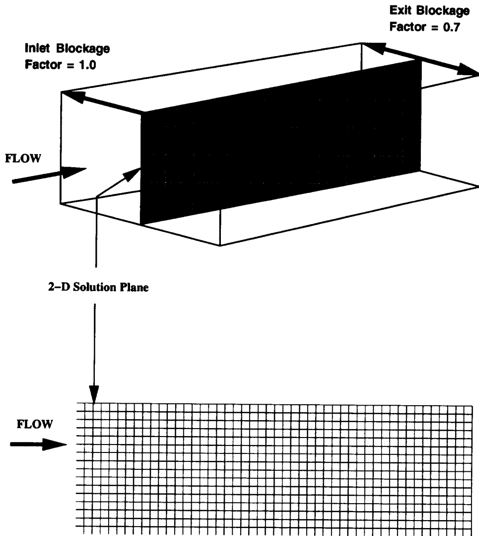
Figure 4.6: Simple channel flow with linear variation in cross sectional area results in a linear variation of the blockage term \lambda .
