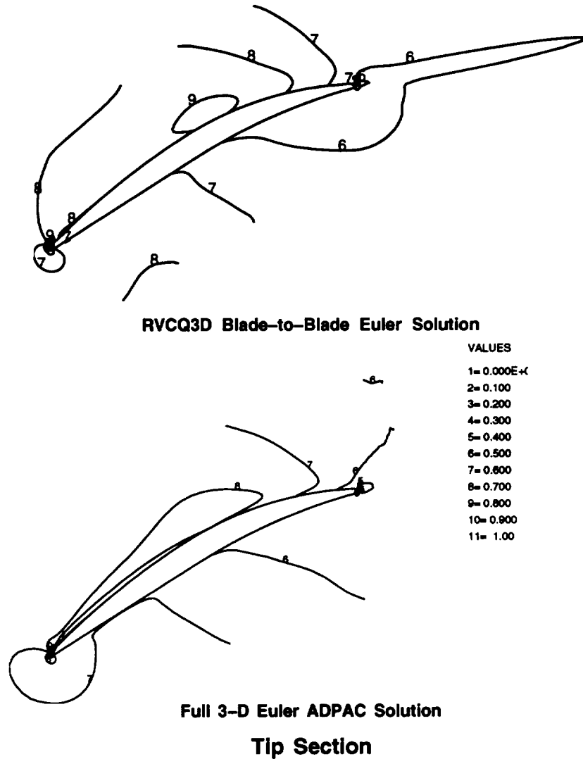
Figure 7.12: The Mach number contours at the tip section are in good agreement. The quasi-3D solution is at a slightly higher flow rate than the 3-D Euler section.
