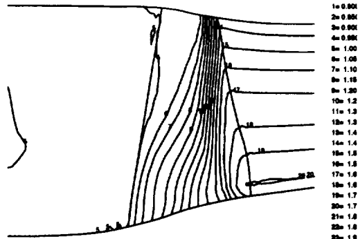
Body Forces Computed From 3-D Solution Imposed in Throughflow Analysis
