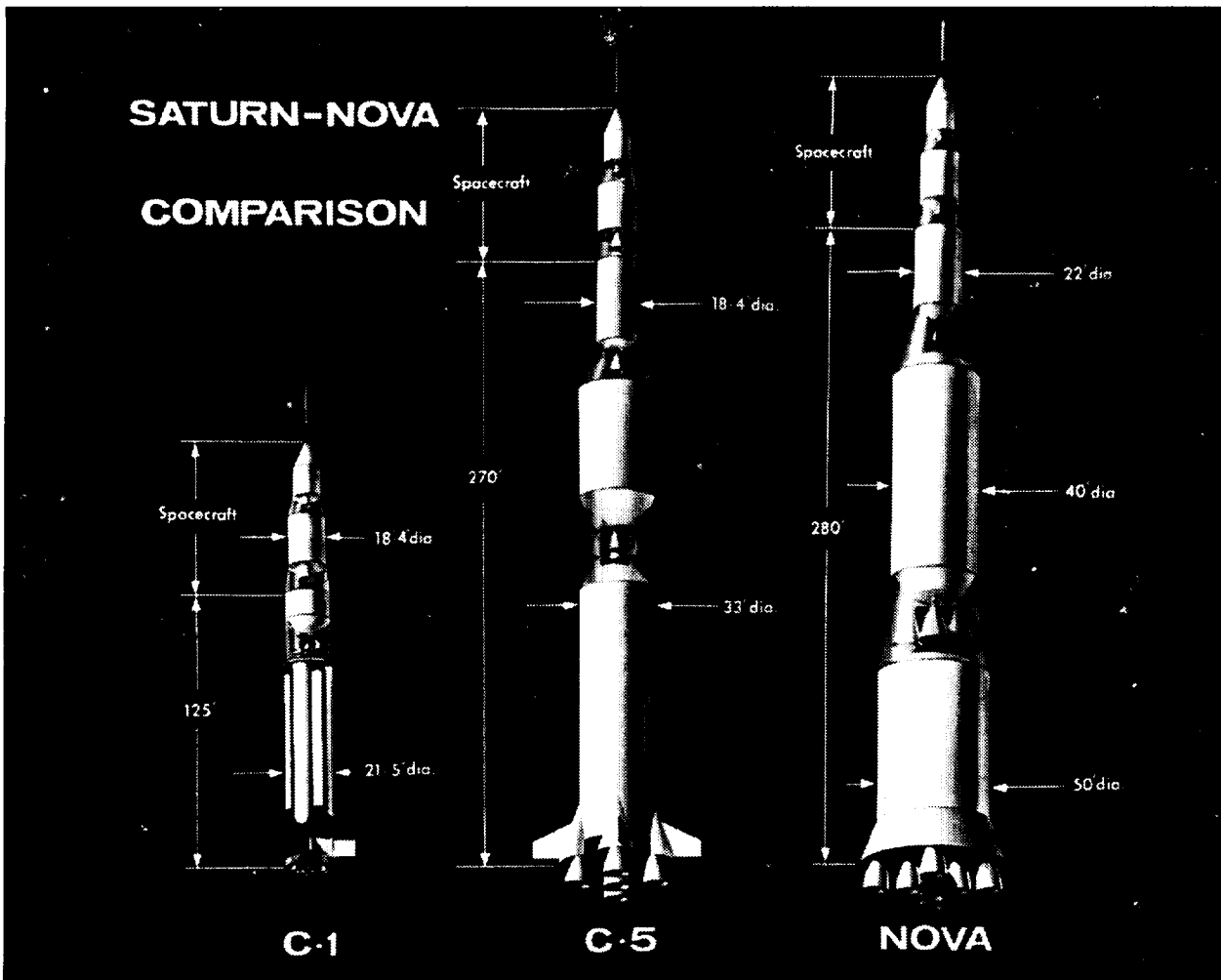
A comparison of the proposed mammoth Nova rocket with the very large Saturn C-5 and C-1 launch vehicles.
