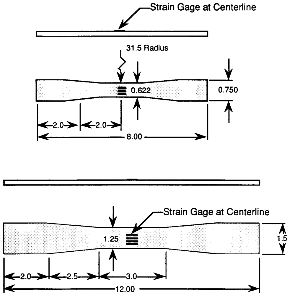
Figure 11. Compression Specimens used at Lockheed.
