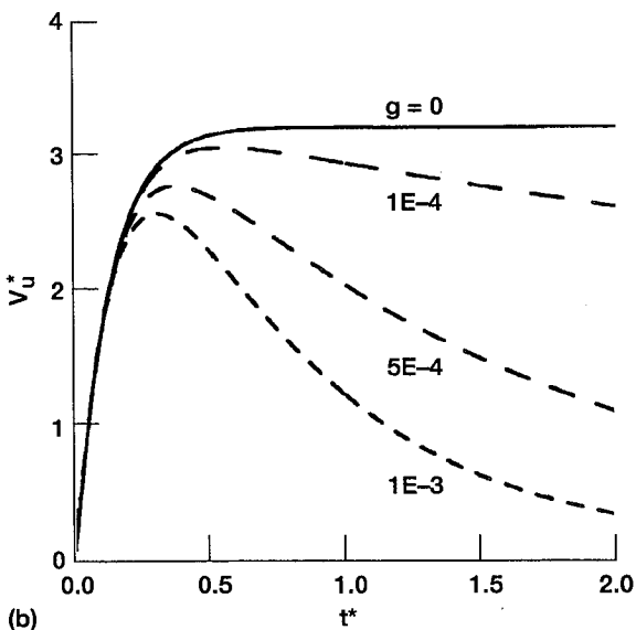
Figure 4a.— h^* , and 4b. V_U^* , versus t^* , respectively, for the U-tube configuration: effect of finite acceleration field, g ( m/s^2 ).
