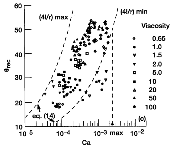
Figure 15.—Ca dependence of (a) \theta_{adv} ID indicated, (b) \theta_{adv} viscosity indicated, and (c) \theta_{rec} viscosity indicated for factory cleaned (D) straight tubes.
