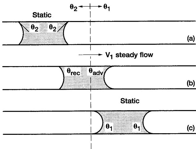
Figure 1.—Schematic of steady flow resulting from a discontinuous wetting condition on the interior of a circular tube of constant radius where \theta_1 < \theta_2 .
