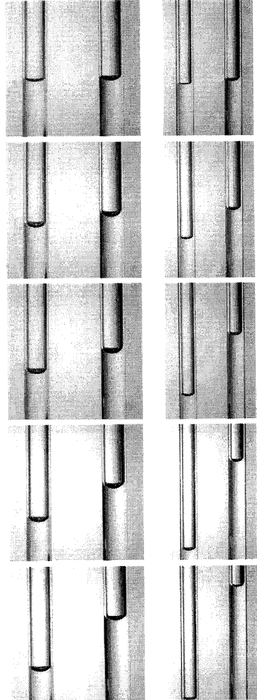
Figure 5.—Selected frames from two U-tube drop tower tests, \nu = 1cS . Time progression is top to bottom in 0.5s increments, U-portion of tubes not pictured, and left legs of U-tubes are coated. [Left: r = 2.97 , l = 121 , L = 192 mm, V_U = 8.1 mm/s. Right: r = 1.90 , l = 115 , L = 186 mm, V_U = 3.2 mm/s.]
