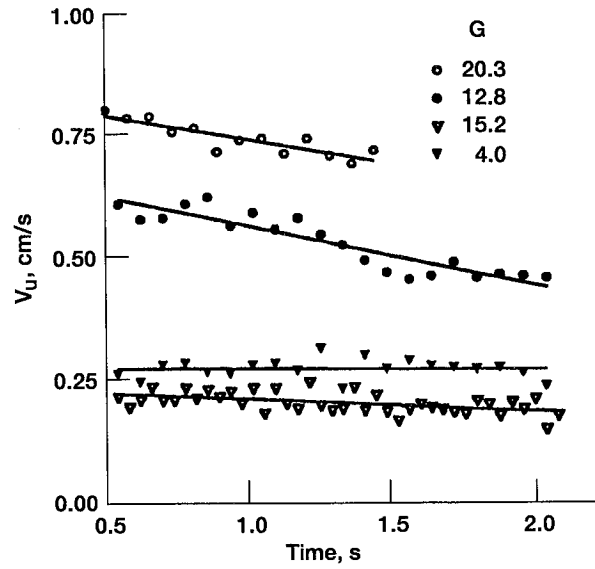
Figure 9.—Instantaneous velocity of liquid slug versus time for U-tube tests of fig. 8. Symbols are consistent with test conditions.
