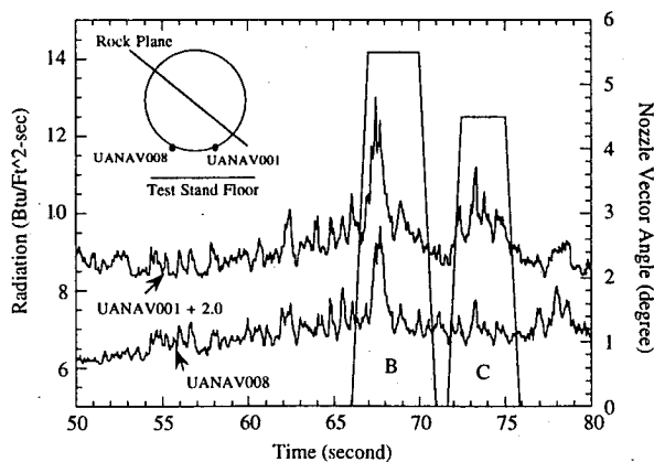
Figure 7. Significant Radiation Spike Measured Only by Nozzle Radiometer Mounted Adjacent to Rock Plane in Lower Half of Nozzle During TEM-11 Rock Event C.
