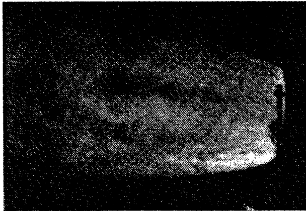
Figure 5b. Ejection of Hot, Bright Slag Near Bottom of Nozzle During 11 psi Pressure Perturbation at 68 Seconds in TEM-11 Test. These Ejecta were Localized and Continuous During Short Intervals. Still Frame from 2000 Frames/Second Camera Located on the North Side 300 Feet from the Nozzle.
