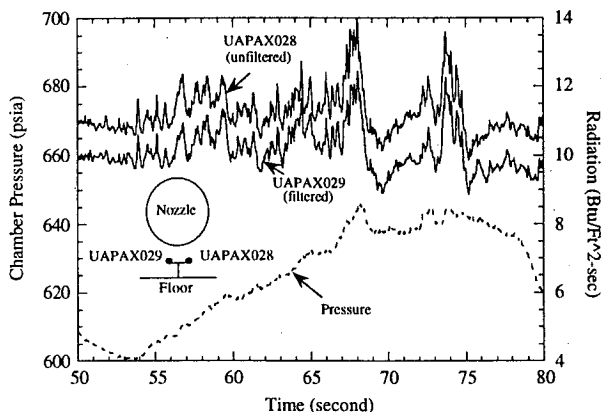
Figure 9. Radiative Flux Measured by 50-Degree, Fast-Response Radiometers in FSM-4 Test.
