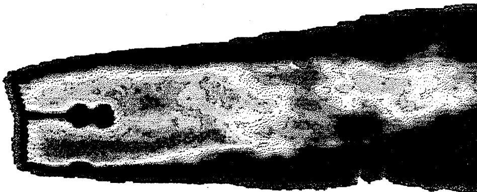
Figure 10b. Plume Thermal Image at 67.6 Seconds During the 11-psi Chamber Pressure Perturbation in the TEM-11 Test. The Nozzle Is Vektored to a 5.5-Degree Pitch. Hotter Emissions from the Ejecta in the Plume Near the Bottom of the Nozzle Exit Plane.
