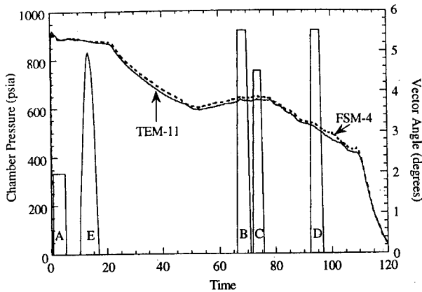
Figure 4a. Chamber Pressure Traces for TEM-11 and FSM-4 Tests.
