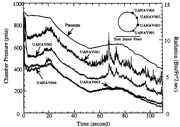
Figure 6a. TEM-11 Nozzle Wall Radiometer Heat Fluxes. Radiometers Mounted on Nozzle Top Half Were Quiescent During Motor Burn While Radiometers on Bottom Half Were Noisier with Distinct Radiation Spikes.
