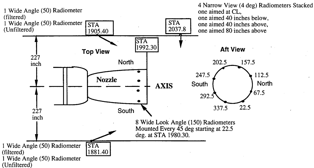
Figure 3. TEM-11 Static Firing Radiometer Arrangement To Support the Pressure Perturbation Studies.
