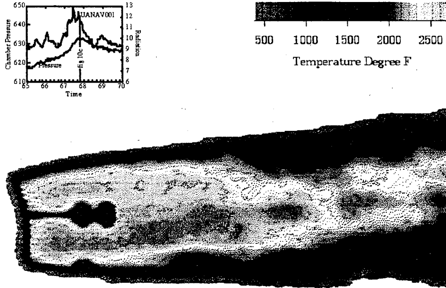
Figure 10c. Plume Thermal Image at 67.8 Seconds During the 11-psi Chamber Pressure Perturbation in the TEM-11 Test. The Nozzle Is Still Vected to a 5.5-Degree Pitch. Hotter Emissions from the Ejecta in the Plume Still Observed Near the Bottom of the Nozzle Exit Plane.
