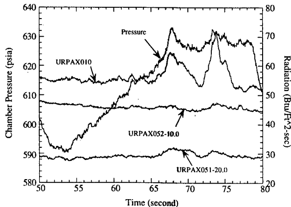
Figure 8. Radiative Fluxes Measured by 4-degree Narrow View Radiometers in TEM-11 Test. The Measured Fluxes are Shifted by Increments of 10 Btu/ft 2 -sec for Clarity.
