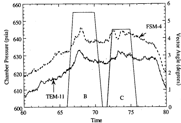
Figure 4b. Chamber Pressure Traces in the 60- to 80-Second Time Frame for TEM-11 and FSM-4 Tests Showing the Pressure Perturbations During Vectoring Events B and C.
