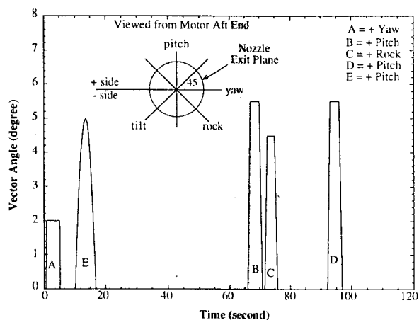
Figure 2. Nozzle Vectoring Employed in TEM-11 and FSM-4 Test To Induce Expulsion of Slag. (Event E was added to FSM-4.)
