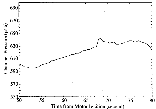
Figure 1. Chamber Pressure Perturbation in Right-Hand RSRM During STS-54 Launch.
