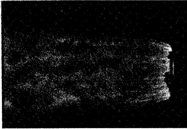
Figure 5a. Quiescent Plume Before Nozzle Vectoring Event B at 66 Seconds in TEM-11 Test. Still Frame from 2000 Frames/Second Camera Located on North Side 300 Feet from Nozzle.
