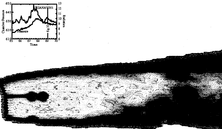
Figure 10d. Plume Thermal Image at 69.0 Seconds After the 11-psi Chamber Pressure Perturbation Event in the TEM-11 Test. The Nozzle Is Still Held in the 5.5-Degree Pitch Position. No Unusual Hot Emissions Observed in the Plume.
