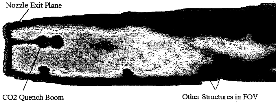
Figure 10a. Plume Thermal Image at 65.5 Seconds Before the 11-psi Chamber Pressure Perturbation in the TEM-11 Test. The Nozzle Is at Null Position. No Unusual Hot Emissions Noticed in the Plume. The Color Scale Provided Above Applies to All the Following Thermal Images in This Report.
