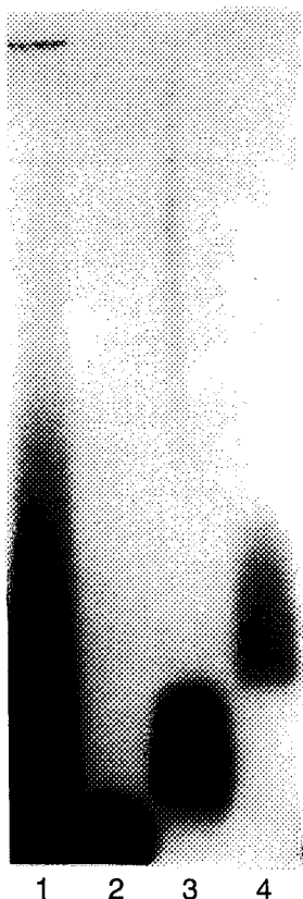
Fig. 5. Gel electrophoretogram of the products obtained by heating ^3\text{P}T_8 -urea with HBSA (lane 1) and the lower (lane 2), middle (lane 3), and upper (lane 4) sections of lane 1, reelectrophoresed after elution from the original gel.
