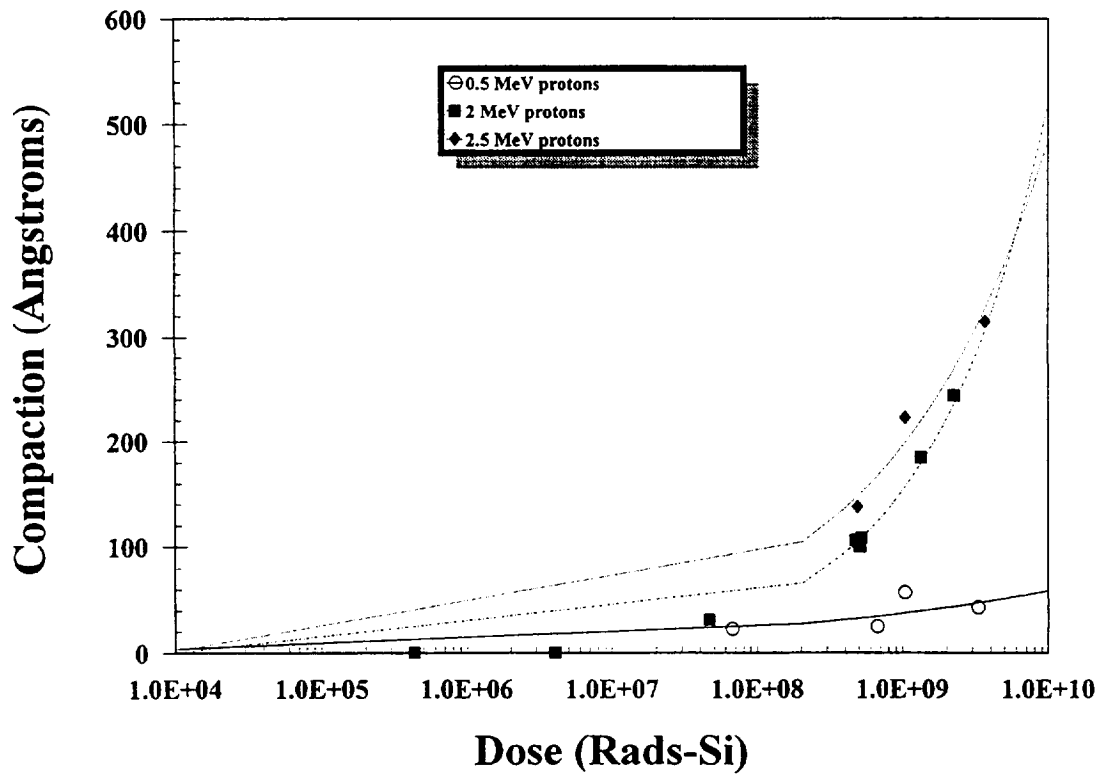
Figure 4. Proton-induced compaction of Zerodur™ exposed to a flux of 5 \times 10^{10} protons/cm 2 s.
