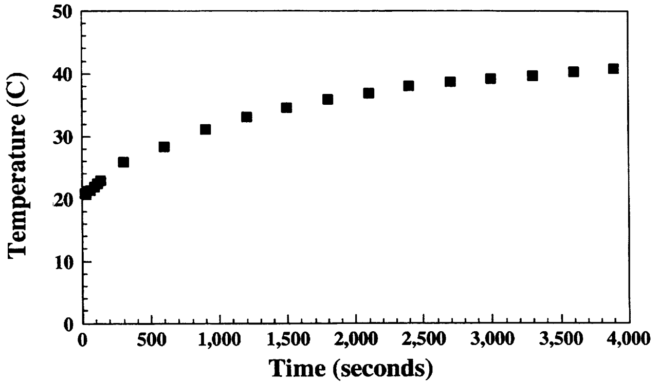
Figure 1. Increase in Zerodur™ surface temperature exposed to 2.0 MeV protons at 175 \times 10^{11} protons/cm 2 s.
