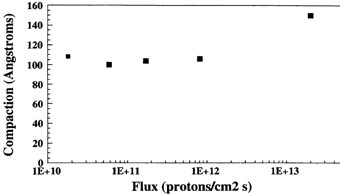
Figure 3. Relationship between the compaction of Zerodur™ and 2.0 MeV proton flux. The fluence for this test was 1.74 \times 10^{14} protons/cm 2 .
