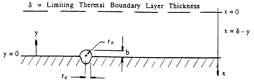
Figure 2.2a Pre-existing vapor nucleus protruding from a cavity
