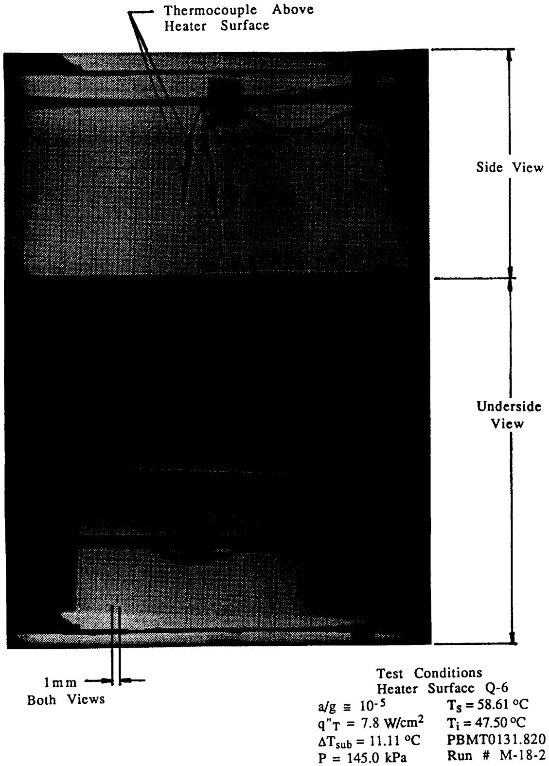
Figure 5.26a Category F: the initial bubble at the edge of the heater surface, time = 0.513 sec
