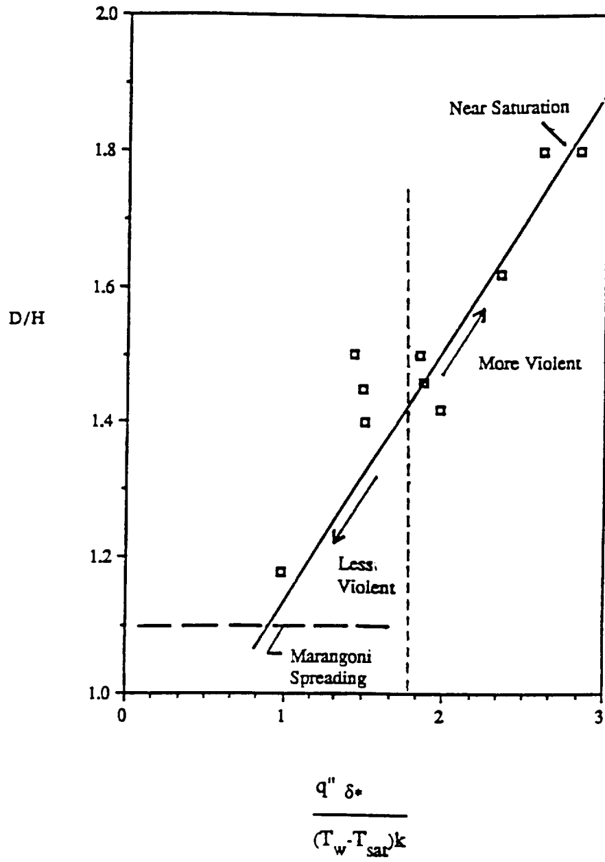
Figure 6.17 Bubble shape at onset of categories D and E in microgravity
