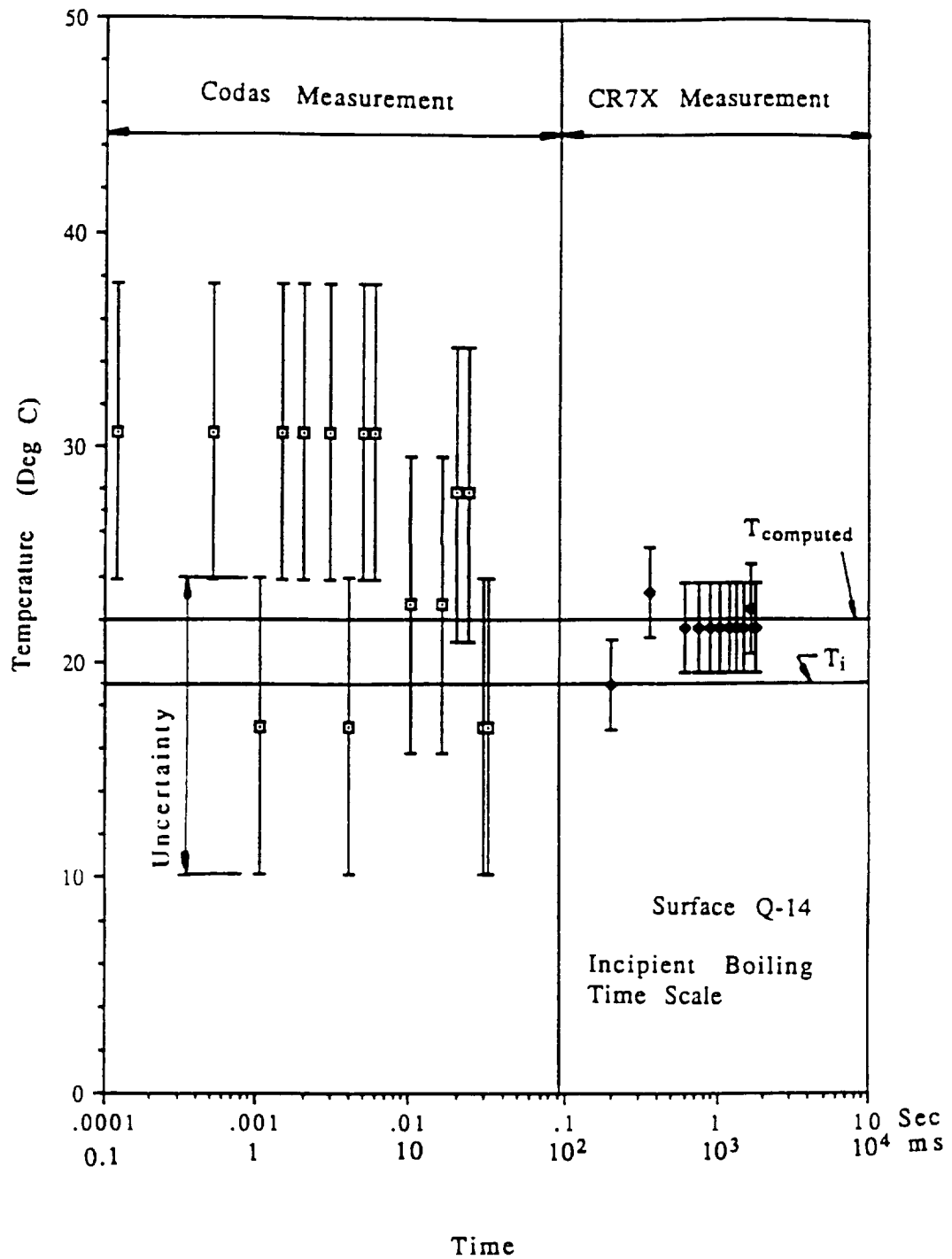
Figure 5.27 Demonstration of transient thin gold film temperature measured with the Codas and the CR7X systems
