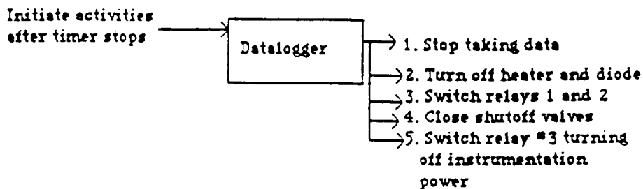
Figure 4.1 Sequence of events during a free fall microgravity test in the NASA Lewis RC drop tower
