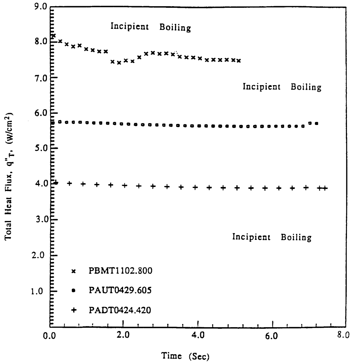
Figure 5.11 Representative measurements of the constant imposed total heat flux from the laboratory and drop vessels
