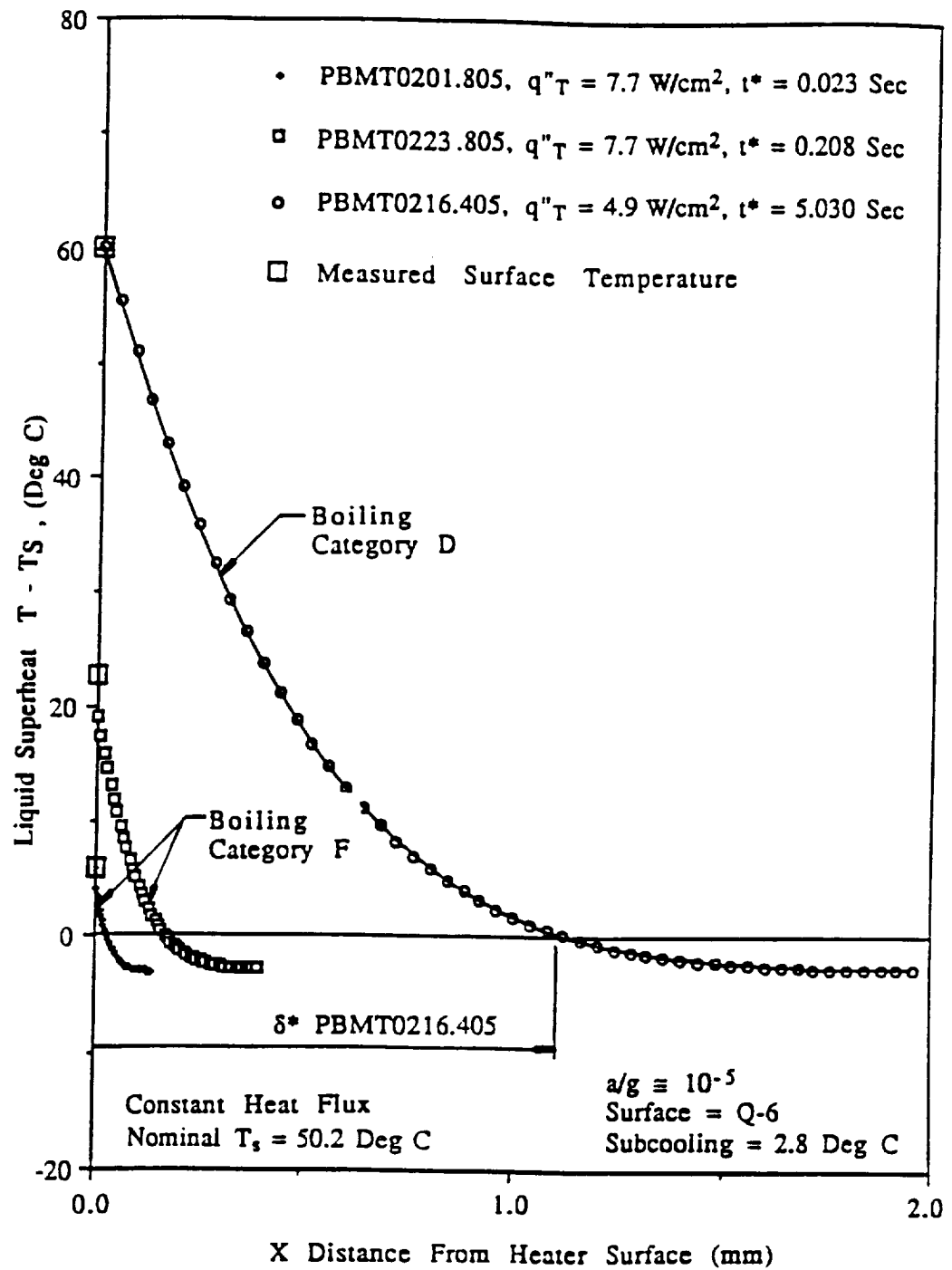
Figure 6.4 Computed liquid superheat in microgravity from imposed heat flux at boiling inception, 2.8 °C subcooling (surface Q-6)
