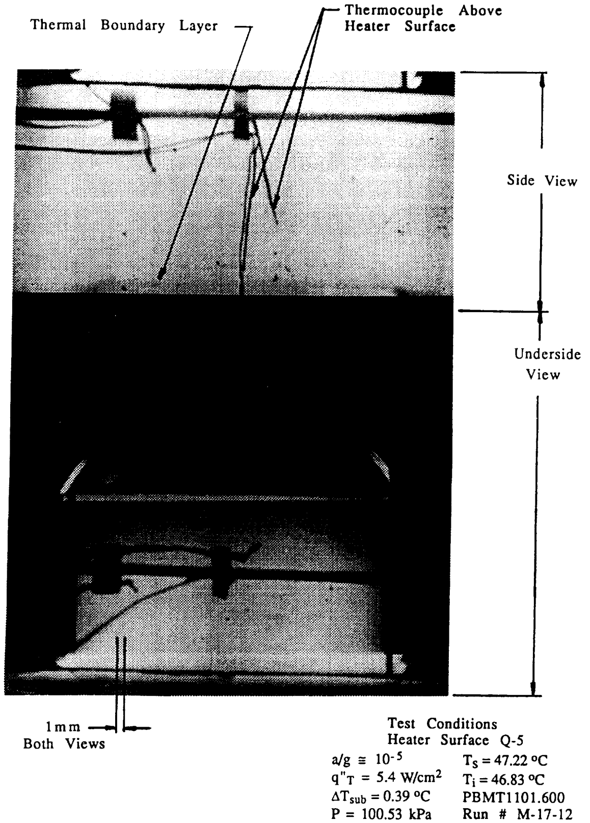
Figure 5.25a Category E: incipient boiling in the presence of the conduction thermal boundary layer, time = 1.130 sec
