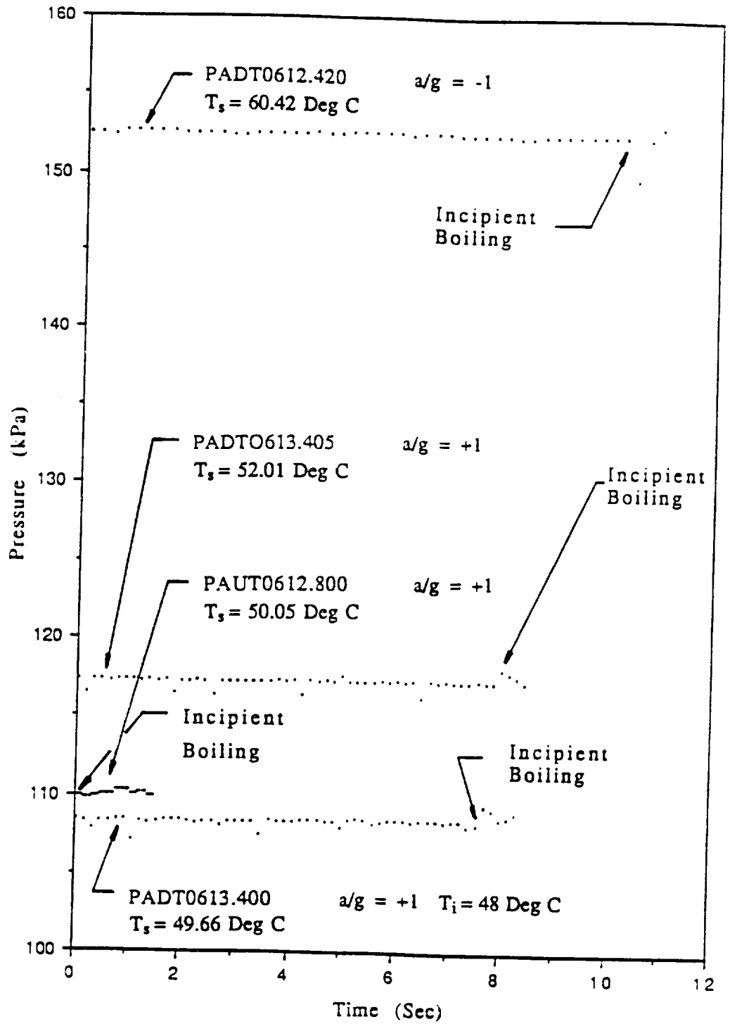
Figure 5.9 Representative pressure transducer measurements from the laboratory pool boiling vessel
