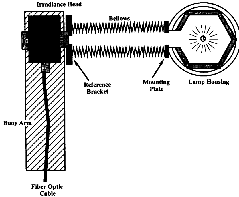
Fig. B-1. Irradiance measurements were performed by positioning the irradiance DUT at the reference bracket, with the reference surface of the DUT flush against the reference surface of the bracket.
