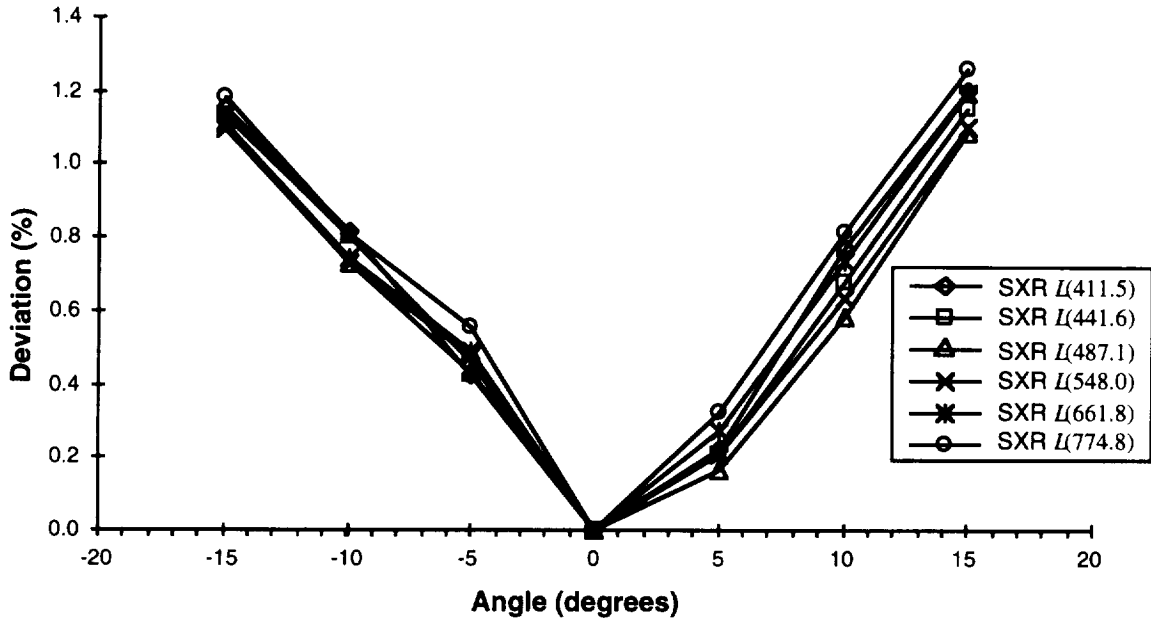
Fig. 30. Lambertian quality (angular uniformity of radiance) of the GSFC sphere, measured within 15° of the normal to the center of the plane of the exit aperture using the SXR. The quantity plotted is the spectral radiance at a particular viewing angle minus the spectral radiance at normal incidence, normalized to the normal incidence value, for the six measurement wavelengths of the SXR.
