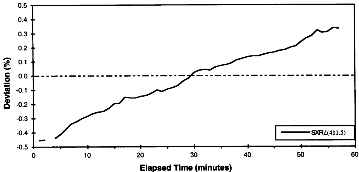
Fig. 25. Temporal stability of the spectral radiance of the BSI sphere as measured with the SXR on 26 Sept 1994, shown as the spectral radiance at 411.5 nm minus the average spectral radiance at this wavelength over the measurement interval, normalized to the average value.
