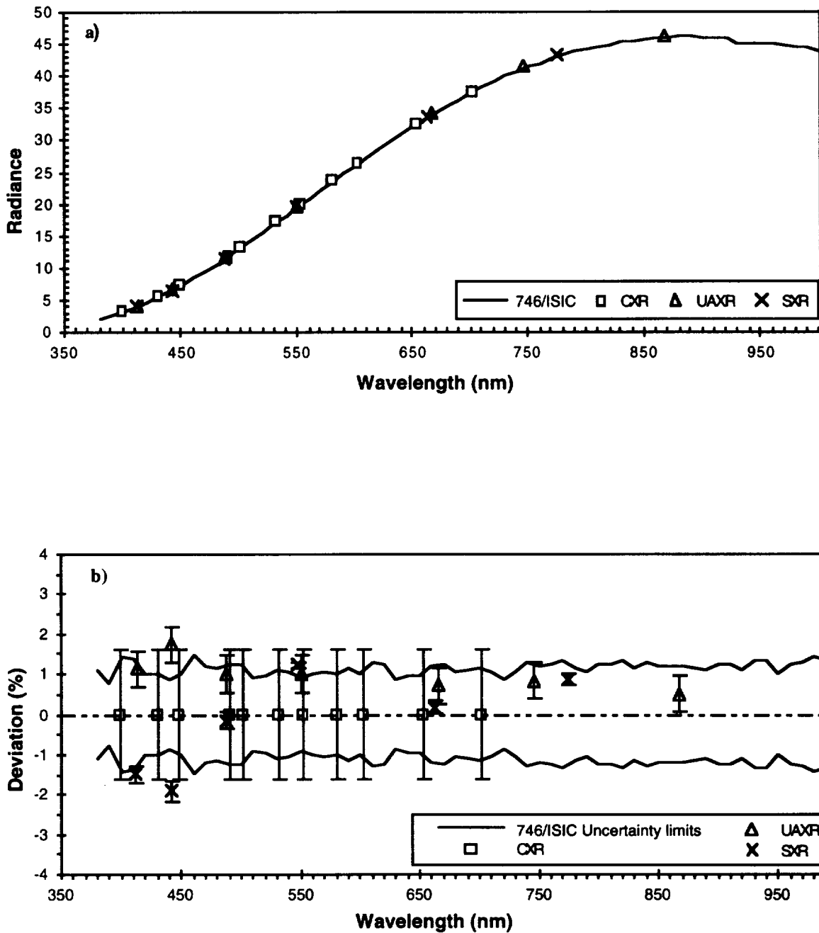
Fig. 16. a) Average spectral radiance in units of \mu\text{W}/(\text{cm}^2 \text{sr nm}) of the GSFC sphere (16 lamps) as measured with the 746/ISIC on three days using F268 or F269. The average spectral radiance of the two data sets using F268 on 29 Sept 1994 was used to calibrate the CXR and UAXR radiometers as explained in the text. b) Results from panel a with respect to the average of all of the 746/ISIC data for the GSFC sphere and the uncertainties, calculated using the standard deviation of the individual measurements. The quantity plotted using the symbol (see legend) is the average of the CXR, SXR, or UAXR data minus the average spectral radiance of the GSFC sphere as determined with the 746/ISIC, normalized to the average 746/ISIC values.
