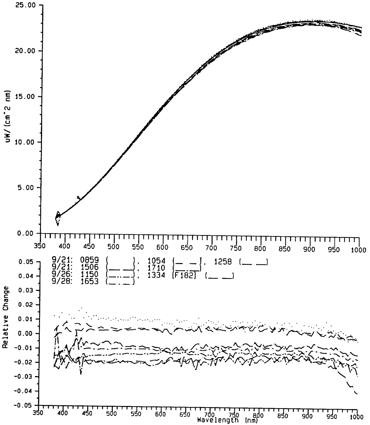
Fig. 5. The lower panel illustrates the relative changes with respect to the NIST October 1992 values for F269. The quantity plotted is the spectral irradiance for F269 which was determined at SIRREX-3 (using lamps F268 or F182) minus the NIST October 1992 values for F269, normalized to the NIST October 1992 values. The dates and times in the legends correspond to the measurements of F269 using the 746/ISIC. On 21 Sept 1994, the NIST August 1994 values of F268, transferred using other lamps at SIRREX-3 from the 28 Sept 1994 measurements, were used to determine the spectral irradiance of F269 (see text). On the other two days, the NIST August 1994 values of F268 (26 and 28 September) or F182 (26 September) were used as the reference lamp.
