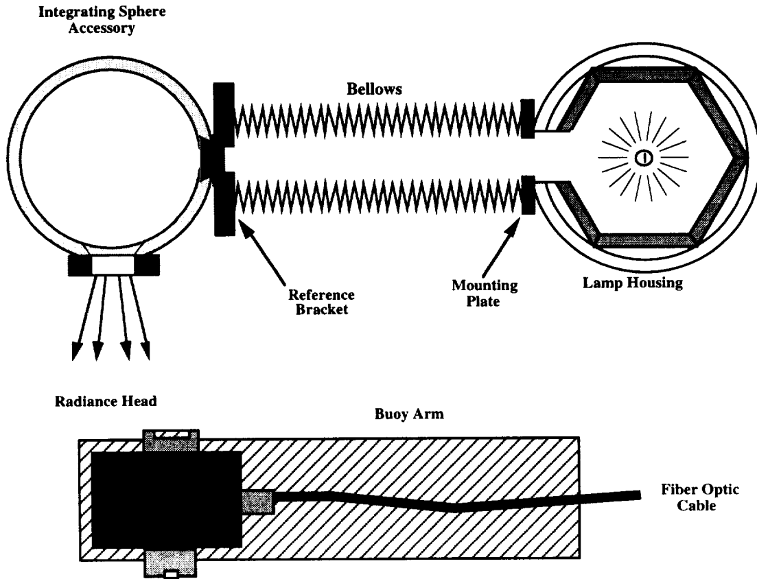
Fig. B-2. Radiance measurements were performed using the ISA. The entrance aperture of the ISA was aligned with the reference bracket, and the DUT was aligned to view the exit aperture of the ISA.
