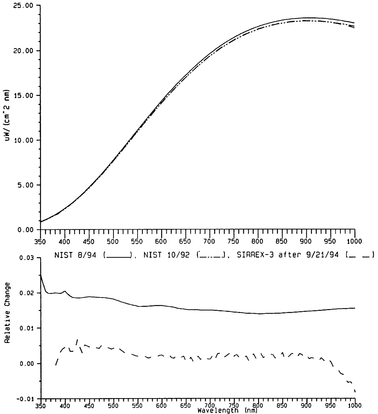
Fig. 1. NIST August 1994 calibration of the spectral irradiance (upper panel) of FEL lamp F269 (solid line) compared to the NIST October 1992 calibration, and to the new values derived using lamps F268 and F182, after the change in F269 between 12:58 and 15:06 PDT on 21 Sept 1994 (Fig. 2). The lower panel illustrates the relative changes with respect to the 1992 values. The quantity plotted using the solid line is the new measured value, or value being compared (NIST August 1994 data) minus the reference value (NIST October 1992 data), normalized to the NIST October 1992 data. The dashed line similarly shows the SIRREX-3 data compared to the NIST 1992 data.
