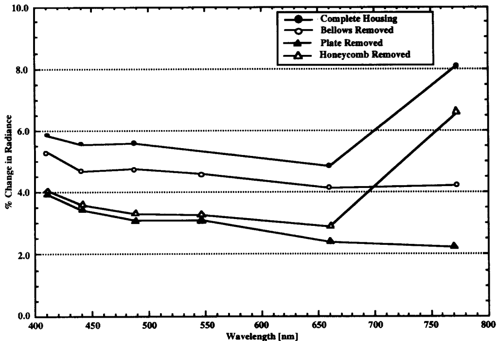
Fig. B-4. It was verified that scattered light was not entering the sphere by blocking the direct path from the lamp to the ISA. The results are shown in this figure.
