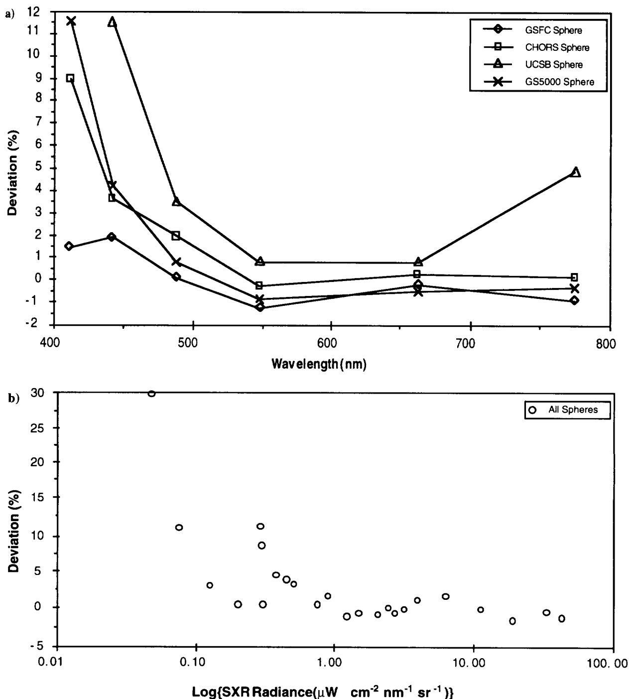
Fig. 32. a) Comparison of measurements of spectral radiance of the GSFC, CHORS, UCSB, and GS-5000 sphere sources using the 746/ISIC and the SXR. The quantity plotted for each sphere source (see legend) is the 746/ISIC result minus the SXR result, normalized to the SXR result. b) The same data as in panel a, except that the normalized deviations between the 746/ISIC and SXR measurements for these four sphere sources have been plotted as a function of the spectral radiance as measured by the SXR.
