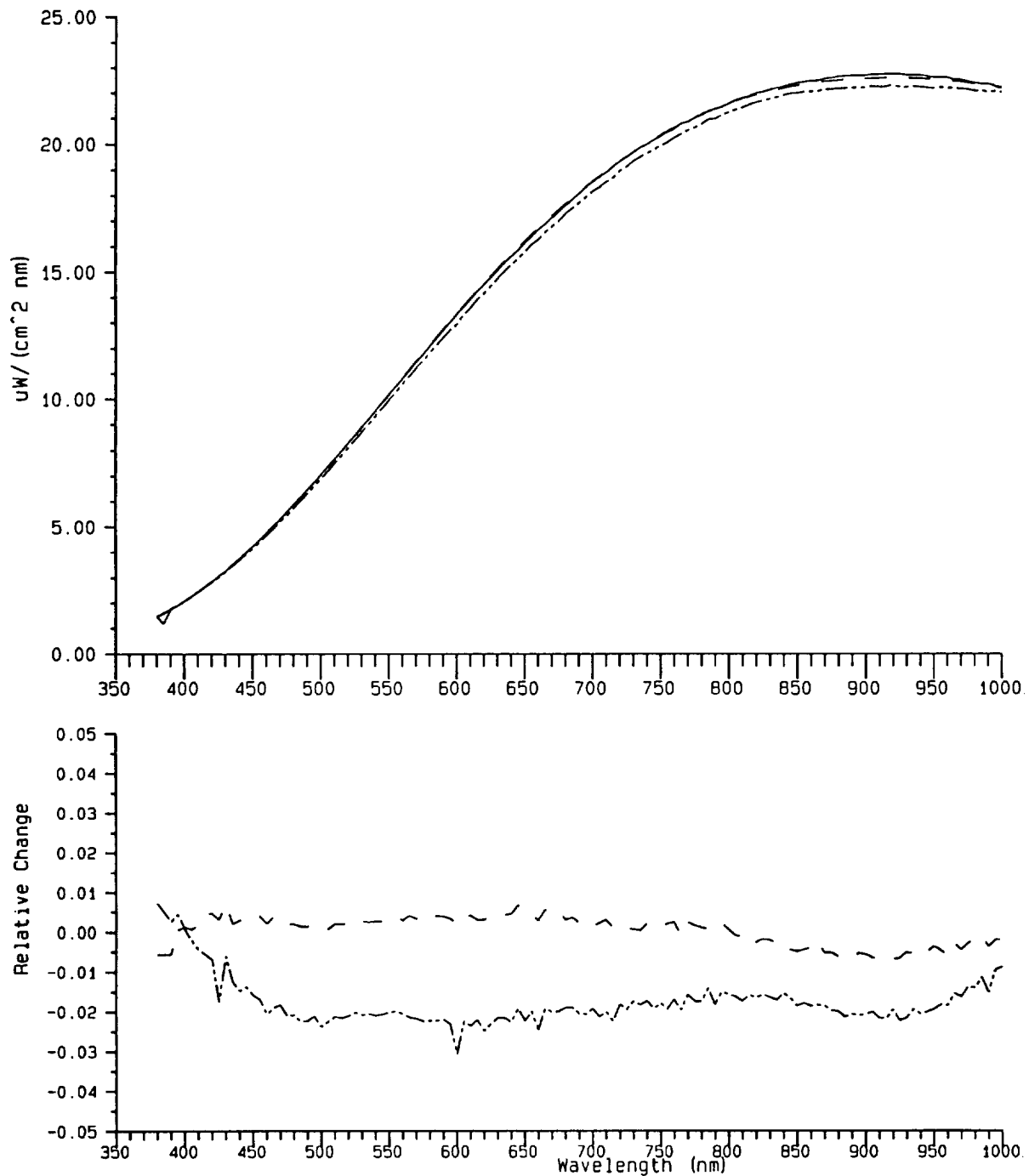
Fig. 10. Spectral irradiance of FEL lamp F123 determined by using F269 on 20 Sept 1994 (solid line), compared to the SIRREX-2 values (dash-dot-dot line) and the original calibration by OL in 1981 (dashed line). The spectral irradiance is plotted in the upper panel. The lower panel illustrates the relative changes with respect to the SIRREX-3 values. The quantity plotted using the dash-dot-dot line is the SIRREX-2 data minus the SIRREX-3 data, normalized to the SIRREX-3 data. The dashed line similarly shows the original calibration of F123 by OL in 1981.
