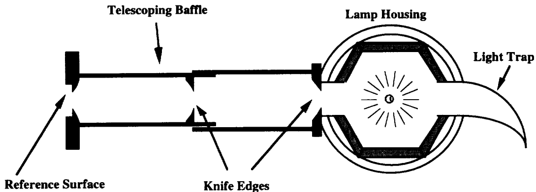
Fig. B-5. This figure shows specific improvements to be made to the baffling on the EG&G bench to assure accuracy during the irradiance calibrations.
