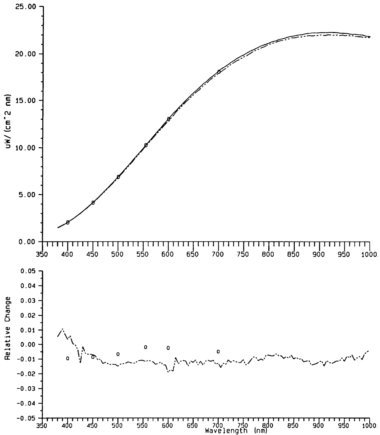
Fig. 8. Spectral irradiance of FEL lamp F321 determined using F269 on 20 Sept 1994 (solid line), compared to the SIRREX-2 values (dashed line) and the original calibration by NIST in February 1991 (o symbol). The spectral irradiance is plotted in the upper panel. The lower panel illustrates the relative changes with respect to the SIRREX-3 values. The quantity plotted using the dash-dot-dot line is the SIRREX-2 data minus the SIRREX-3 data, normalized to the SIRREX-3 data. The o symbol similarly shows the original calibration of F321 by NIST in February 1991.
