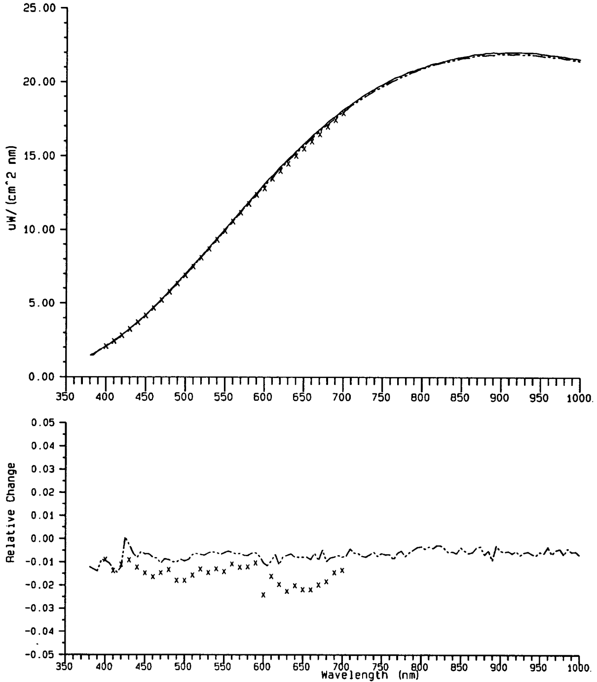
Fig. 11. Spectral irradiance of FEL lamp F12G determined using F269 on 20 Sept 1994 (solid line), compared to the SIRREX-2 values (dashed line) and the calibration by UM ( \times symbols). The spectral irradiance is plotted in the upper panel. The lower panel illustrates the relative changes with respect to the SIRREX-3 values. The quantity plotted using the dash-dot-dot line is the SIRREX-2 data minus the SIRREX-3 data, normalized to the SIRREX-3 data. The \times symbol similarly shows the calibration of F12G by UM.
