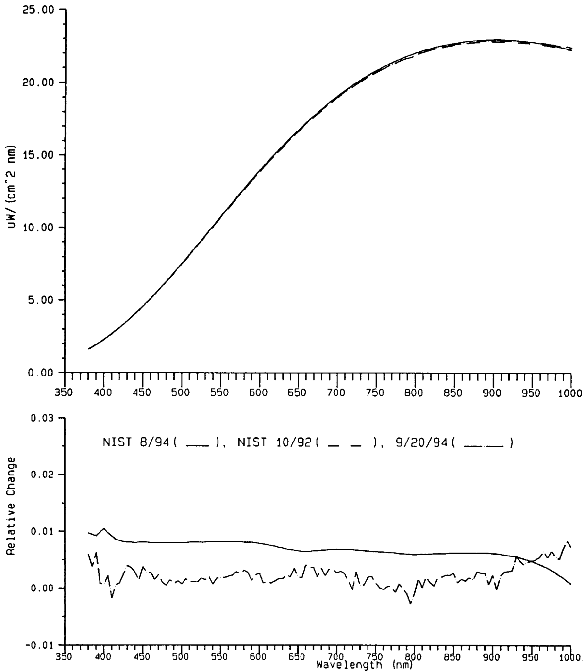
Fig. 2. Spectral irradiance of FEL lamp F268 measured using F269 (NIST August 1994 values) on 20 Sept 1994, compared with spectral irradiance values of F268 as calibrated by NIST in October 1992 and August 1994 (see legend above). The upper panel shows the spectral irradiance for F268 and the lower panel shows the changes with respect to the 1992 data. The quantity plotted is the new measured value (or value being compared from NIST August 1994) minus the reference value (NIST October 1992 data for F268), normalized to the NIST October 1992 data. The dash-dot-dash line shows the SIRREX-3 measurements for F268 compared to the NIST 1992 data.
