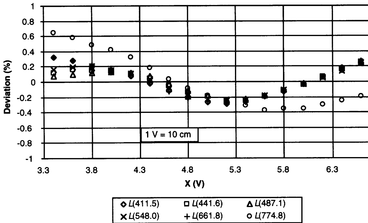
Fig. 26. Horizontal scans of the GSFC sphere radiance measured at all six wavelengths of the SXR on 9 Sept 1994, just prior to SIRREX-3 and after the GSFC sphere had been recoated. The SXR viewed a target area in the exit aperture of the sphere that was approximately 4 cm in diameter. The quantities plotted are the spectral radiance measured at a particular wavelength and horizontal position minus the average spectral radiance for all such measurements in the exit aperture of the sphere, normalized to this average value. The SXR was aligned to view the center of the exit aperture at the midpoint of the horizontal scan.
