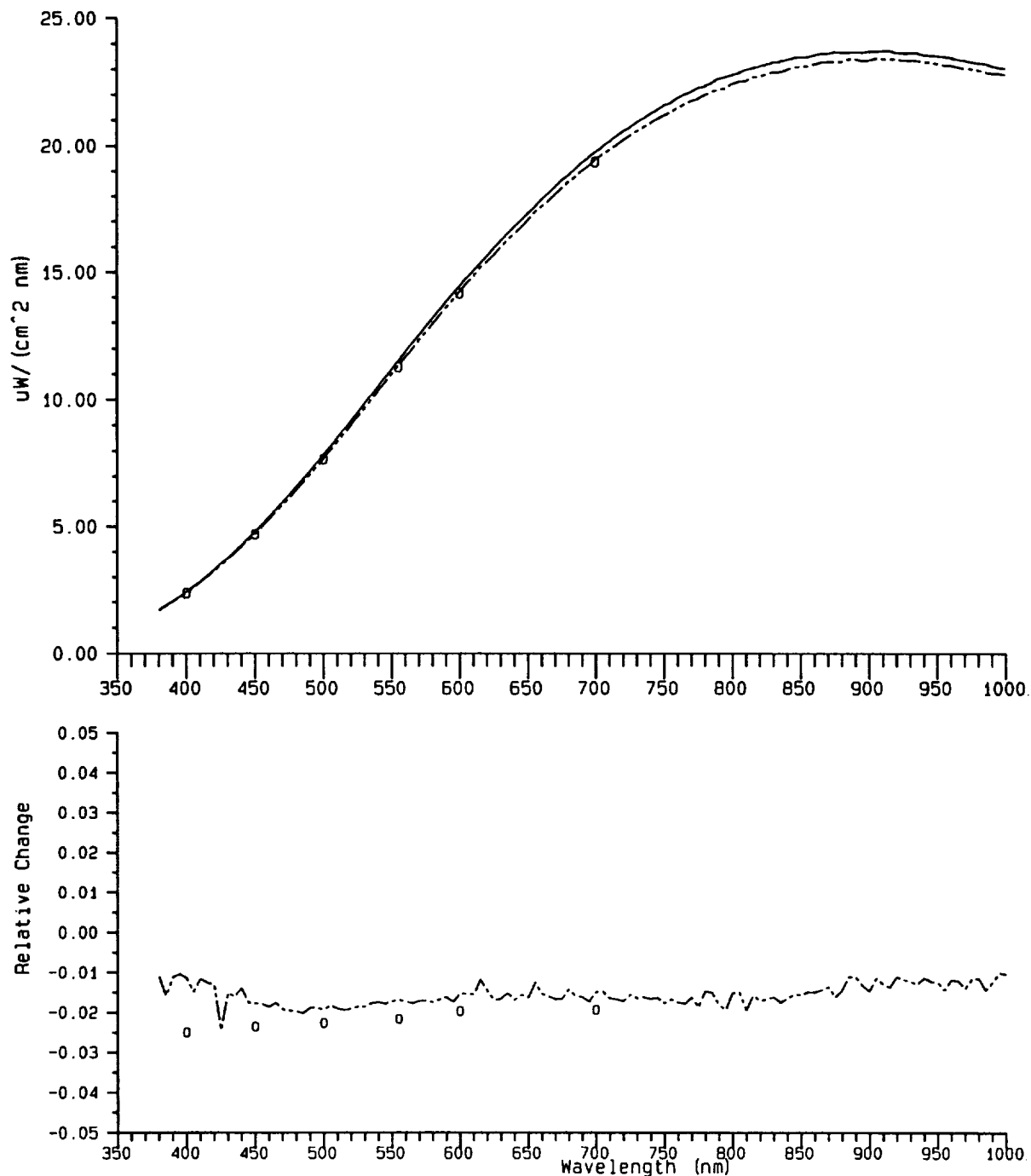
Fig. 9. Spectral irradiance of FEL lamp F308 determined using F268 on 28 September (solid line), compared to the SIRREX-2 values (dashed line) and the original calibration by NIST in October 1992 (o). The spectral irradiance is plotted in the upper panel. The lower panel illustrates the relative changes with respect to the SIRREX-3 values. The quantity plotted using the dash-dot-dot line is the SIRREX-2 data minus the SIRREX-3 data, normalized to the SIRREX-3 data. The o symbol similarly shows the calibration of F308 by NIST in October 1992.
