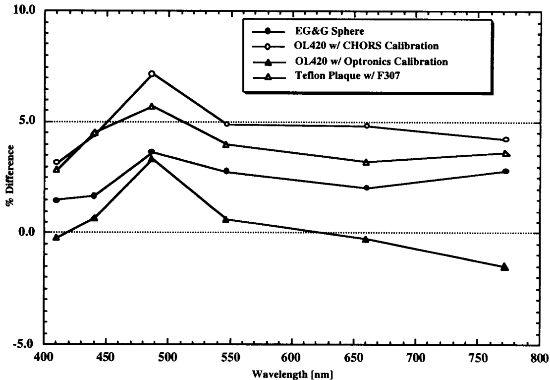
Fig. B-3. This figure shows the plot of the percent deviation of the SXR measurement from the presumed radiance of the sources at the six SXR channel wavelengths.
