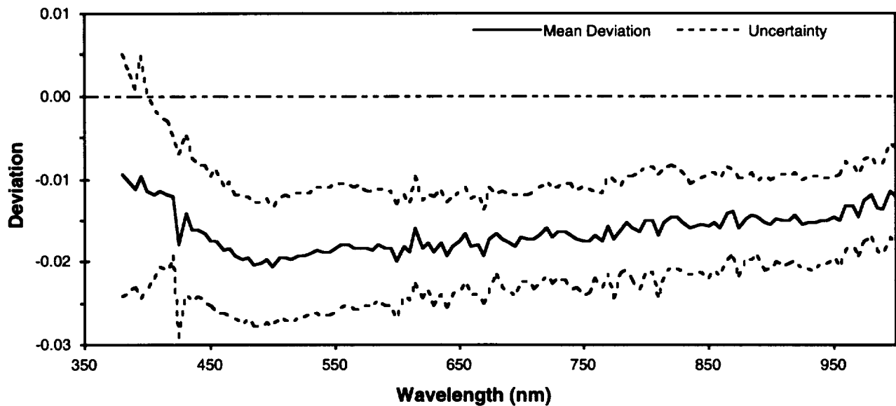
Fig. 15. The average change in the lamp irradiances measured at SIRREX-3 relative to those measured at SIRREX-2 for the six lamps (F321, F308, F123, F12G, F303, and F307) that were studied in both experiments. The quantity plotted using the solid line is the average of the relative changes, or deviations (i.e., the SIRREX-2 data minus the SIRREX-3 data) normalized to the SIRREX-3 data (see the lower panels of Figs. 8–13). The quantity plotted using the dashed line is the average deviation plus or minus the standard deviation of the relative changes for the six lamps.
