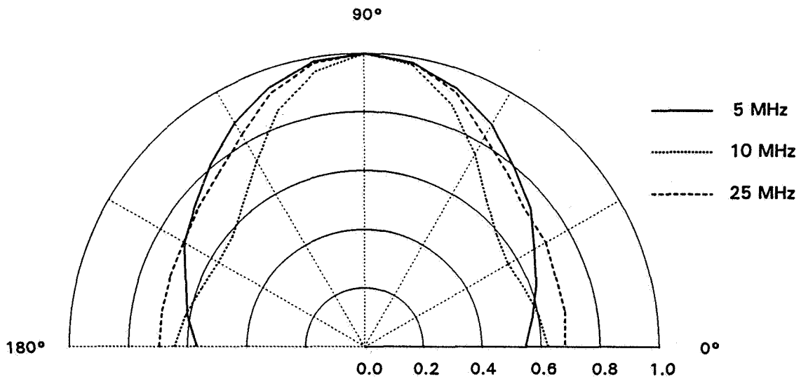
b) Radiation Patterns for Higher Frequencies.
