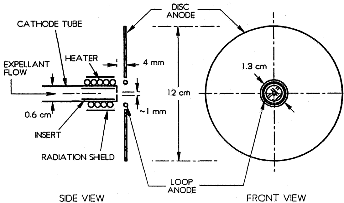
a) Hollow-Cathode Plasma Contactor Schematic.
