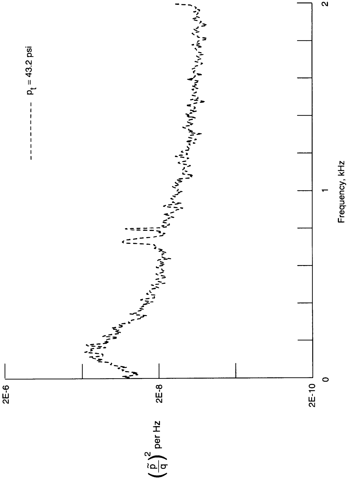
(c) M = 0.6 .
