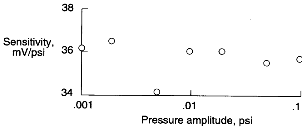
(b) Dynamic range at 1 kHz.
