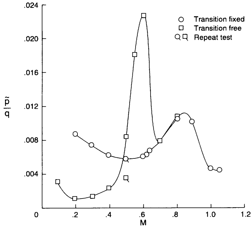
(a) p_1 = 15 psi; ambient temperature; minimum Reynolds number boundary; air mode.
