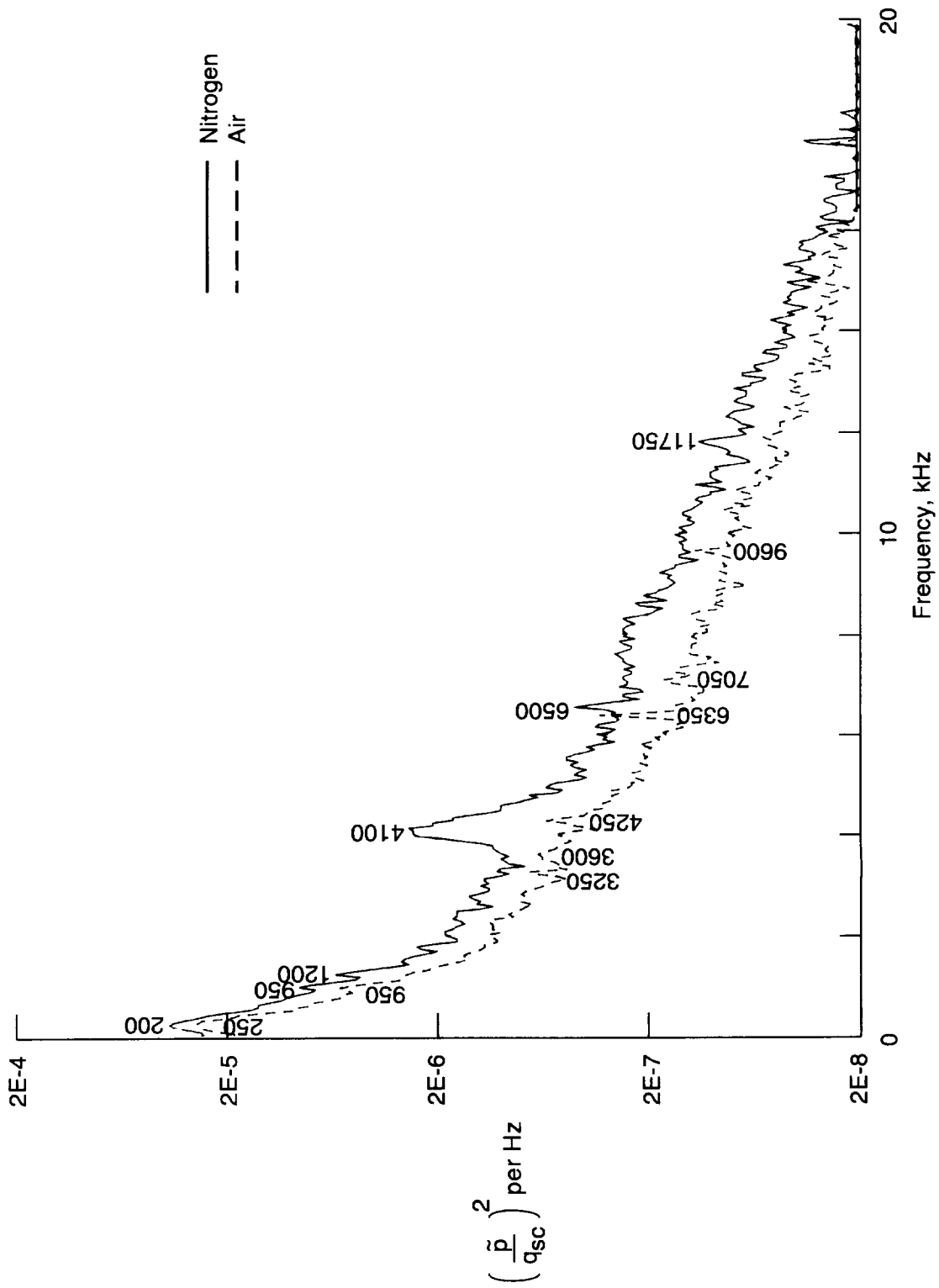
(e) M = 0.75 .
