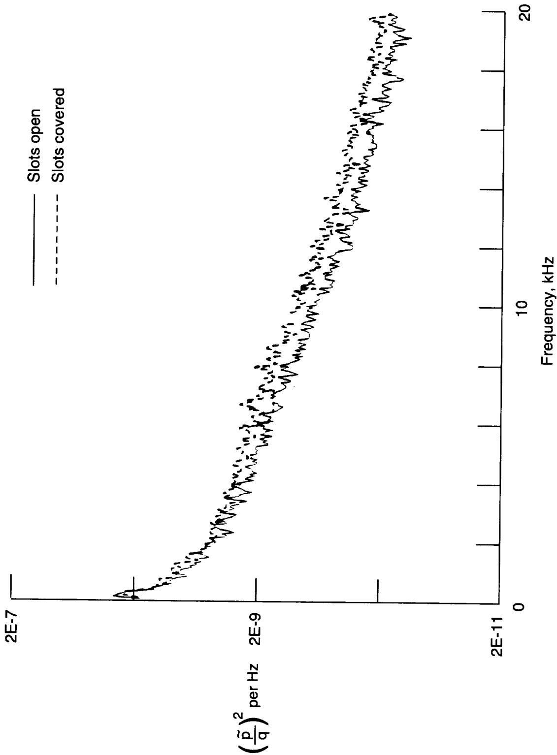
(a) M = 0.2 .
