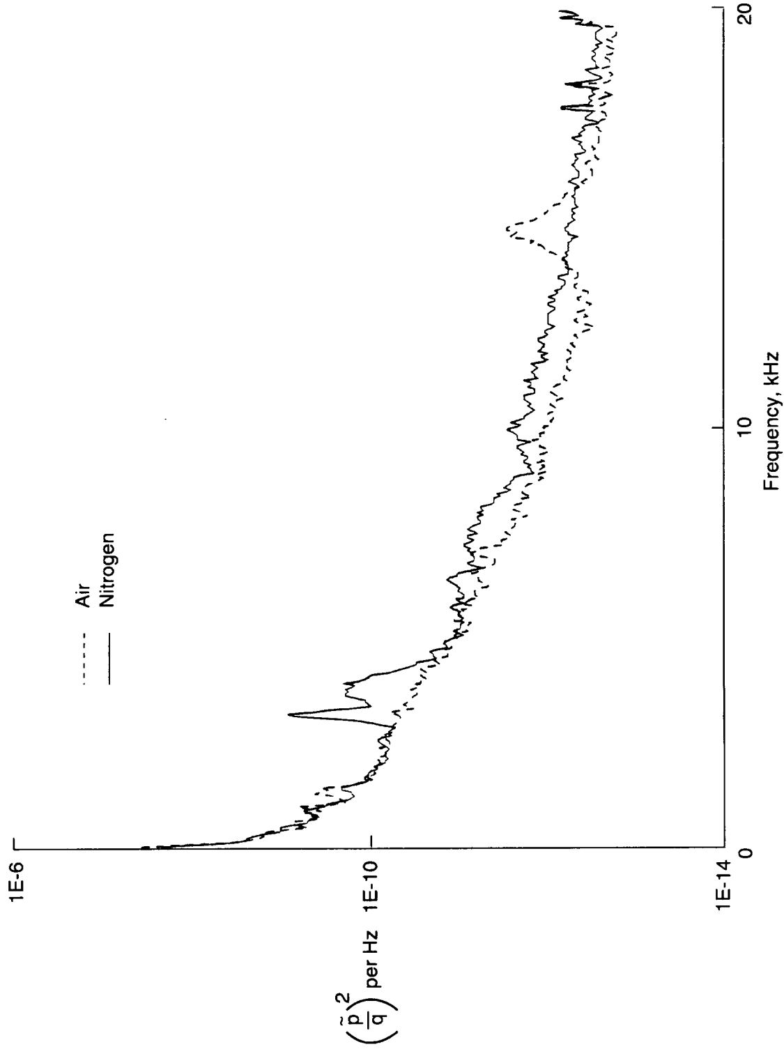
(a) M = 0.2 .
