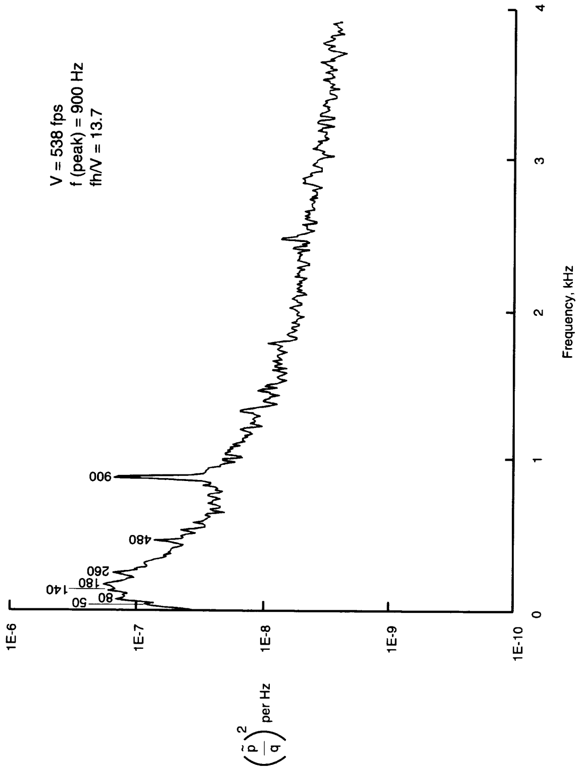
(c) M = 0.742 .
