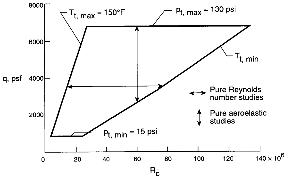
Figure 3. Operating envelope at constant Mach number. M = 1.0 ; \bar{c} = 0.82 \text{ ft} .
