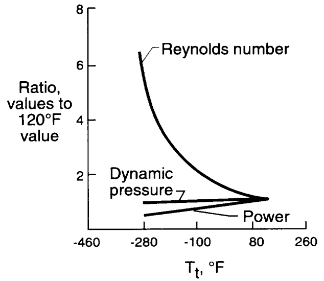
(b) Test conditions and fan drive power.
