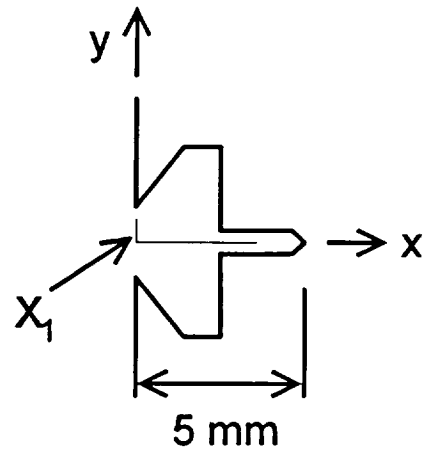
(b) Displacement-Gage Notch ( W = 38\text{ mm} ).
