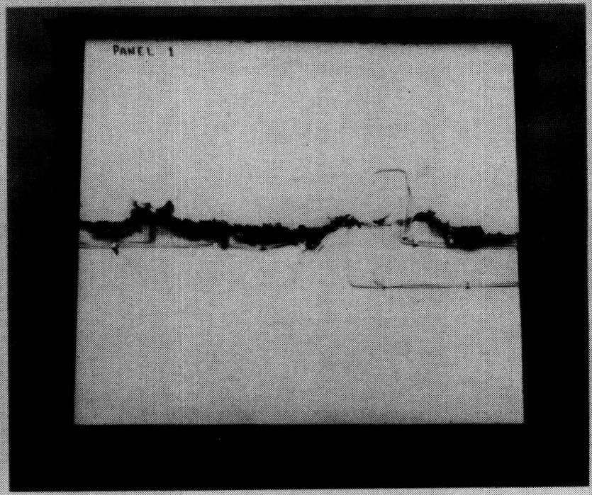
Skin side
