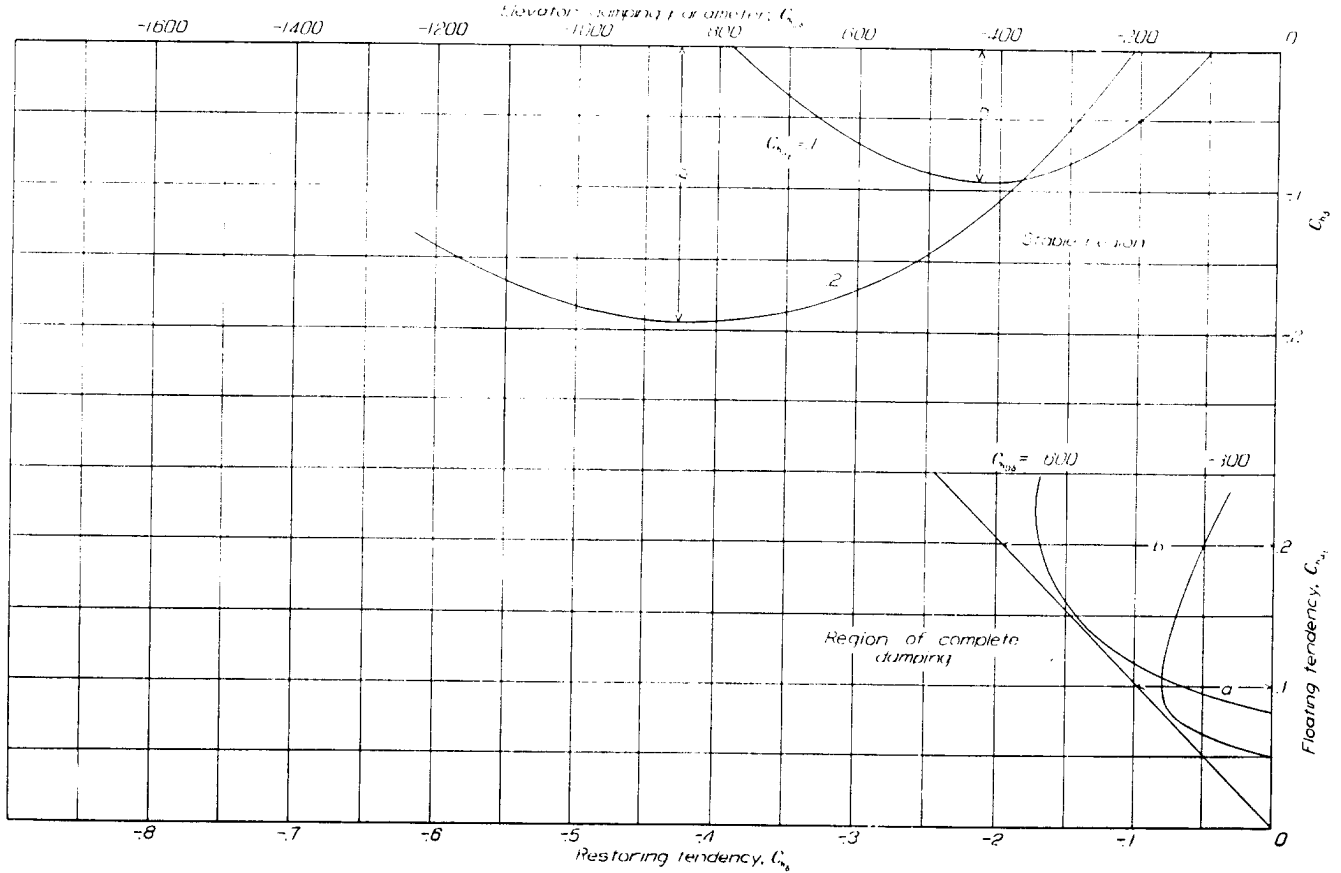
FIGURE 17.—Method of constructing boundary for complete damping.
