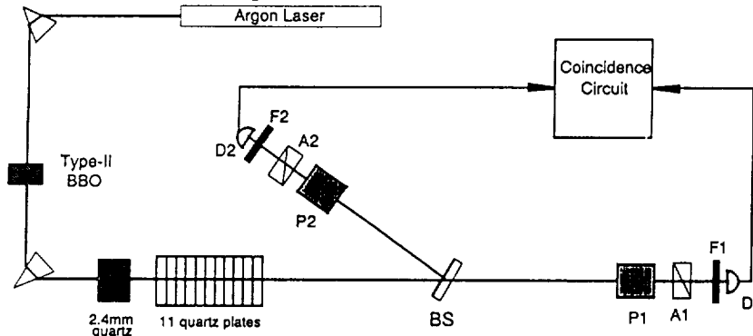
Figure 3. Schematic set up for the new type two-photon interferometer.
