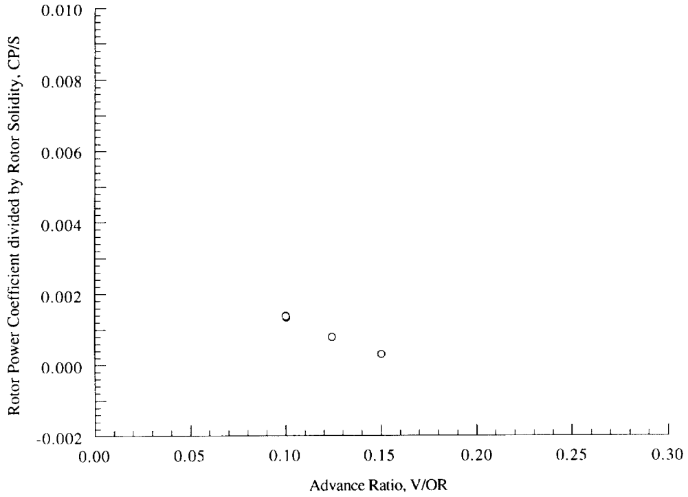
Figure 20(a). Rotor power coefficient as a function of advance ratio, \alpha_S = 10 deg, C_T/\sigma = 0.070 .
