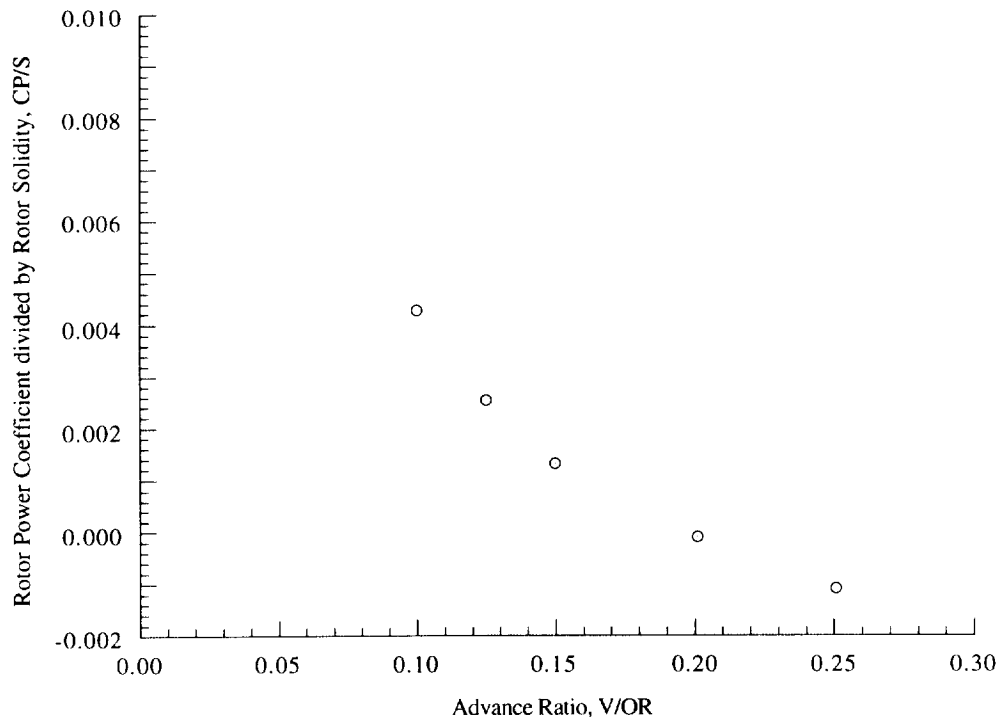
Figure 20(f). Rotor power coefficient as a function of advance ratio, \alpha_S = 10 deg, C_T/\sigma = 0.120 .
