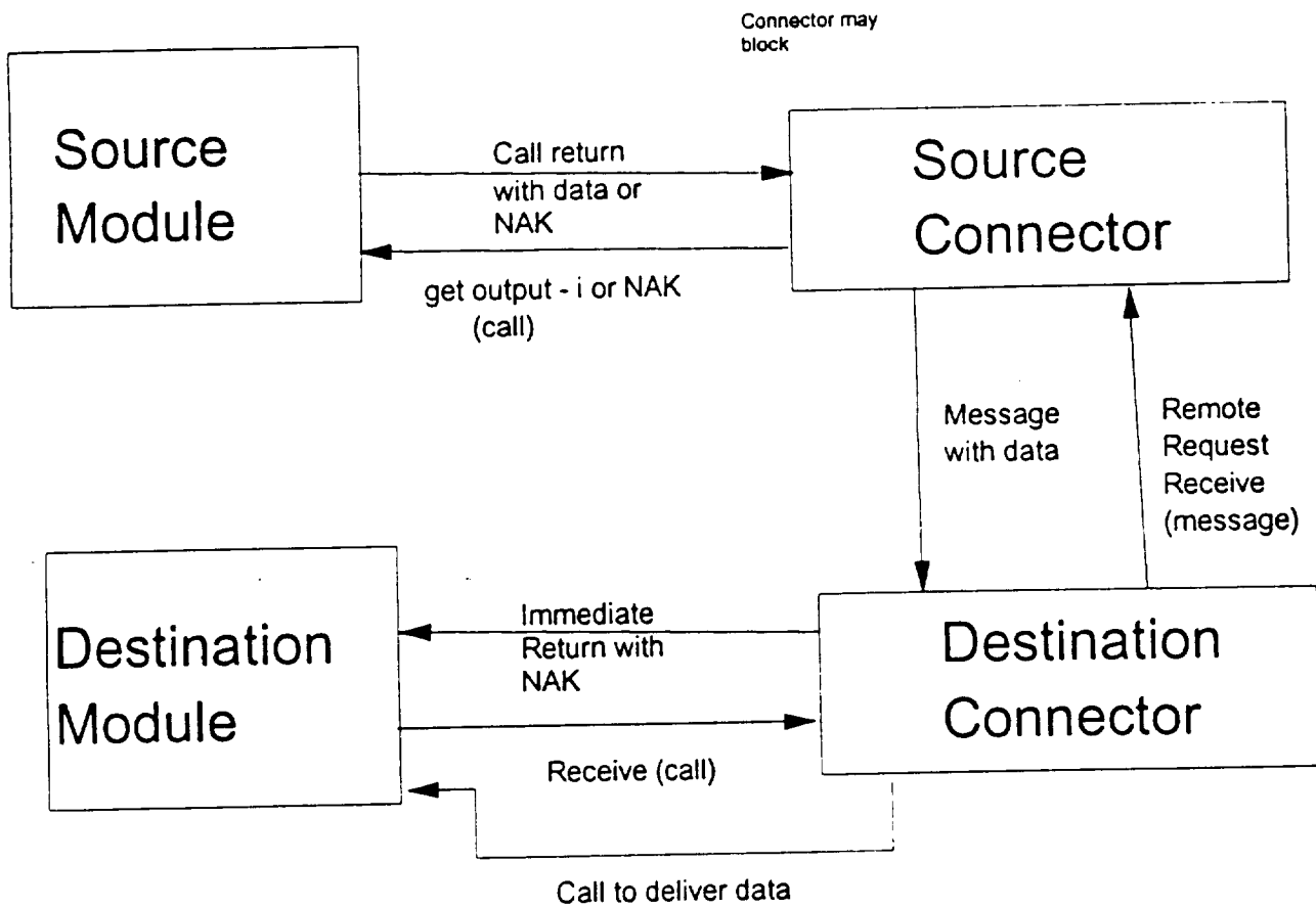
Figure 3.3 Inter-Module Communication Modules in separate processes
