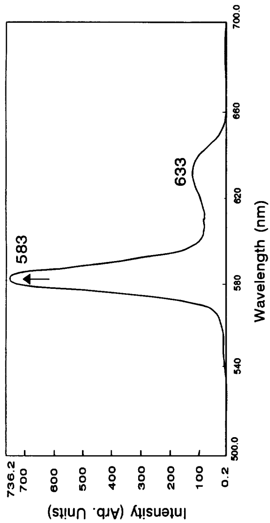
Figure-4. Emission Spectrum from Mg.OEP molecules dissolved in \text{CH}_2\text{Cl}_2 , excited at 4010 \text{ \AA} .
