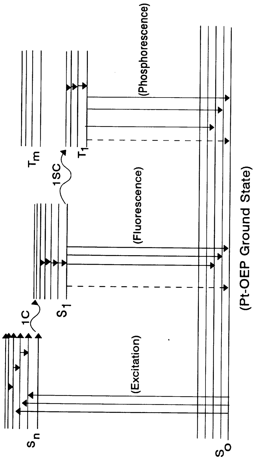
Figure -1 (b). Typical level Scheme for a metalloporphyrin molecule.
