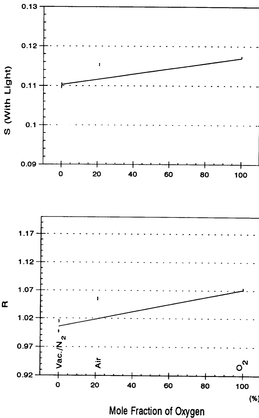
Figure-6 (b). Variation of Doppler Broadening Parameters in (Pt.OEP) Molecules as a Function of Mole Fraction of Oxygen.
