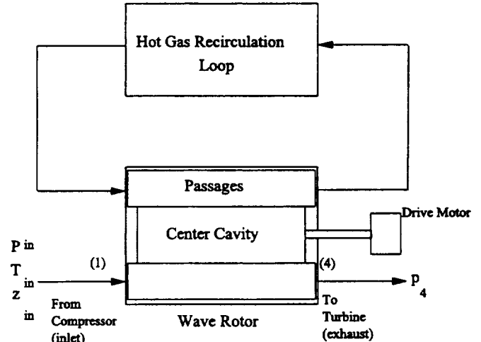
Figure 2 System Layout
