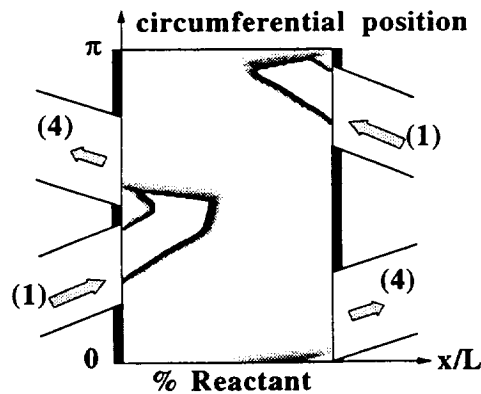
Figure 7 Reverse-Flow Detonation-Mode Cycle
