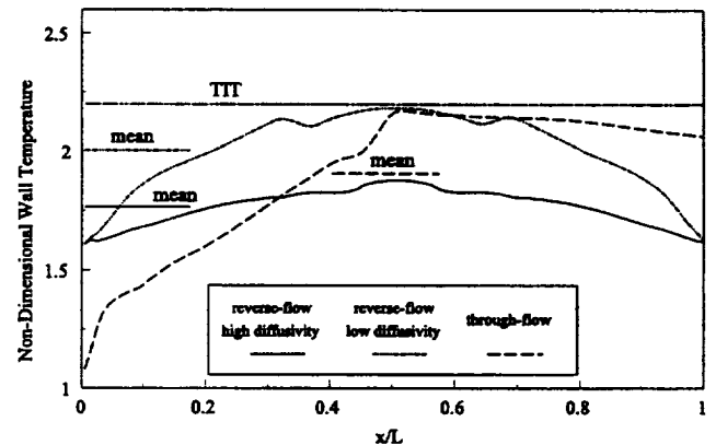
Figure 9 Detonation Mode Wall Temperatures
