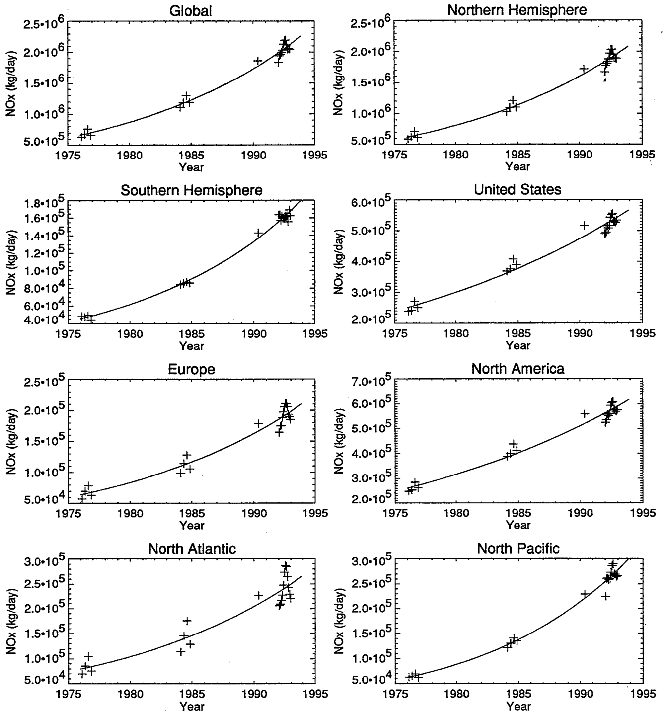
Figure 4-5. Calculated NOx emissions as a function of year for the time period 1976-1992 in the 9-13 kilometer altitude band. The solid line is the fit to an exponential growth curve.
