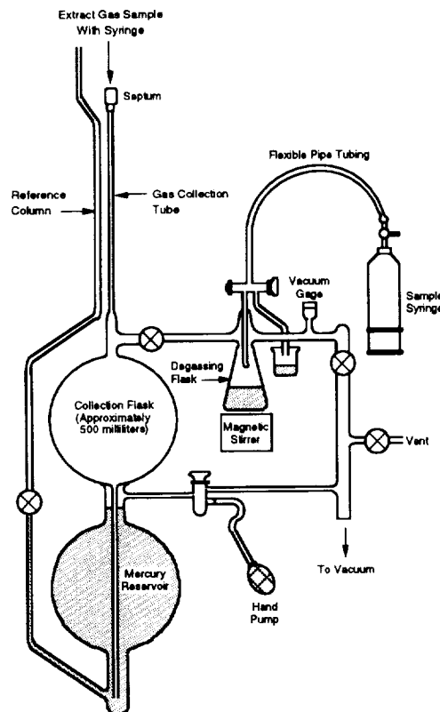
ASTM Procedure Apparatus
