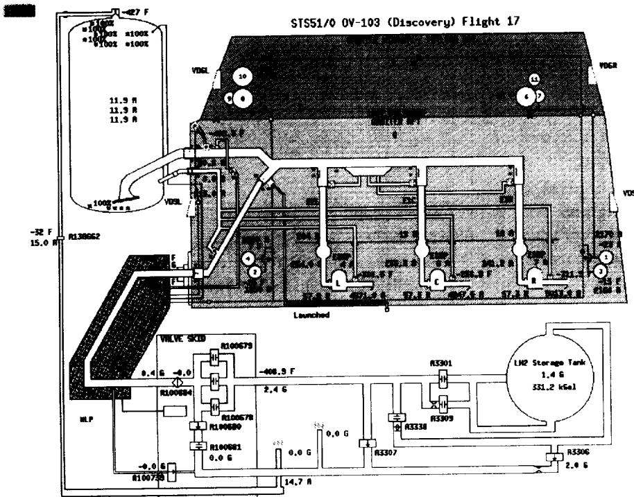
Liquid Hydrogen Screen
