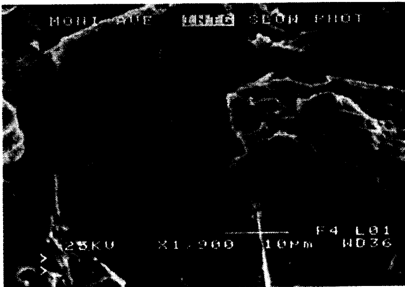
Scanning Electron Micrograph of the Fracture Surface (Magnification: 1,900X)
