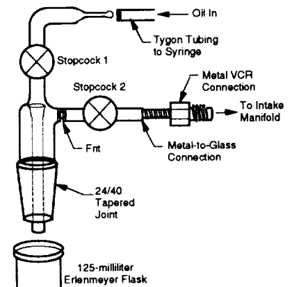
New Analysis System (New Outlet Apparatus)
