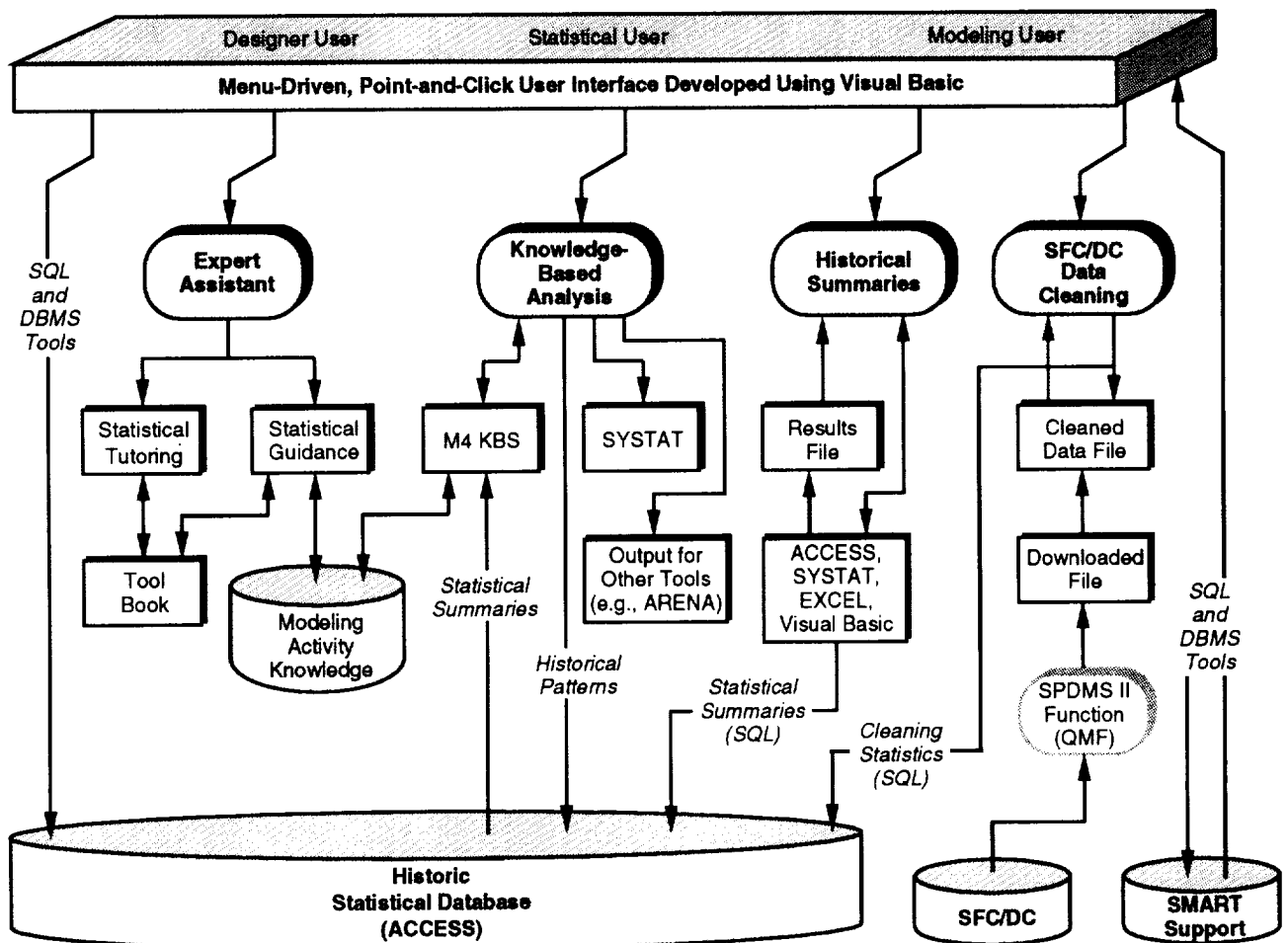
SMART Framework
