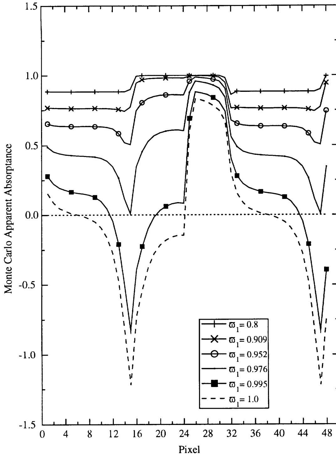
Figure 3.29 Apparent absorbance for N_c = 50\% and a = 0.25 geometric values, and conservative droplet scattering for different vapor absorptance values.
