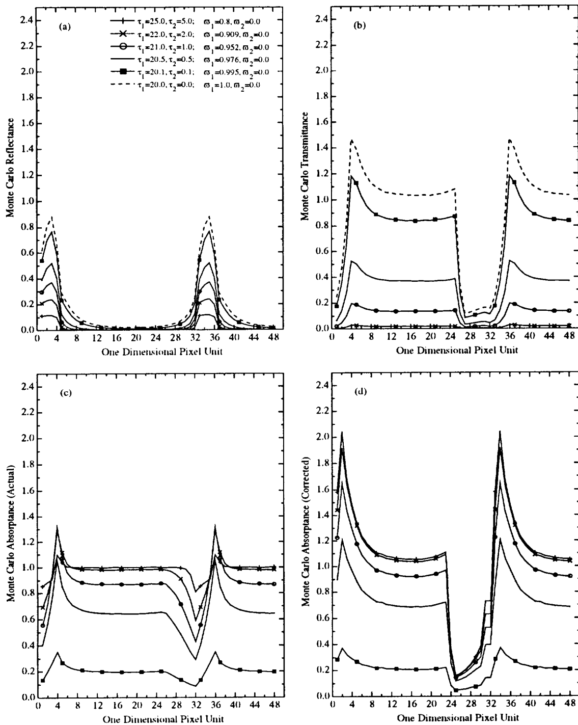
Figure 3.7 Same as Figure 3.5 except for a cloud fraction of 12.5% and aspect ratio of 1.0.
