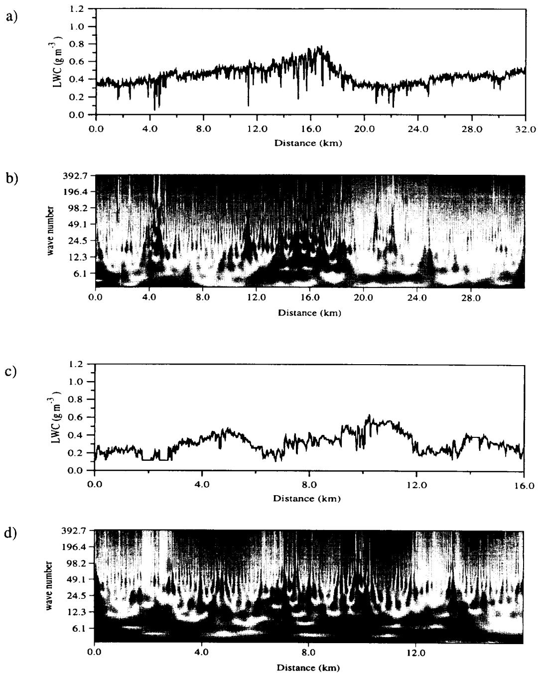
Figure 6.5 Time series data samples and modulus scalograms where wave number is in units of \text{km}^{-1} , and darker areas correspond to higher magnitudes and lighter areas correspond to lower magnitudes in the scalograms. For time series from (a) June 2, 1992 and (c) June 8, 1992 along with their modulus scalograms (b) and (d) respectively.
