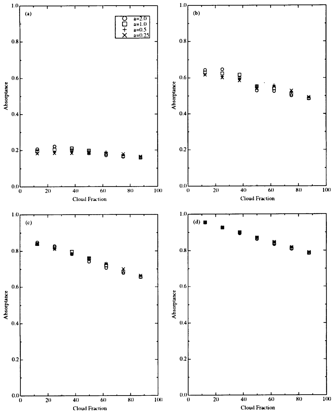
Figure 3.45 System absorbance for conservative droplet scattering for different vapor absorption, which yields \bar{\omega} of (a) 0.995, (b) 0.976, (c) 0.952, and (d) 0.909 in the cloudy portion.
