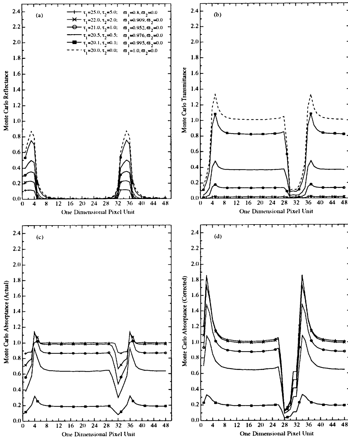
Figure 3.6 Same as Figure 3.5 except for a cloud fraction of 12.5% and aspect ratio of 0.5.
