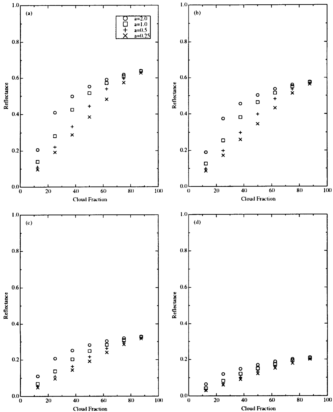
Figure 3.48 System reflectance for zero vapor absorption and \bar{\omega} of (a) 0.995, (b) 0.99, (c) 0.95, and (d) 0.9 in the cloudy portion.
