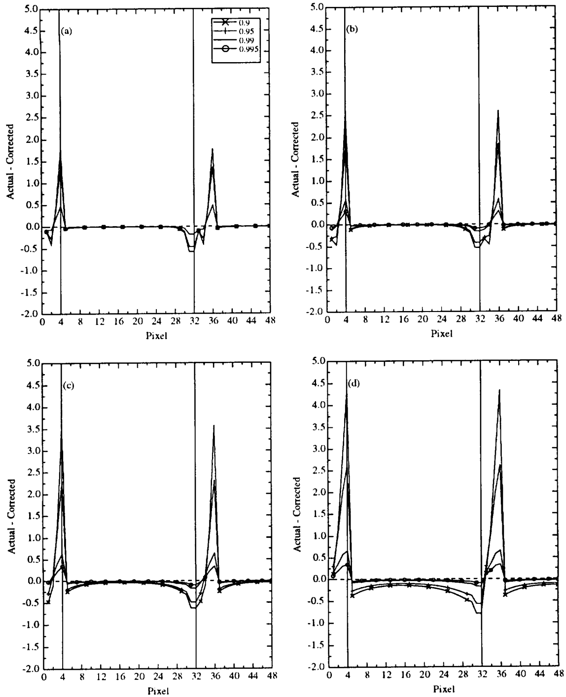
Figure 3.38 Difference between the Monte Carlo Absorbance (actual) and the Corrected Absorption by the Ackerman and Cox method for the second study. For a 12.5% cloud fraction and aspect ratio of (a) 0.25, (b) 0.5, (c) 1.0, and (d) 2.0.
