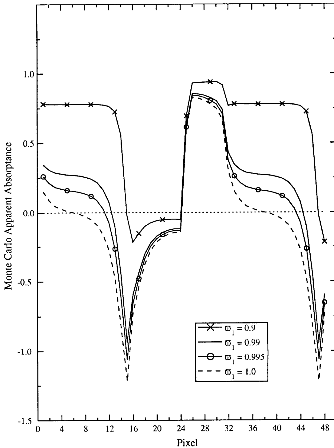
Figure 3.30 Apparent absorptance for N_C = 50\% and a = 0.25 geometric values, and zero vapor absorption values.
