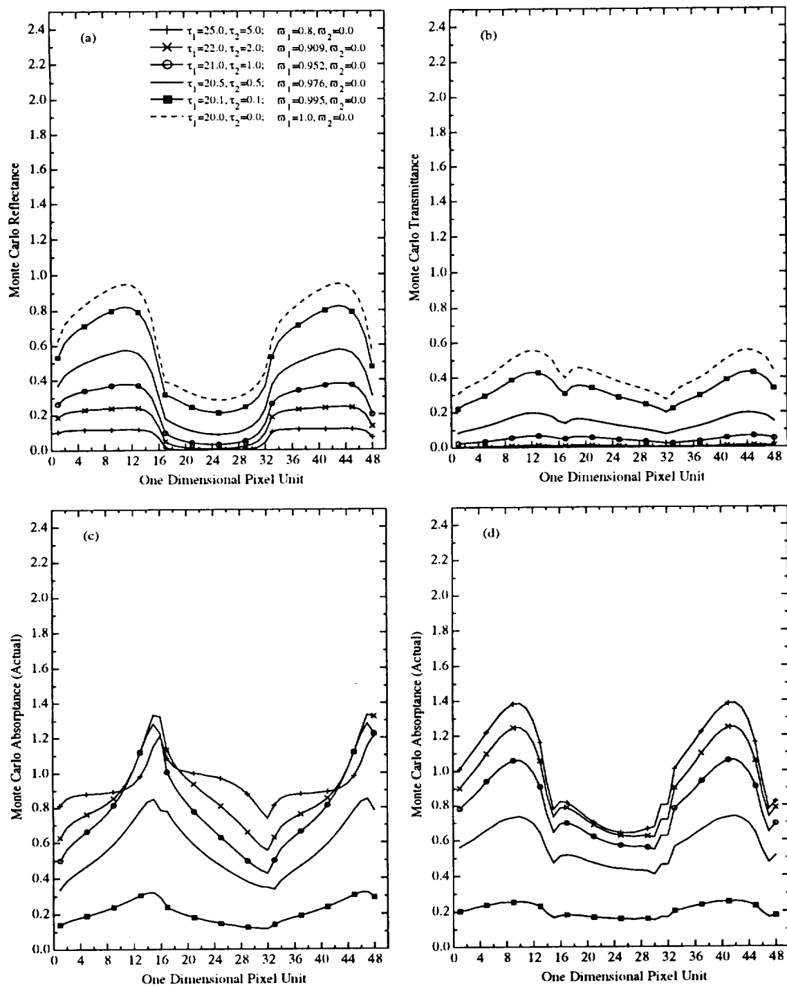
Figure 3.11 Same as Figure 3.5 except for a cloud fraction of 50% and aspect ratio of 1.0.
