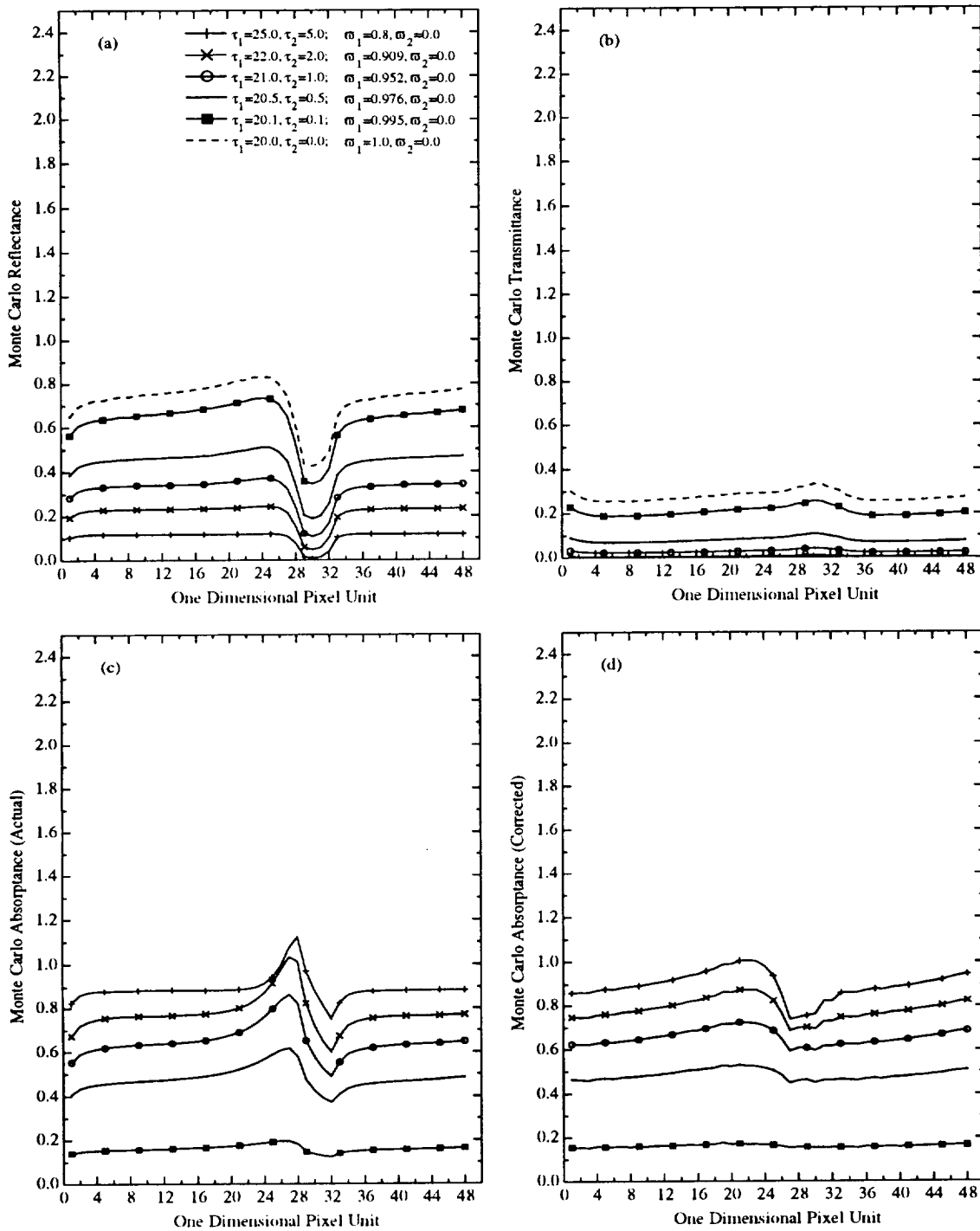
Figure 3.14 Same as Figure 3.5 except for a cloud fraction of 87.5% and aspect ratio of 0.5.
