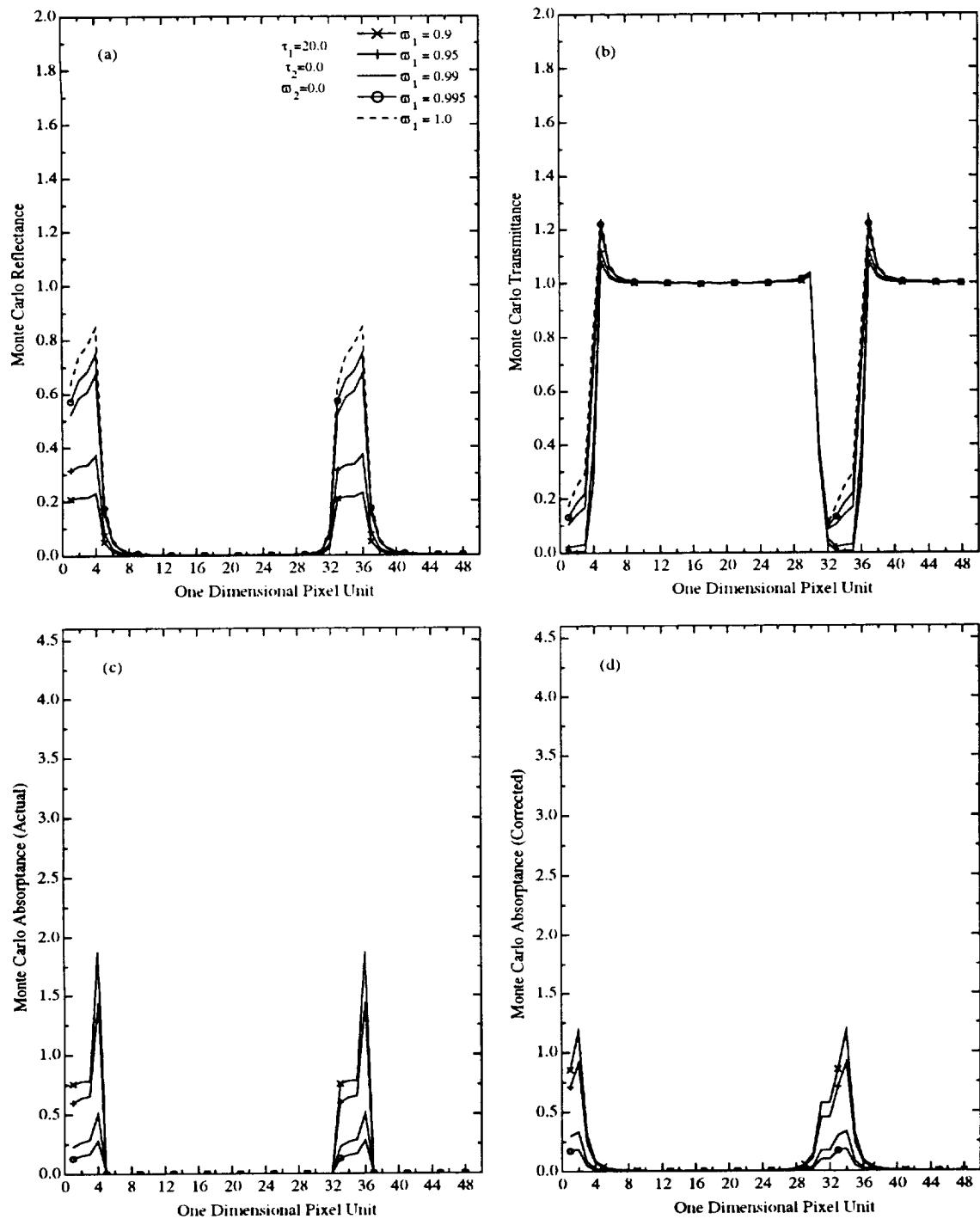
Figure 3.17 Monte Carlo (a) reflectance, (b) transmittance, (c) absorptance, and (d) corrected absorptance for the second study with a cloud fraction of 12.5% and aspect ratio of 0.25.
