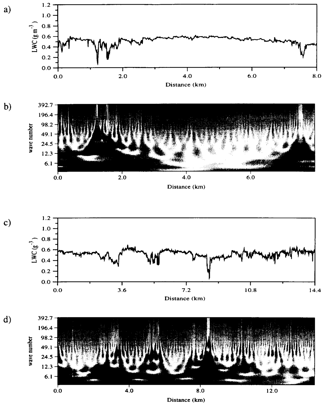
Figure 6.6 Same as Figure 6.5 except for time series from (a) June 13, 1992 and (c) June 17, 1992 along with their modulus scalograms (b) and (d) respectively.
