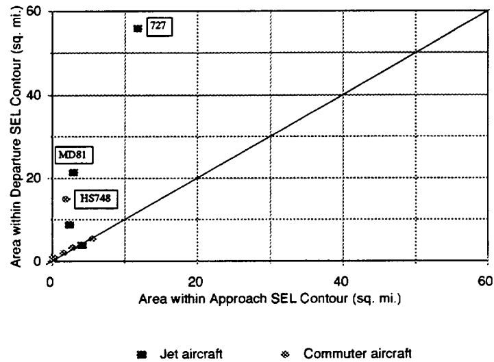
Figure 8 Comparison of land area within 75 dB L ≤ SEL ≤ 80 dB noise contour on departure and approach for 10 aircraft.
