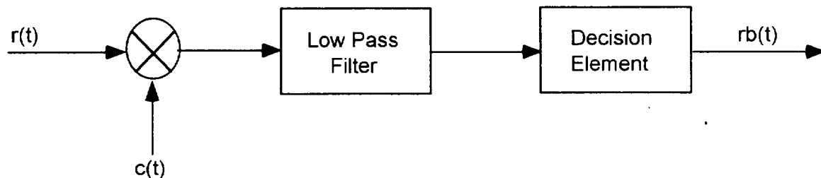
Figure 3.4 DAMA Demodulator
