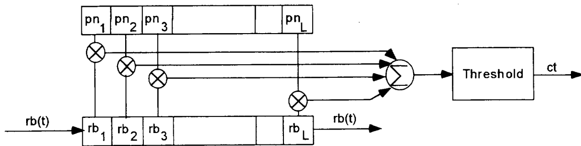
Figure 5.1 PN Acquisition
