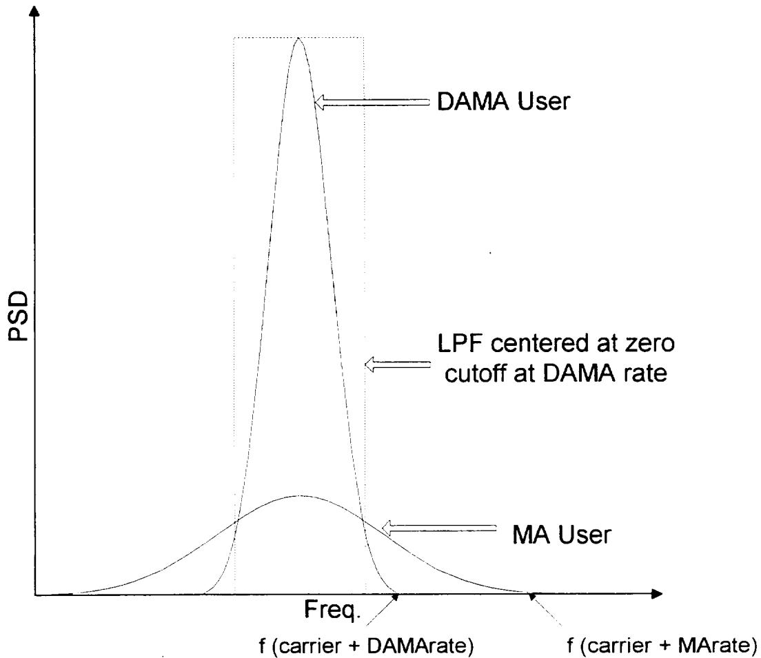
Figure 4.5 (MA = 4* DAMA chip rate)
