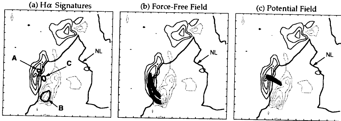
Figure 10. (a) H \alpha flare features superimposed on the magnetogram of AR5747 (adapted from Leka et al. 1993). The dark line marked NL denotes the magnetic neutral line; the contours denote the vertical current. The three small pseudo-circular features enclose areas in which specific H \alpha signatures were detected. The features marked A and B show sites which were identified as high pressure “footpoints,” whereas C was identified as an electron-precipitation site and coincided temporally with hard-X-ray emission. (b) Field-line traces in the estimated force-free coronal field, showing that the high-pressure sites A and B are close to the footpoints of a coronal loop. (c) Field-line traces in the potential coronal field, with the same initial footpoint positions (at A) as in (b), showing that the agreement between the high-pressure sites and coronal-loop footpoints is much better for the estimated force-free field than for a crude current-free field.
