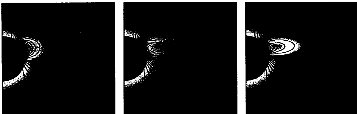
Figure 2. Disruption of an axisymmetric helmet streamer by differential solar rotation. Projected magnetic field lines (shown in black) have been overlaid on the simulated polarization brightness (large values in white, small values blue).
