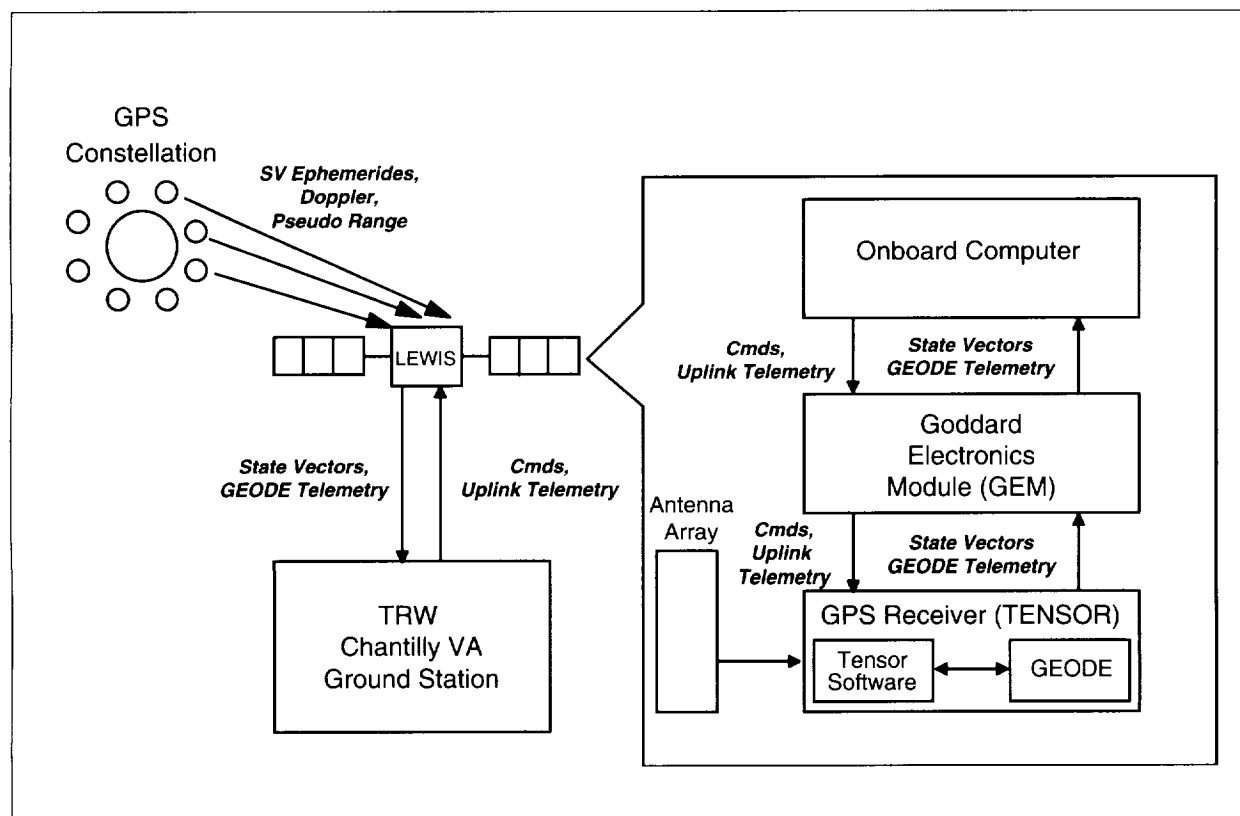
SSTI/Lewis configuration showing Tensor and embedded GEODE software.
