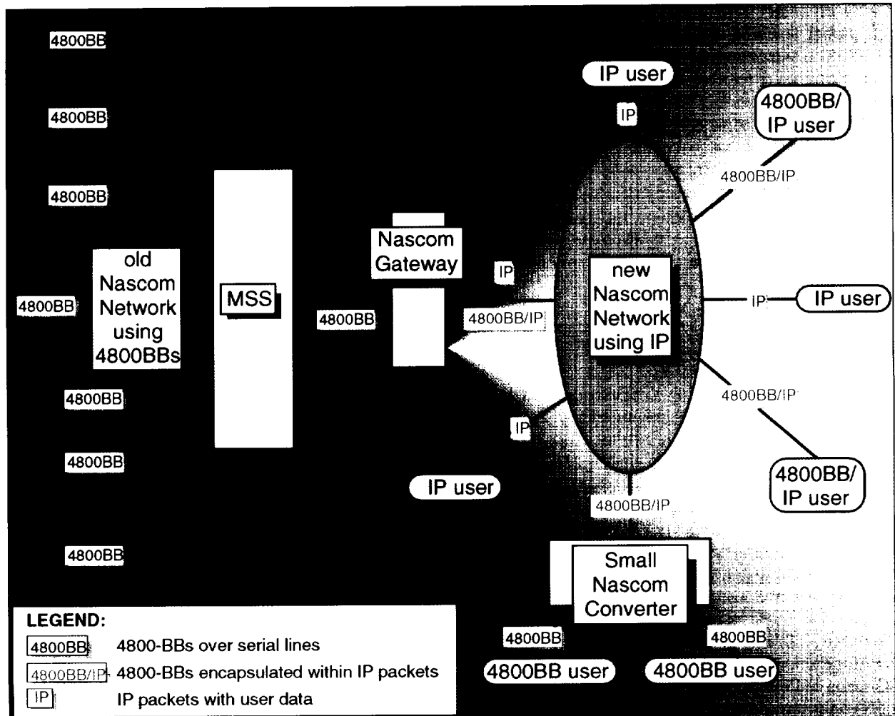
NASCOM IP transition.
