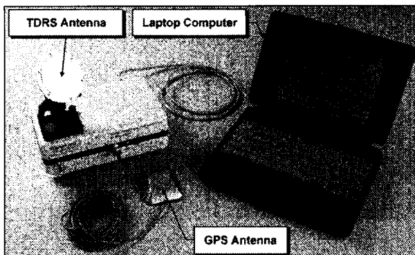
Portable transmitter.
