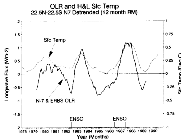
Mean tropical ( 22.5^{\circ}\text{N} to 22.5^{\circ}\text{S} latitude) interannual (12-month running mean) surface air temperature and OLR anomalies for the period from 1979 to 1989. The temperature curve shows deviations from the 1951 to 1980 average as derived by Hansen and Lebedeff (H&L) and coworkers at the Goddard Institute for Space Studies. The OLR curve was obtained by combining measurements from the Nimbus-7 and the Earth Radiation Budget Satellite, and the anomalies are departures from the mean.
