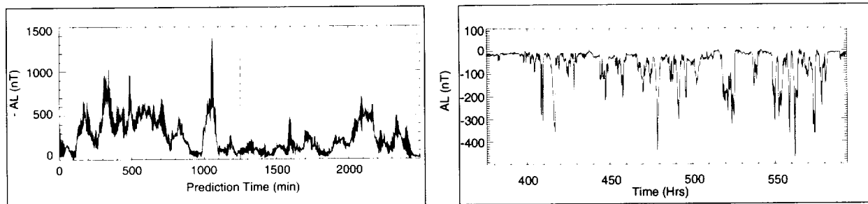
Predictions of AL index using (left panel) the local-linear prediction method and (right panel) the Faraday loop model. The shaded area shows the difference between the predicted and measured AL. Note that -AL is plotted in the left panel.
