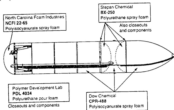
FIGURE 3. TPS Materials
