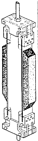
Figure 5. Cryostrain Test Apparatus
