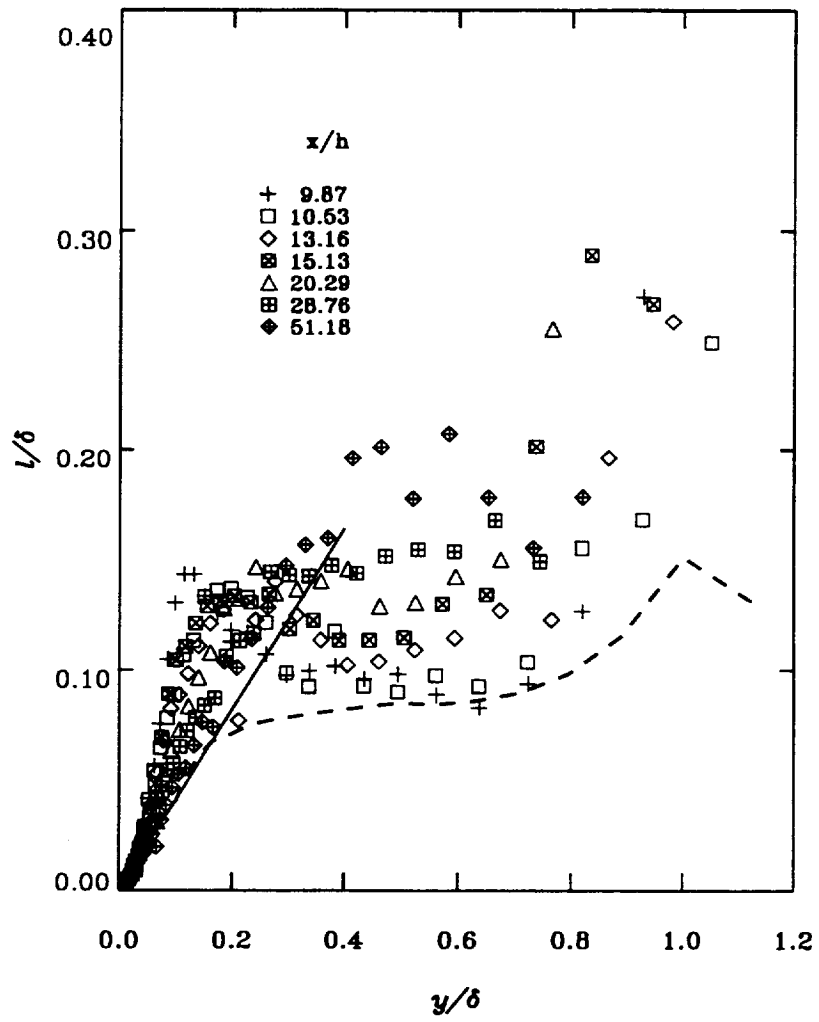
Figure 20. Development of the internal boundary layer: profiles of mixing length and eddy viscosity. Dash line represents upstream TBL. (a) Mixing length (solid line presents 0.41y).
