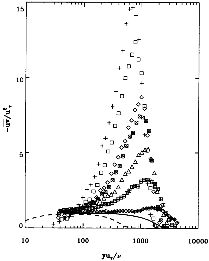
Figure 10. Concluded. (d) Shear stress. All symbols are same as in figure 10(b).
