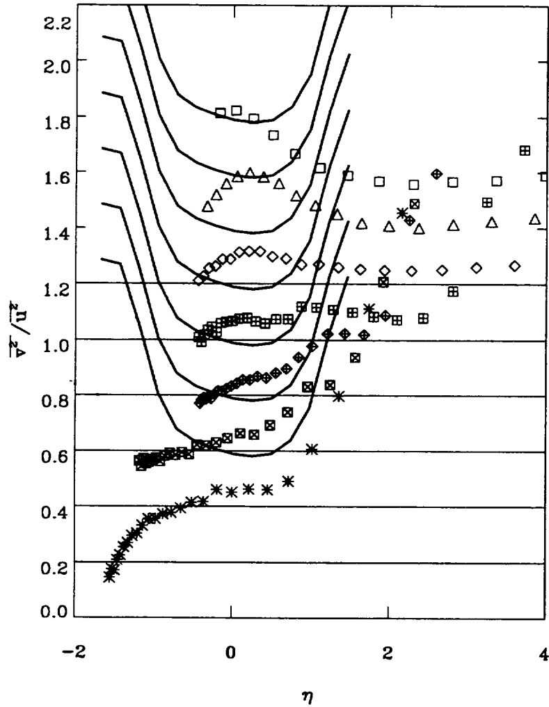
Figure 7. Concluded. (b) Intensity ratio \frac{v^2}{u^2} . All symbols are same as in figure 5(a).
