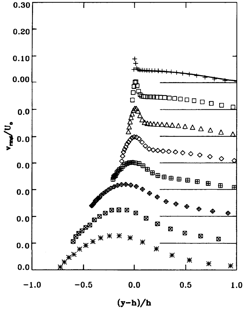
Figure 3. Continued. (c) v_{rms} = \sqrt{v^2} . All symbols as in figure 3(b).
