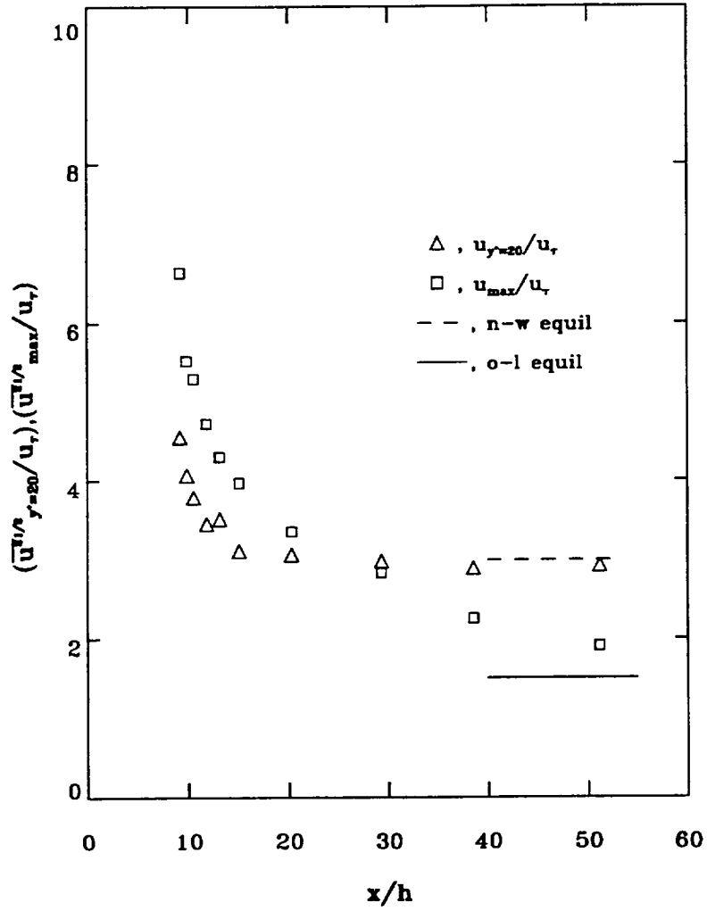
Figure 11. Development of maximum values in the reattached flow. (a) u_{rms} = \sqrt{u^2} ; local maximum in outer layer, and value at y^+ = 20 . n-w equil, near wall equilibrium; o-l equil, outer layer equilibrium.
