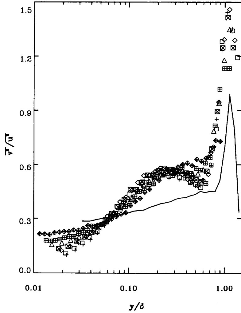
Figure 13. Continued. (b) Intensity ratio \overline{v^2}/\overline{u^2} .
