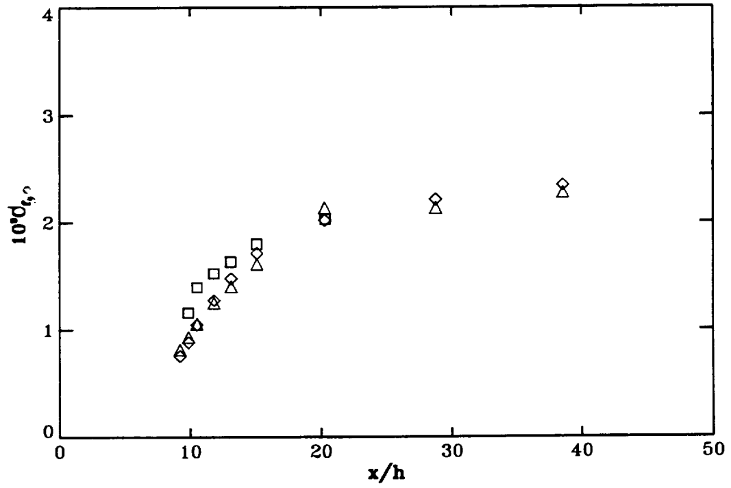
Figure 2. Concluded. (c) Comparison of C_f determined in three different ways: □, LOI-present experiment; △, Ludwig-Tillmann; ◇, Clauser chart.
