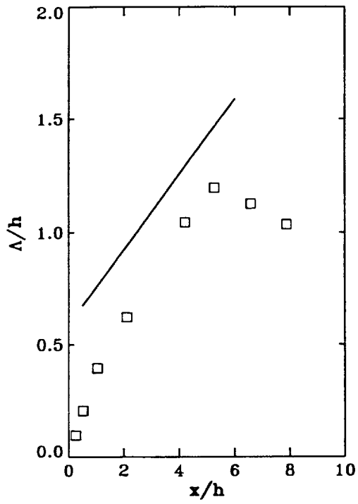
Figure 4. Scaling parameters for internal mixing layer. (a) Shear layer vorticity thickness; solid line depicts plane mixing layer, (b) internal mixing layer growth.
