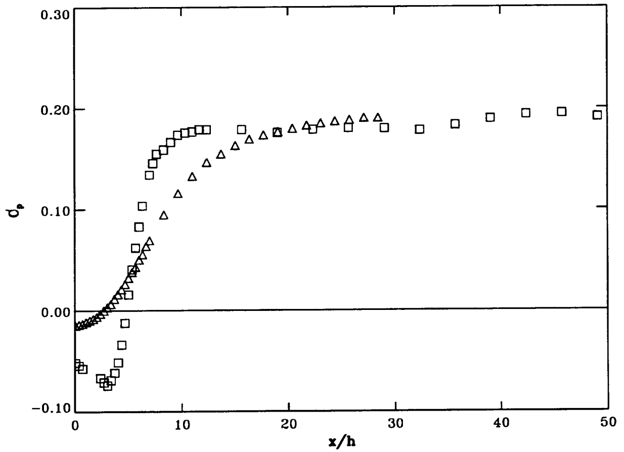
Figure 2. (a) Pressure coefficient. \square , bottom wall; \Delta , top wall.
