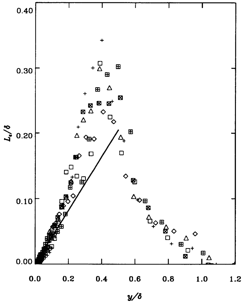
Figure 22. Development of the internal boundary layer: profiles of dissipation length parameter L_\varepsilon = (-\overline{uv})^{3/2} . All symbols are same as in figure 20(a).
