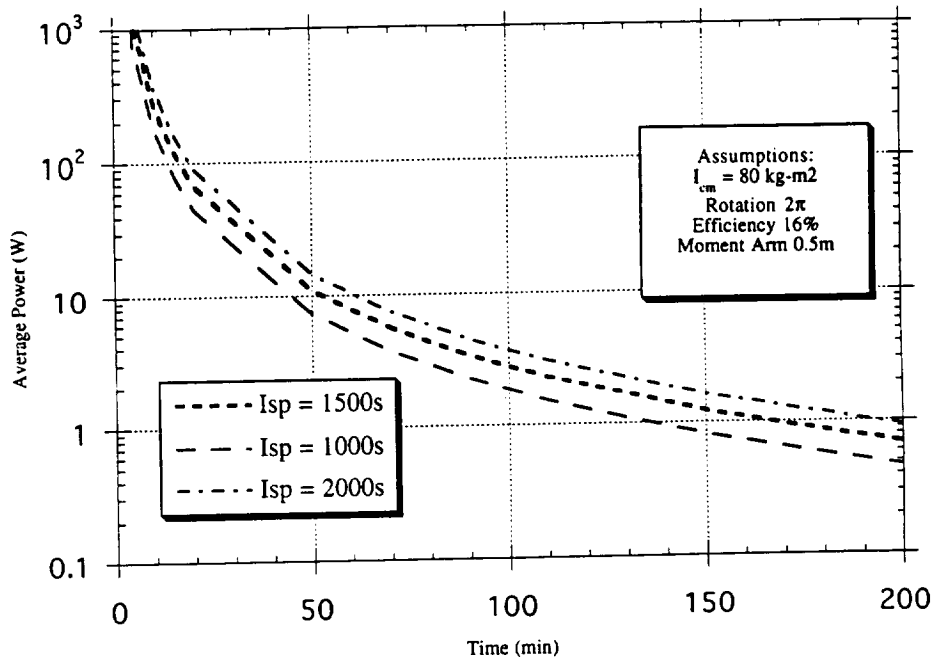
Figure 4-4: PPT System Power Levels for Time to Accomplish 2\pi Slewing Maneuver
