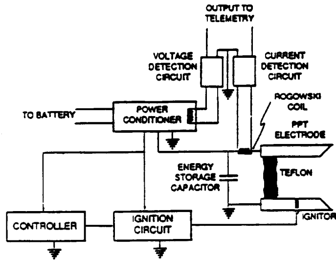
Figure 3-1: PPT flight system schematic. Telemetry signals depend on application.
