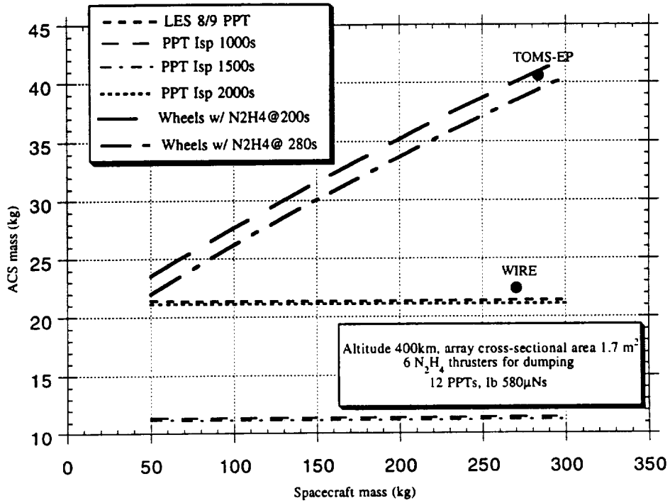
Figure 4-2: Attitude Control System Mass for Varying Spacecraft Mass
