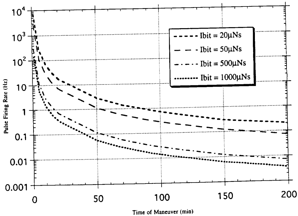
Figure 4-5: Pulse Firing Rates of Differing Impulse Bits for 2\pi Maneuver Times
