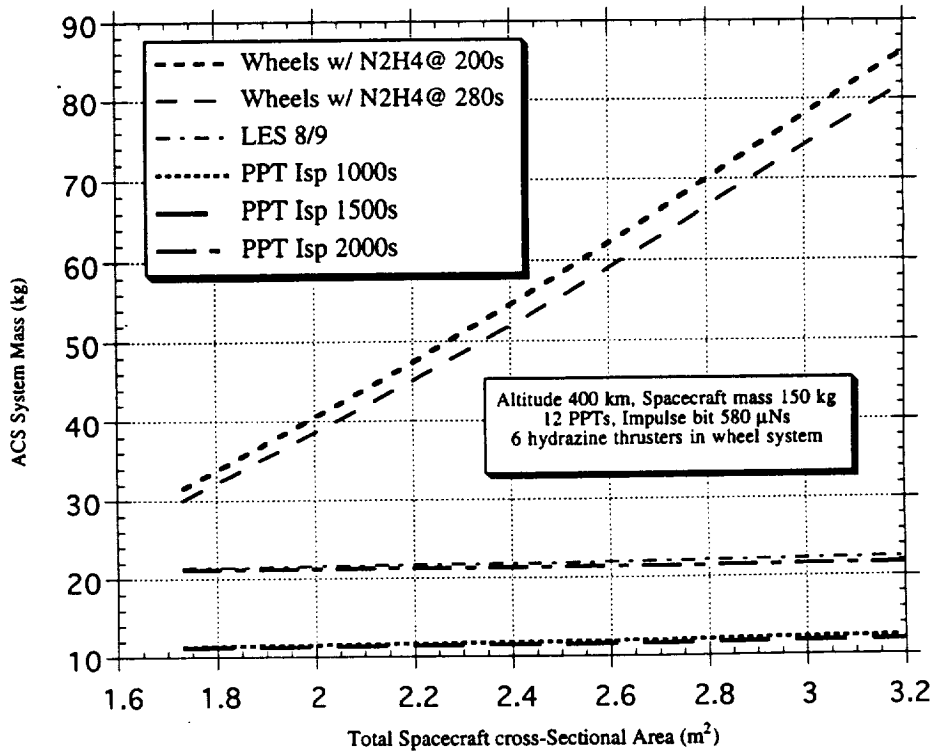
Figure 4-3: Attitude Control System Mass for Varying Array Cross-Sectional Area
