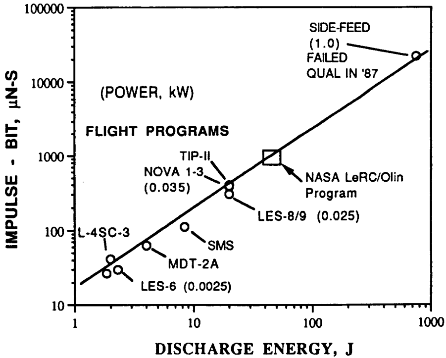
Figure 3-2: Impulse bit vs. stored energy for a range of flight and flight-qualified PPT systems.
