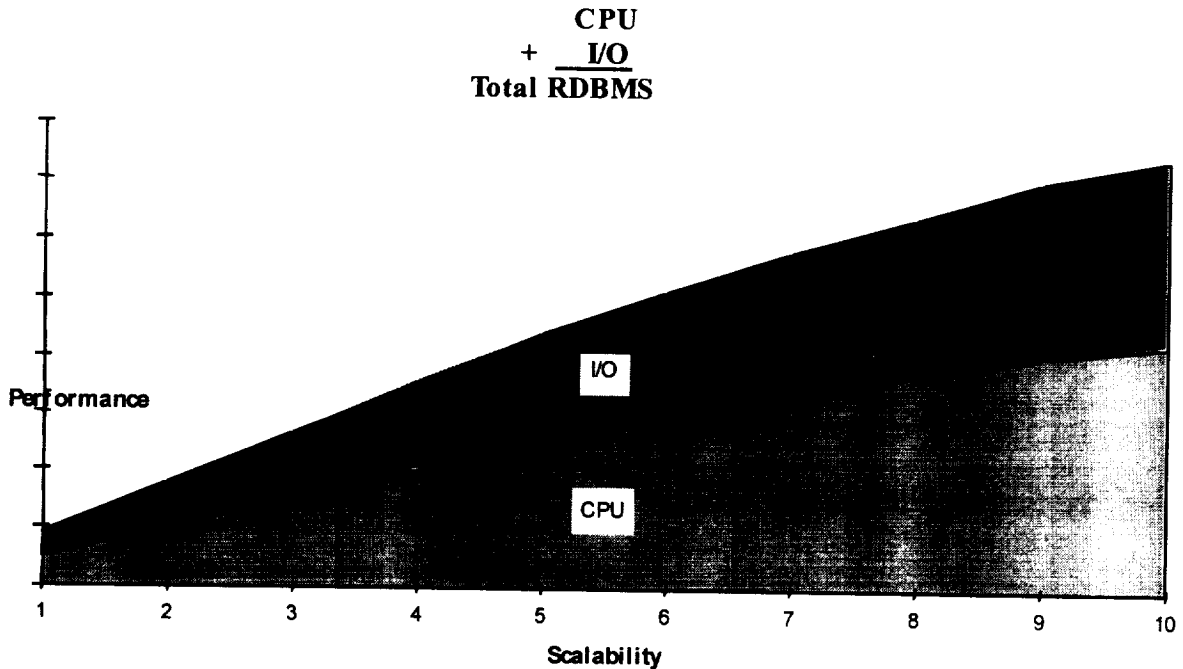
Figure III - RDBMS Performance
