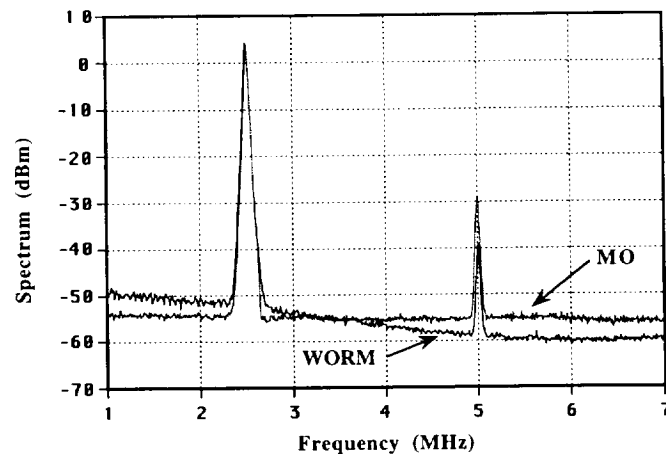
Figure 8. The readout spectrum is shown for WORM and MO readout for a 2.5 MHz tone at a media velocity of 12 m/s. The recording power is 5.1 mW for WORM and 5.0 mW for MO. The read powers are 1.0 and 1.5 mW for WORM and MO readout respectively.
