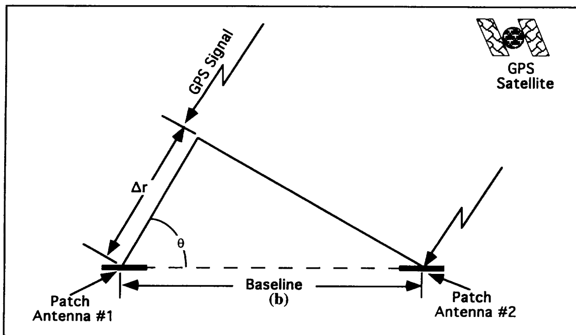
Figure 1. GPS Interferometry
