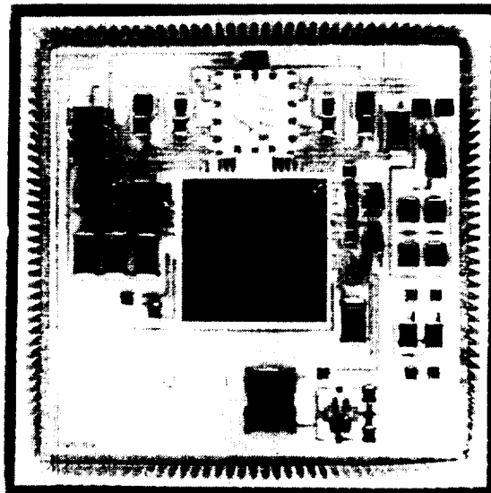
Figure 3. 1 inch by 1 inch Gyro and ASIC Package
