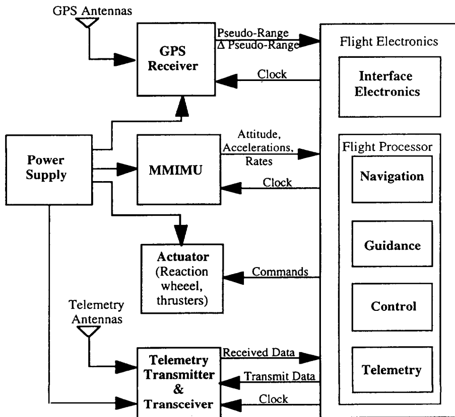
Figure 2. INS/GPS Subsystem
