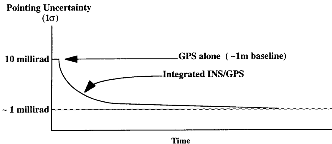
Figure 4. Pointing Accuracy with Integrated INS/GPS
