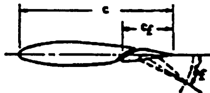
Figure 8.16 Single Slotted Flap Geometry
