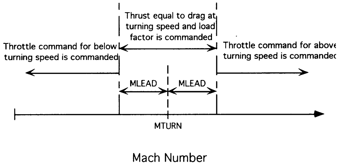
Figure B.4. Throttle Command As A Function OF Mach Number
