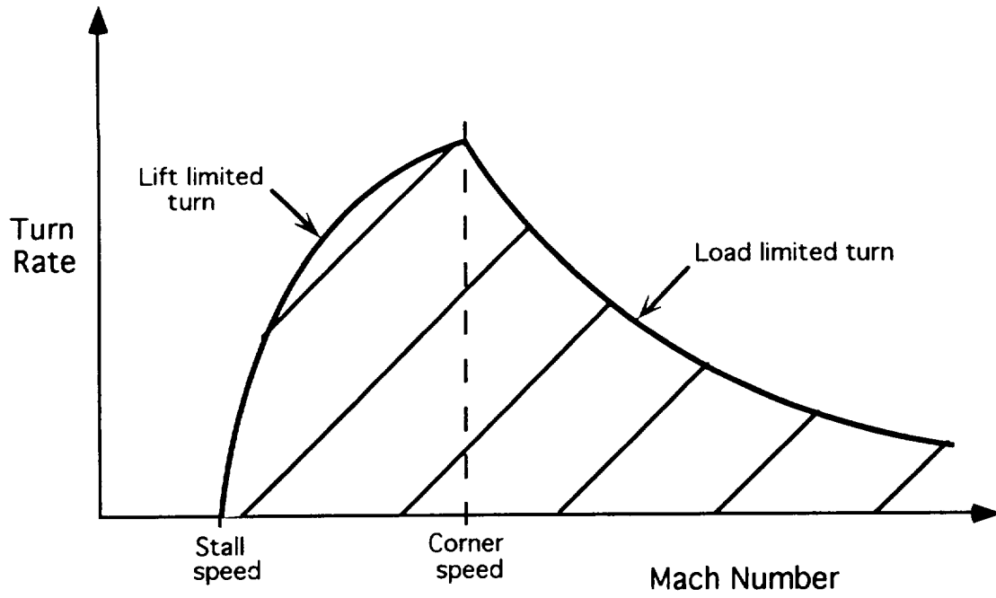
Figure B.2. The Doghouse Plot
