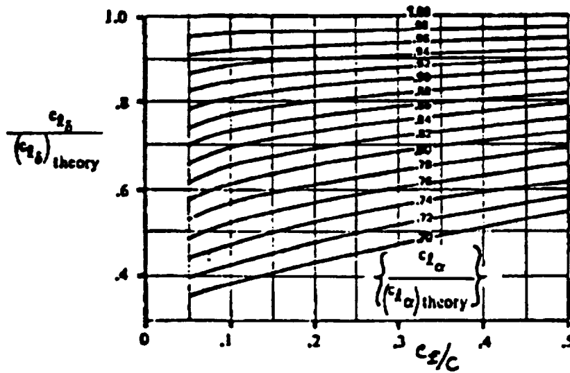
Figure 8.15 Correction Factor for Plain Flap Lift
