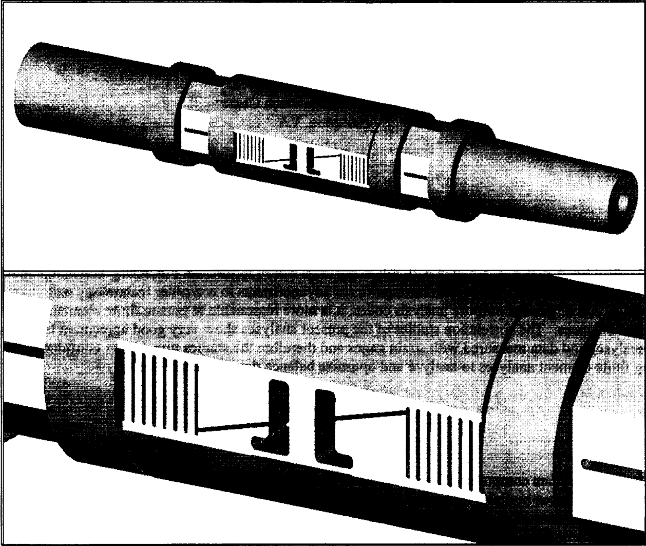
Figure 1. Pro/Engineer geometry model of NTF balance 101A.
