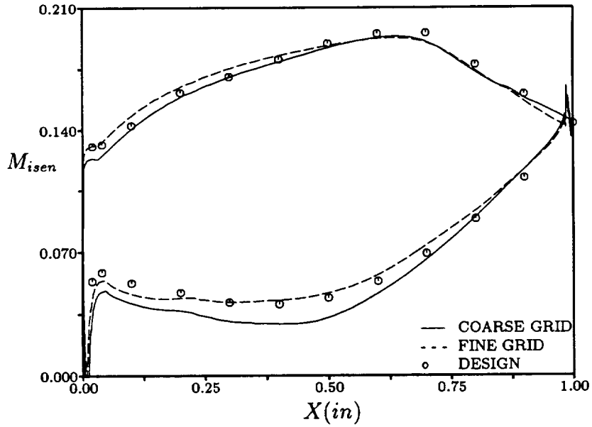
Figure 3: Surface (isentropic) Mach number distribution for PAK B turbine - Re = 40,000 , turbulent
