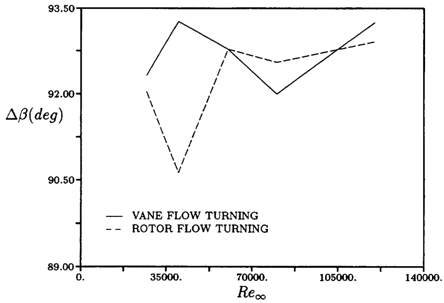
Figure 61: Flow turning angles; Baldwin-Lomax - fixed transition
