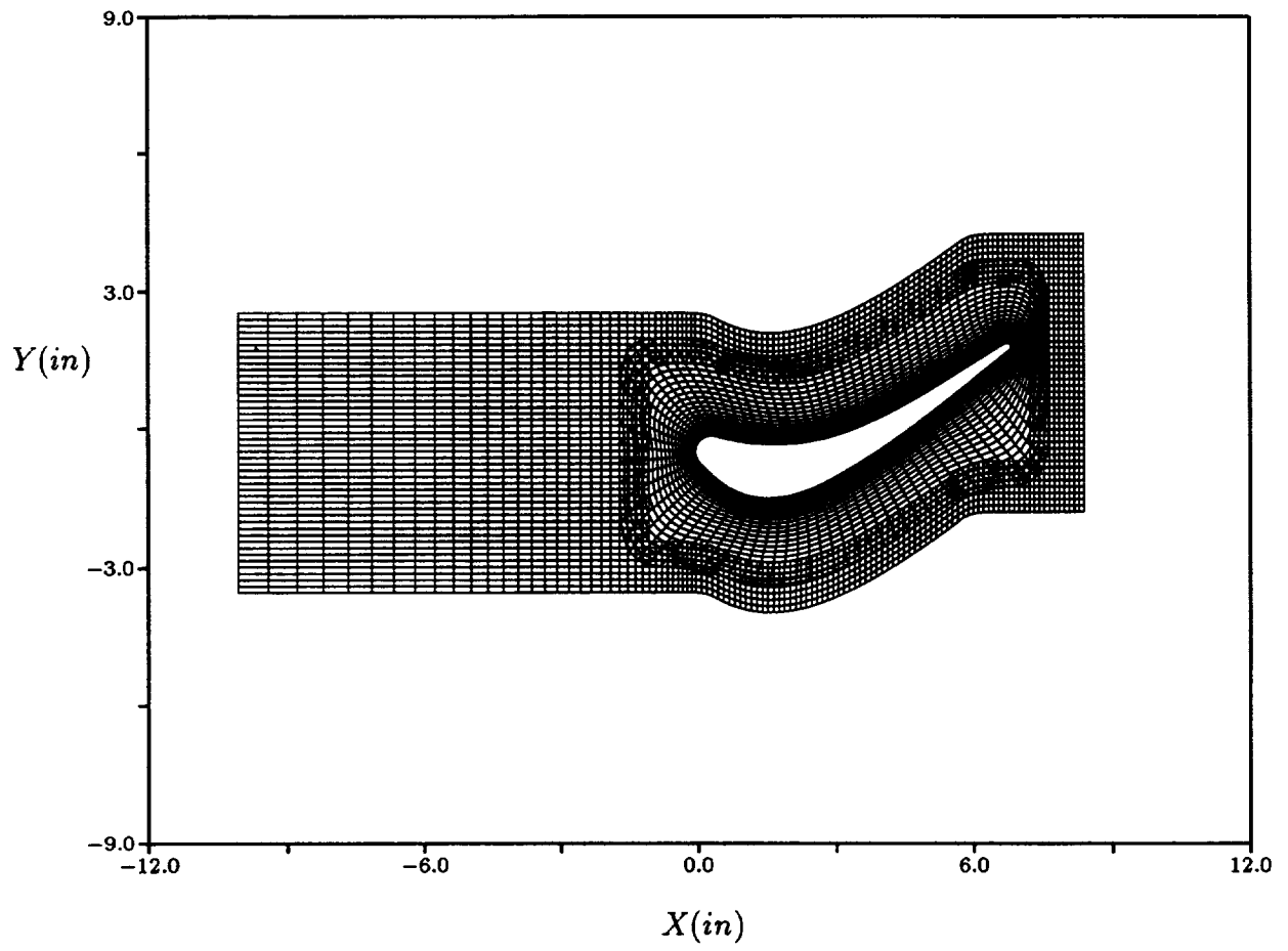
Figure 31: Modified LSRR geometry used to generate wake
