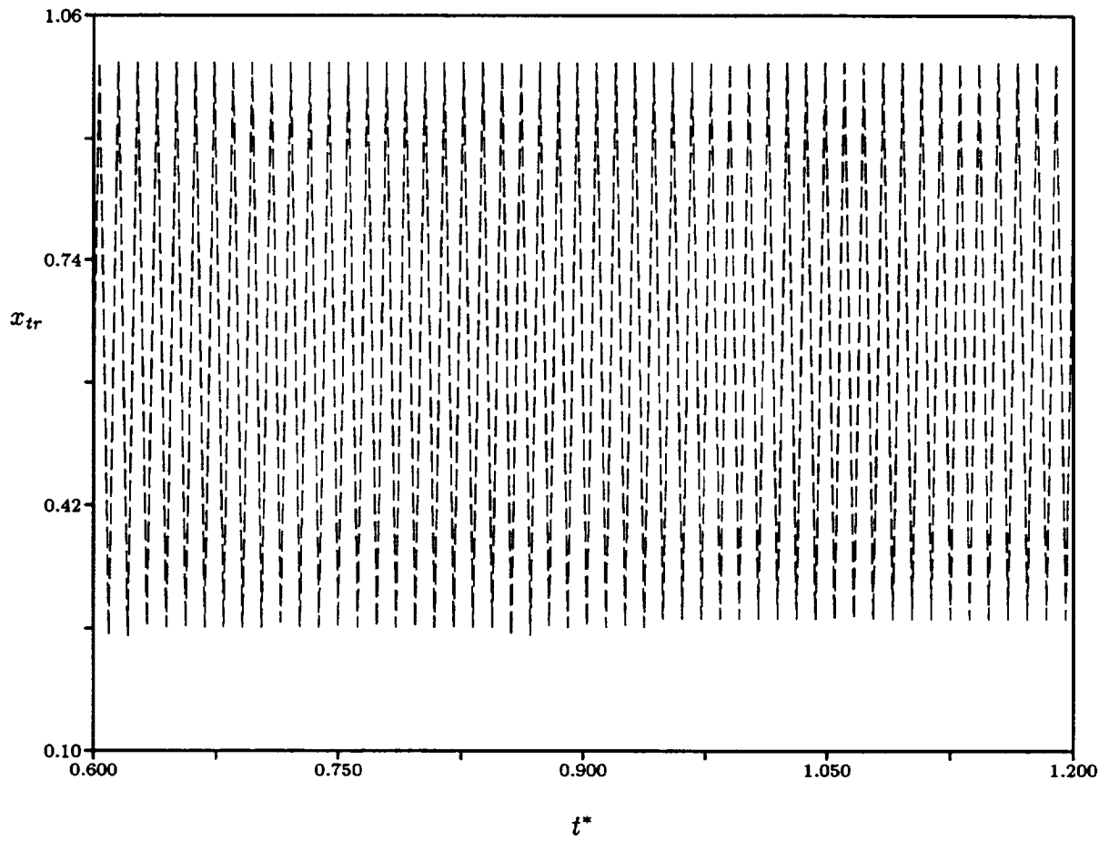
Figure 43: Close-up of time-variation of pressure surface transition location - Re = 40,000 , LSRR stator wake
