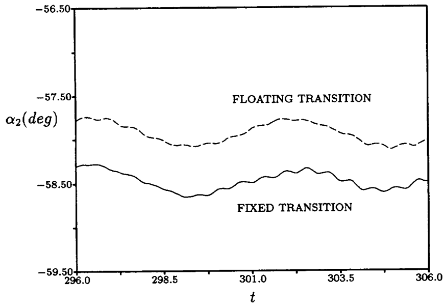
Figure 50: Exit flow angle variation for the PAK B turbine blade - Re = 120,000 , LSRR stator wake
