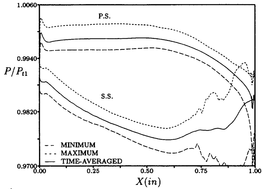
Figure 9: Surface pressure envelope for PAK B turbine - Re = 40,000 , laminar
