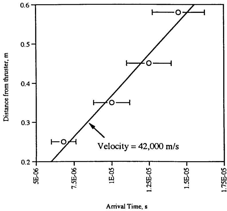
Fig 6 - Time-of-flight ion velocity measurements along plume centerline.
