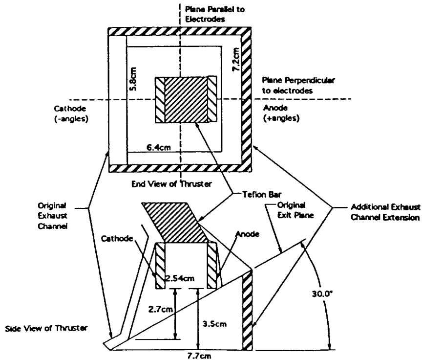
Fig. 2 - LES 8/9 electrode and exhaust channel schematics showing both the original exit plane and exhaust channel extension. Note planes parallel and perpendicular to electrodes.
