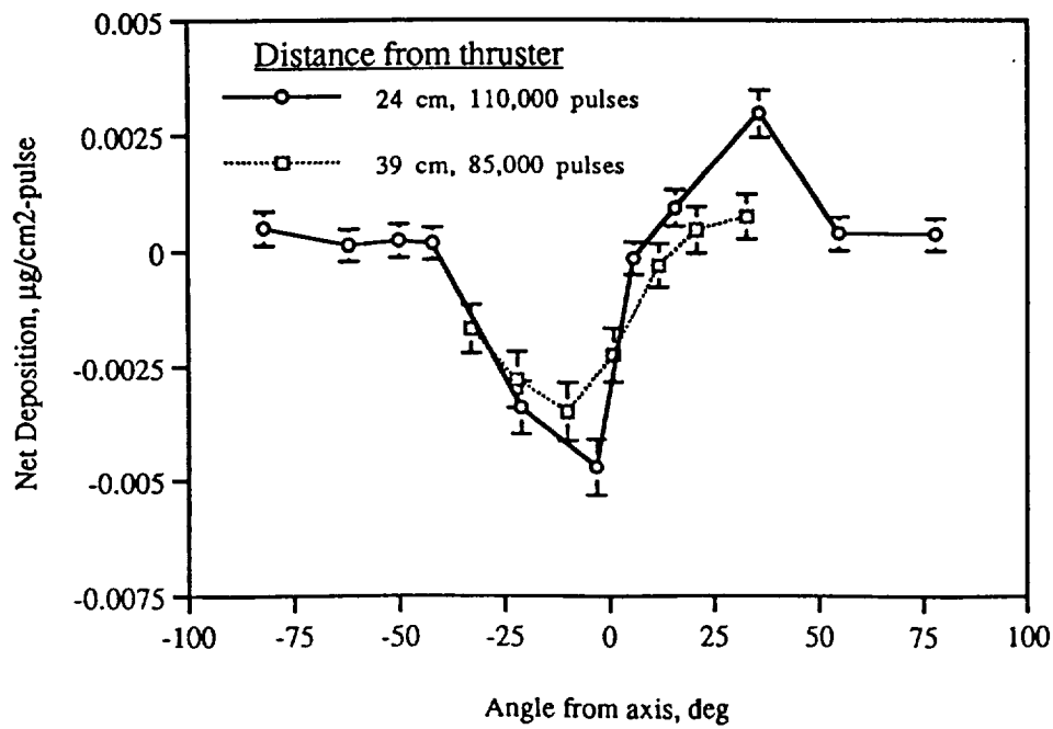
Fig. 8 - Net deposition on quartz slides in near-field region.
