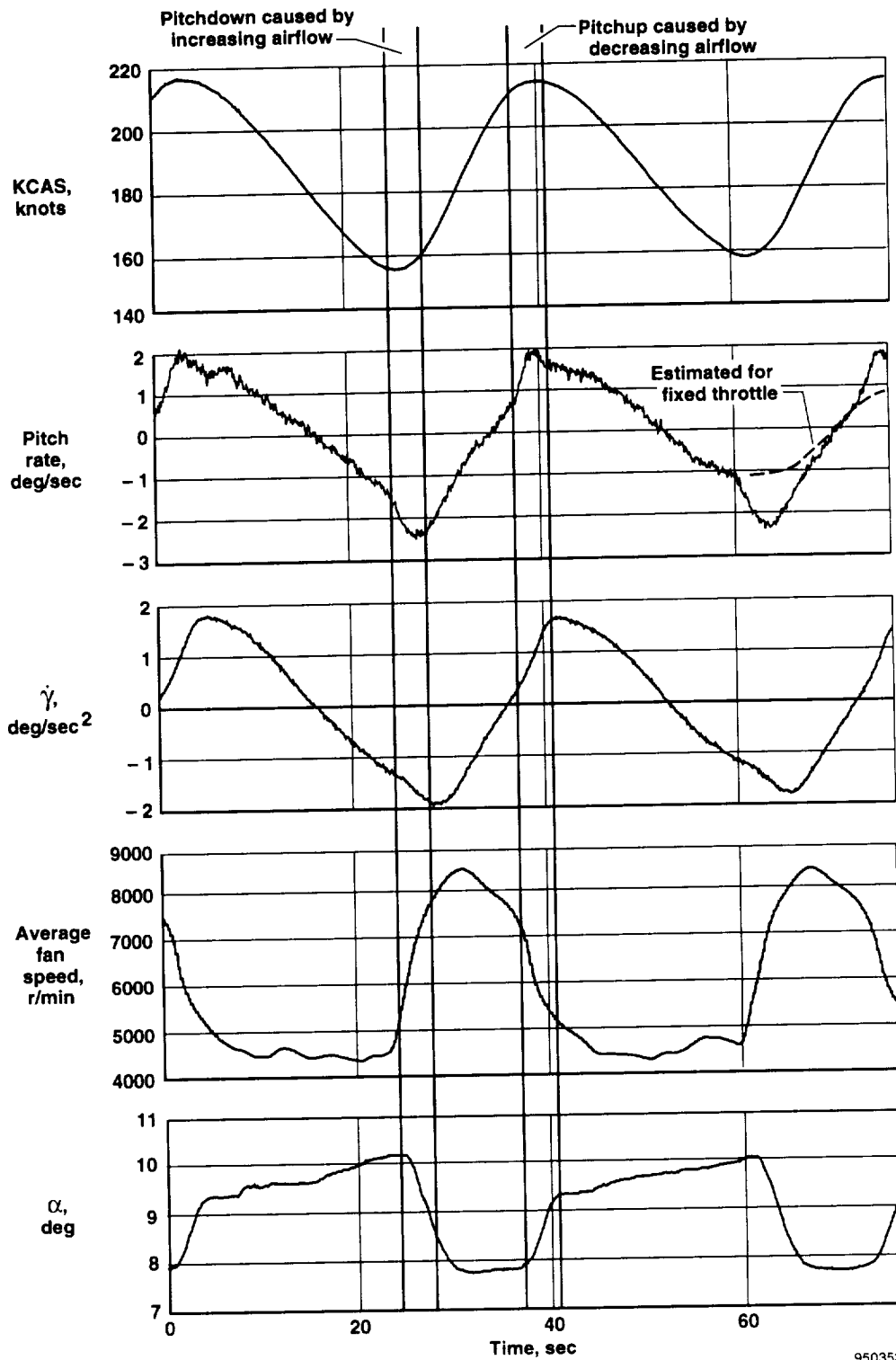
Figure 39. An F-15 PCA pitch oscillation caused by inlet effect, gear up, flaps up, PCA trim on, velocity feedback off and inlets emergency.
