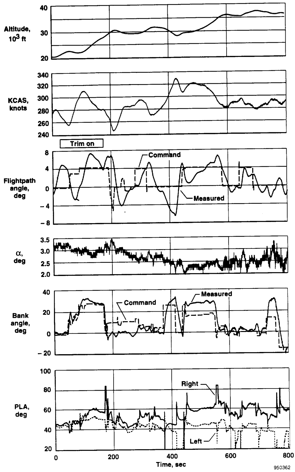
Figure 45. Time history of PCA climb at KCAS = 280 knots, flaps up.
