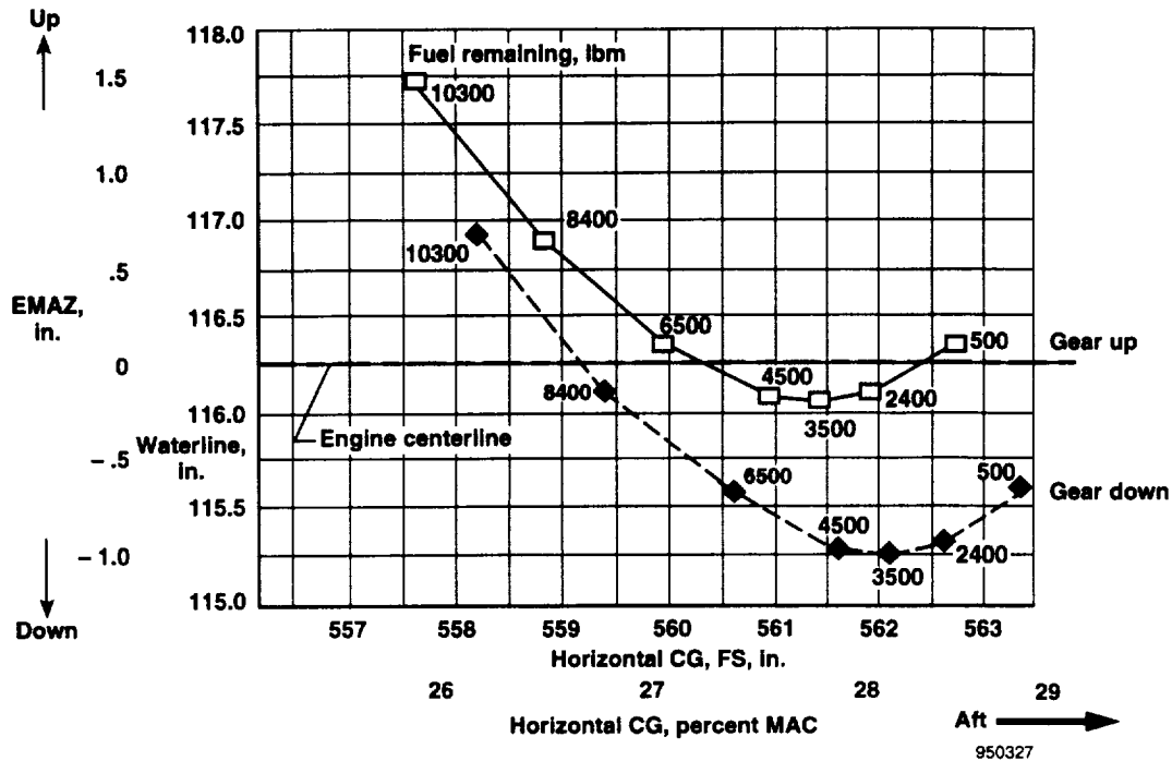
(b) Vertical and horizontal CG for the NASA F-15 HIDE C airplane.
