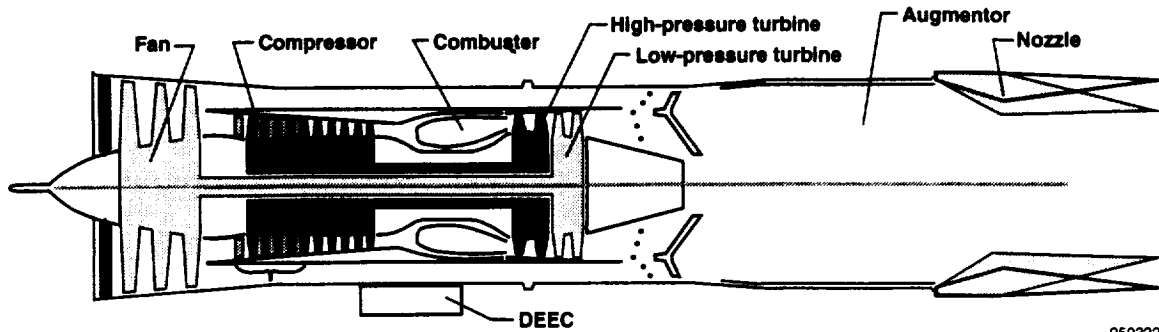
(a) Cutaway view.
