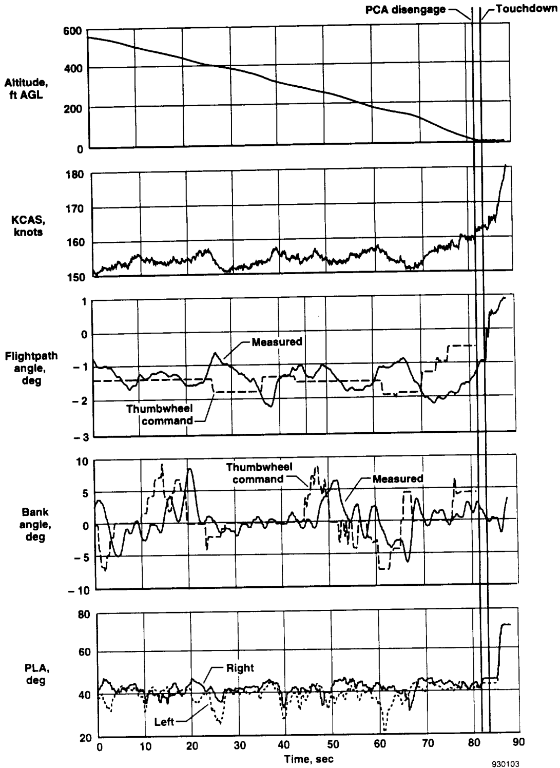
(a) Eighty-three seconds of landing approach.
