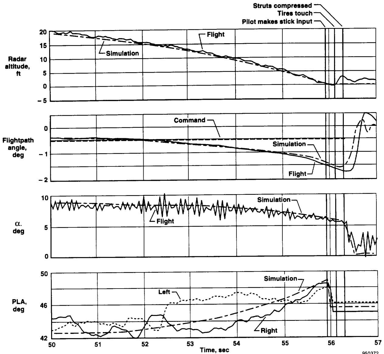
Figure 53. Comparison of final simulation to final 6 sec of PCA landing of figure 37.
