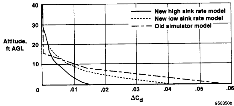
(b) Change in drag coefficient caused by ground effect.
