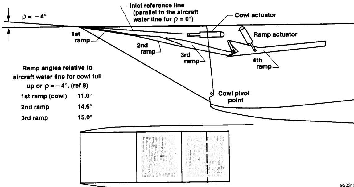
(a) The F-15 inlet in the full-up "emergency" position.
