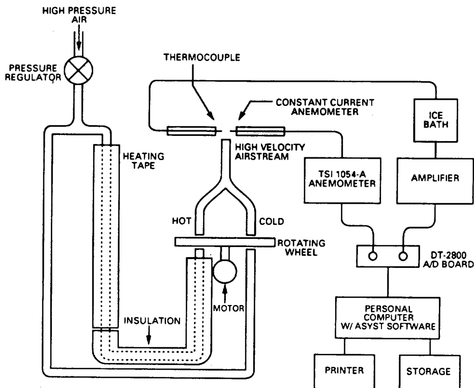
FIG. 2. Schematic of rotating wheel apparatus.
