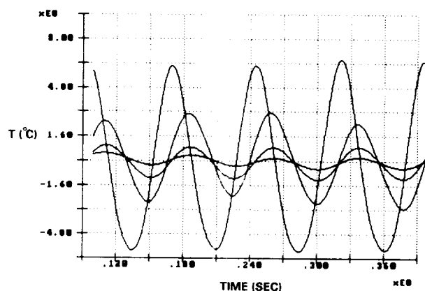
FIG. 3. Temperature profiles for the gas (large amplitude) and three type-K thermocouple wires. Three wires: D_1 = 50.8 \mu\text{m} , \omega_1 = 42 \text{s}^{-1} , D_2 = 101.6 \mu\text{m} , D_3 = 203.2 \mu\text{m} . Gas temperature frequency: \omega = 86 \text{s}^{-1} .
