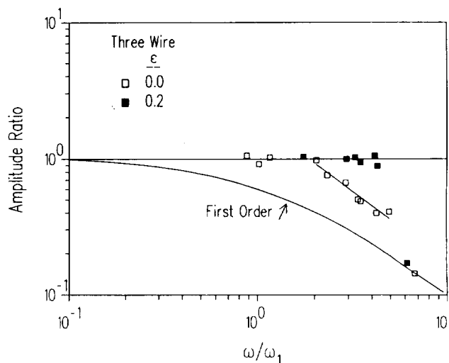
FIG. 7. Amplitude ratio of three-wire thermocouple output-to-true gas temperature. Also shown is first-order response of small wire.
