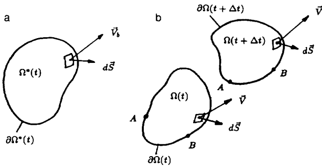
FIG. 1. Definition of a control volume and material volume. (a) Control volume, denoted by \Omega^*(t) , may be nonstationary, e.g., on rotating frame. (b) Material volume, \dot{V}_b = \dot{V}
