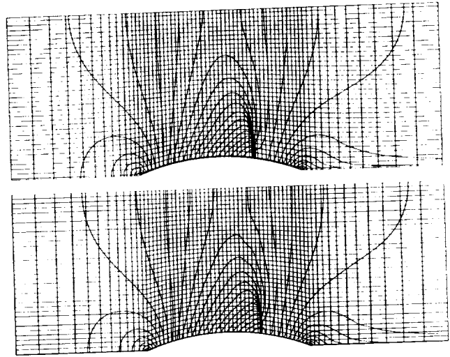
FIG. 6. Mach contours for M_x = 0.675 , 10% bump flow; (a) Lagrangian solution ( 134 \times 70 grid), (b) Eulerian solution ( 266 \times 138 grid). (Contour levels: M_{\min} = 0.0 , M_{\max} = 1.6 , \Delta M = 0.04 .)
