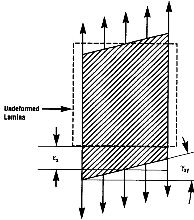
Figure A-1. Deformation of a 45^\circ lamina subject to a uniform stress.
