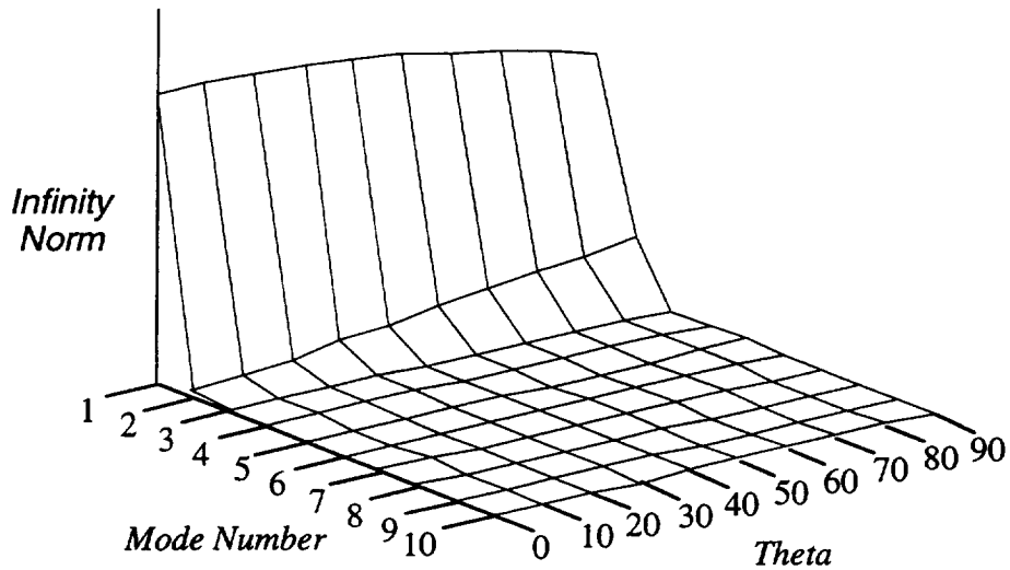
Figure 2.6.1 Infinity Norm of Bode Response as a Function of Mode Number and Theta - Heavy Payload
