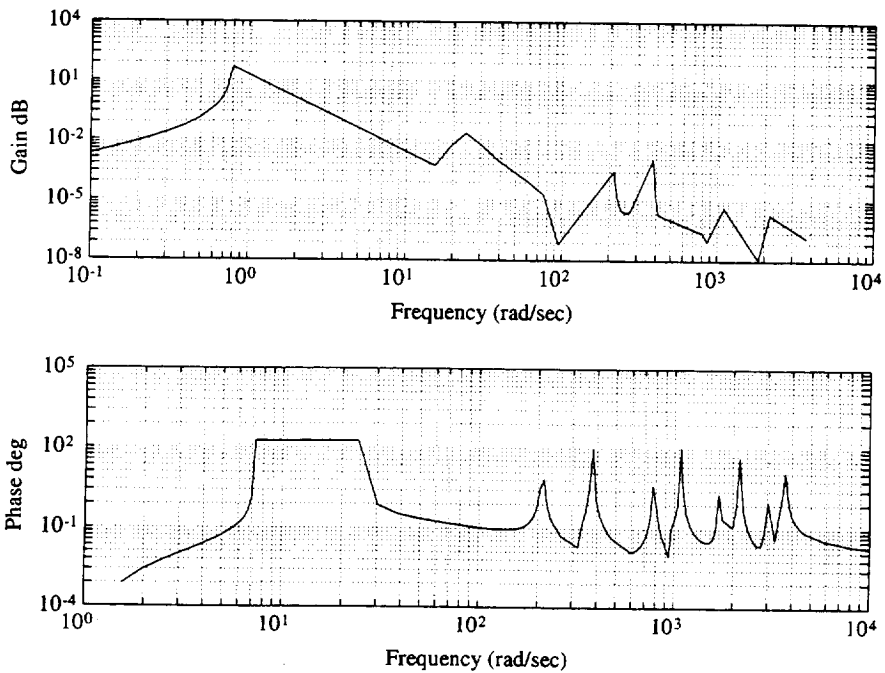
Figure 4.6.3 Maximum Bound on the Additive Model Error E_a(j\omega)
