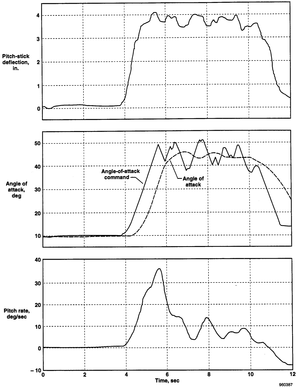
Figure 13. Time history from longitudinal gross acquisition.
