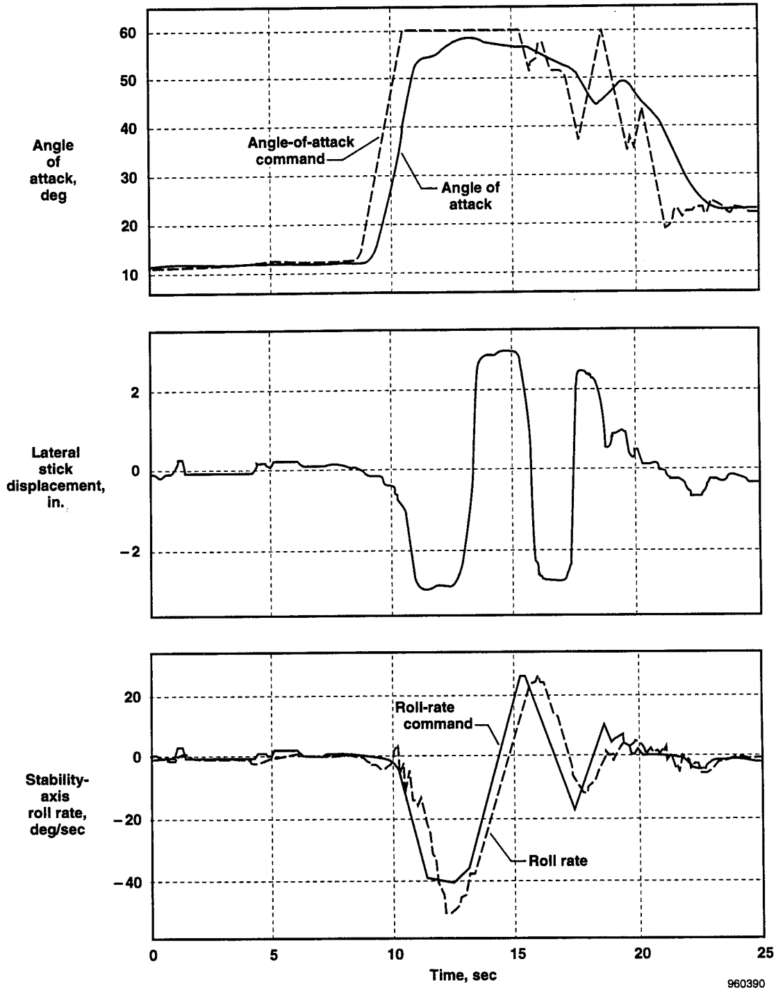
Figure 16. Time histories for lateral gross acquisition.
