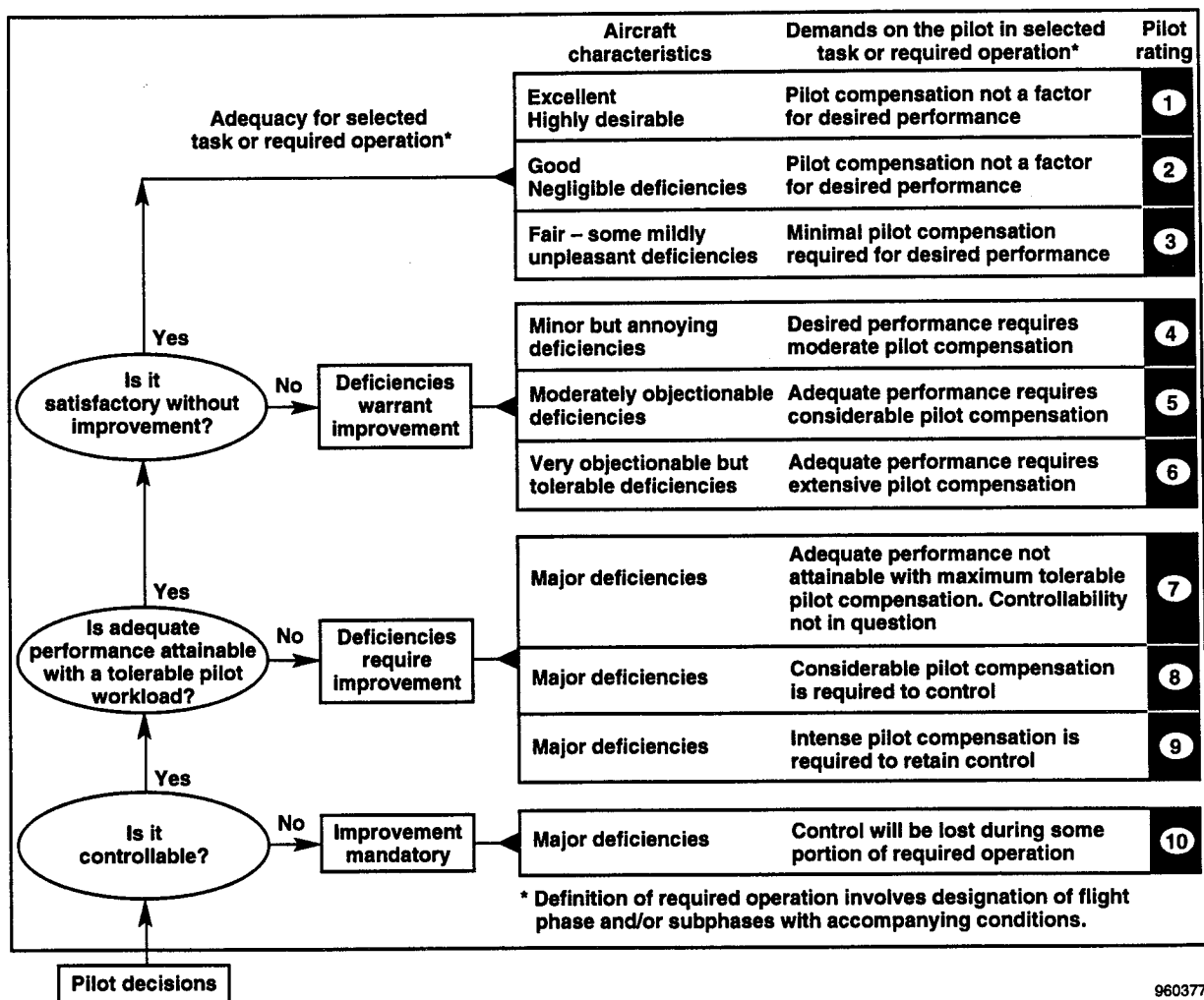
Figure 3. Cooper-Harper rating scale.
