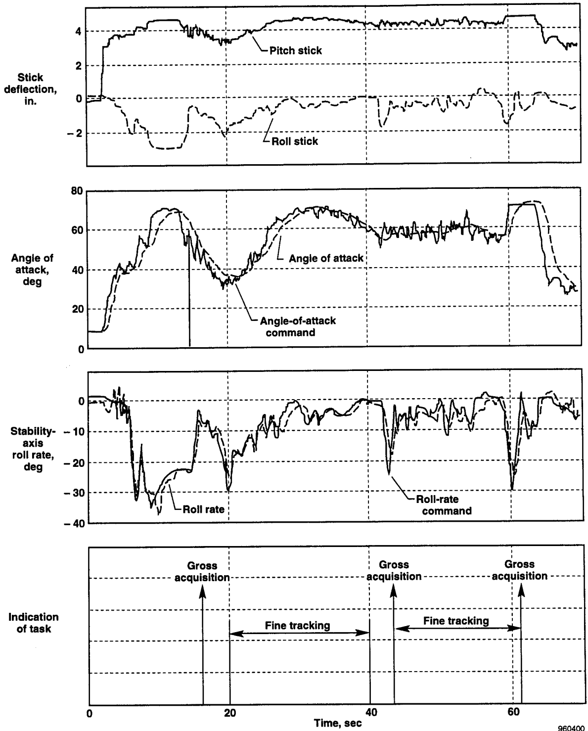
Figure 26. Time history from a combined maneuver.
