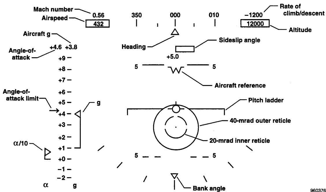
Figure 2. Head-up display symbology.
