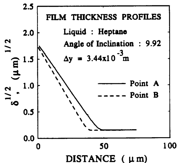
Figure 7. Film thickness profiles of Heptane at different positions (point A and B) for an angle of inclination equal to 9.92^\circ .
