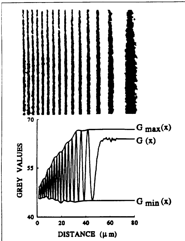
Figure 5. Interference fringes and the gray value plot.
