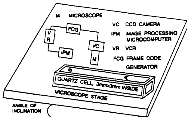
Figure 2. Experimental setup.
