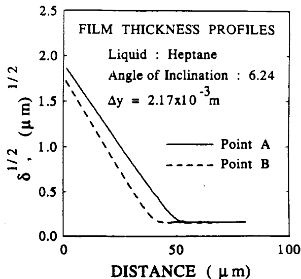
Figure 6. Film thickness profiles of Heptane at different positions (point A and B) for an angle of inclination equal to 6.24^\circ .
