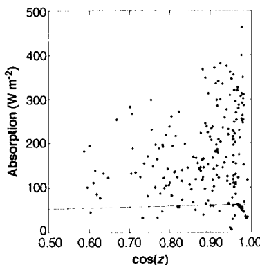
Fig. 2. Three-minute averages of cloud absorption determined by the difference between net flux at 20 km and at 10 km, from TOGA-COARE and CEPEX. The solid line indicates our estimate of clear-sky absorption.
