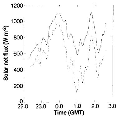
Fig. 1. Net solar flux measured at 20 km from the NASA ER-2 (solid curve) and at 10 km from the NASA DC-8 (dashed curve) over the tropical western Pacific during the TOGA-COARE flight on 31 January 1993.
