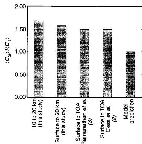
Fig. 5. Summary of estimates of (C_S)/(C_T) determined by this study, (2, 3), and model calculations.
