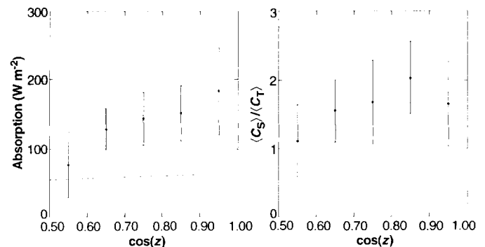
Fig. 3 (left). Averages in 0.1-wide cosine bins of the absorption data shown in Fig. 2. The solid line indicates our estimate of clear-sky absorption. Error bars denote the standard deviation of the sample, a measure of the range of variability in observed cloud absorption.
