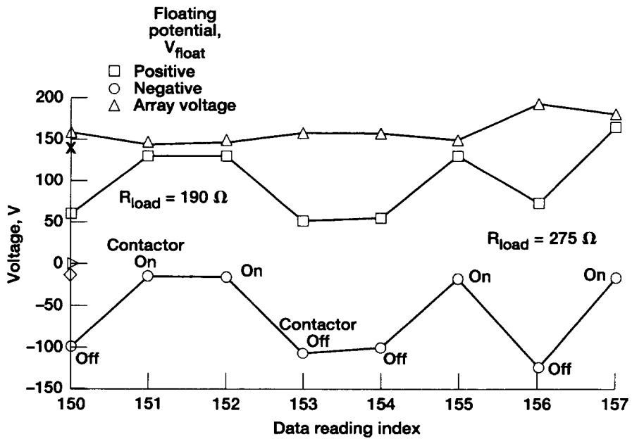
Figure 26.—Floating potentials.
