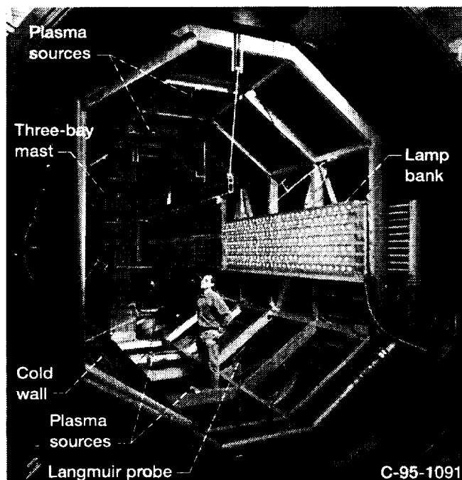
Figure 1.—Test cage assembly in tank 5.
