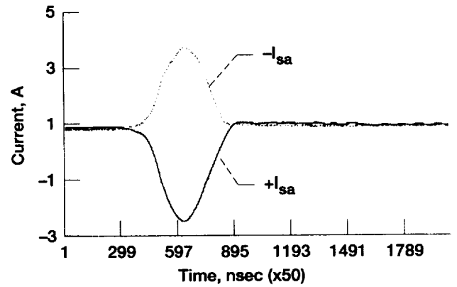
Figure 31.—Array current during arc.
