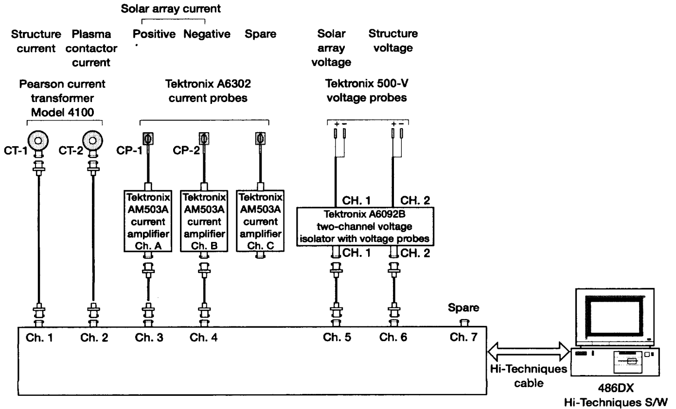
Figure 5.—Transient data acquisition system.
