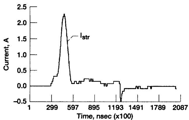
Figure 35.—Arc example 2.
