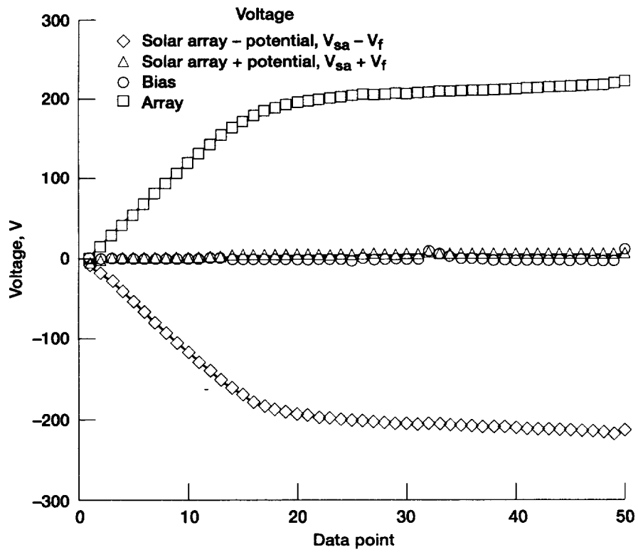
Figure 15.—Floating potentials.
