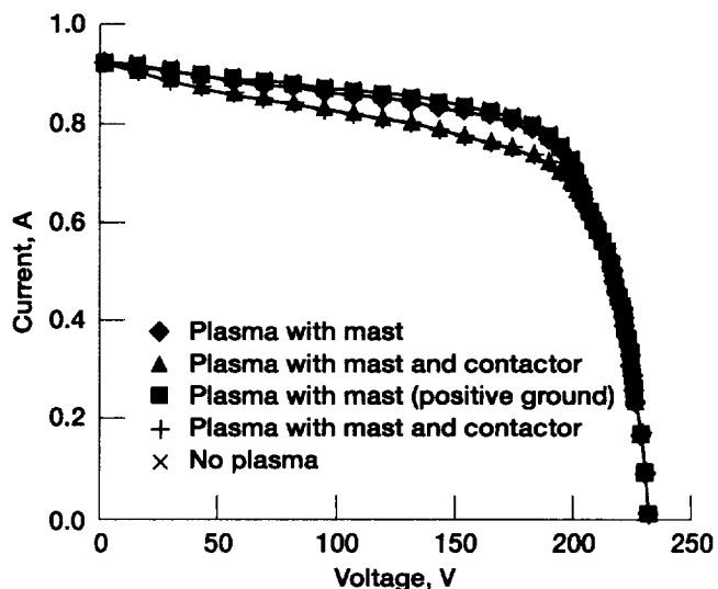
Figure 38.—Operation comparison.
