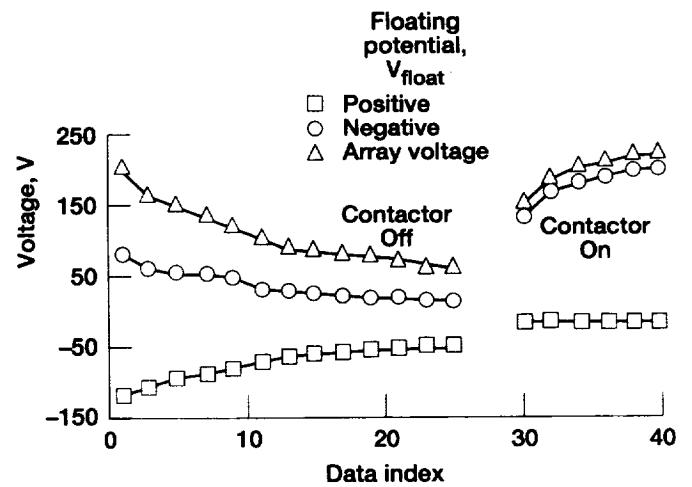
Figure 32.—Constant negative floating potential with contactor.
