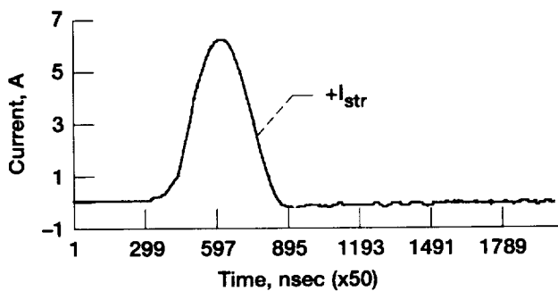
Figure 29.—Large arc.
