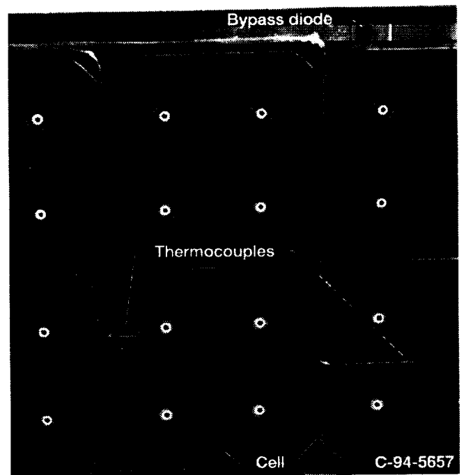
Figure 10.—Photovoltaic cell.
