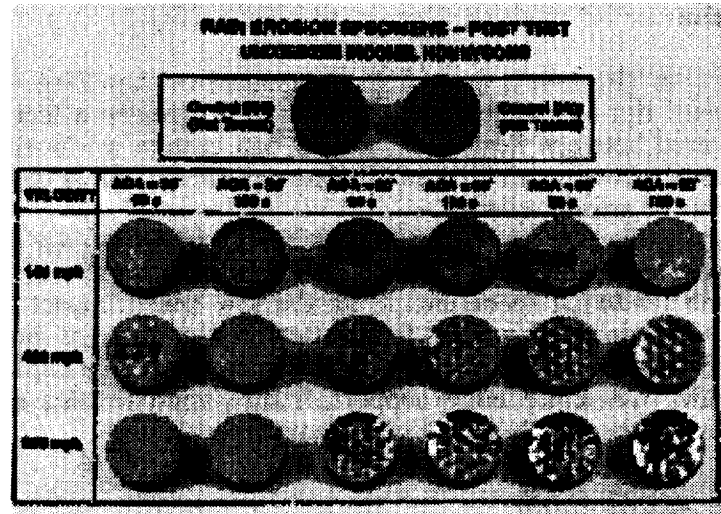
FIGURE 9. Inconel 617 Honeycomb Coupons Tested in Rotating Arm Rain Erosion Facility.
