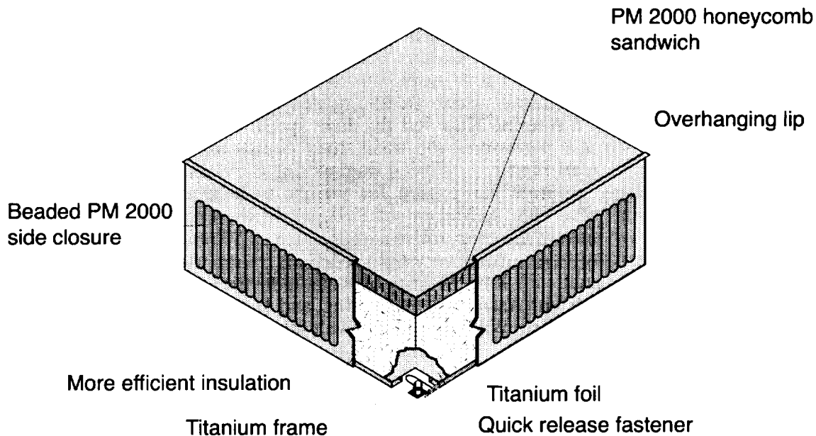
FIGURE 19. Next Generation Prepackaged Metallic TPS Panel.
