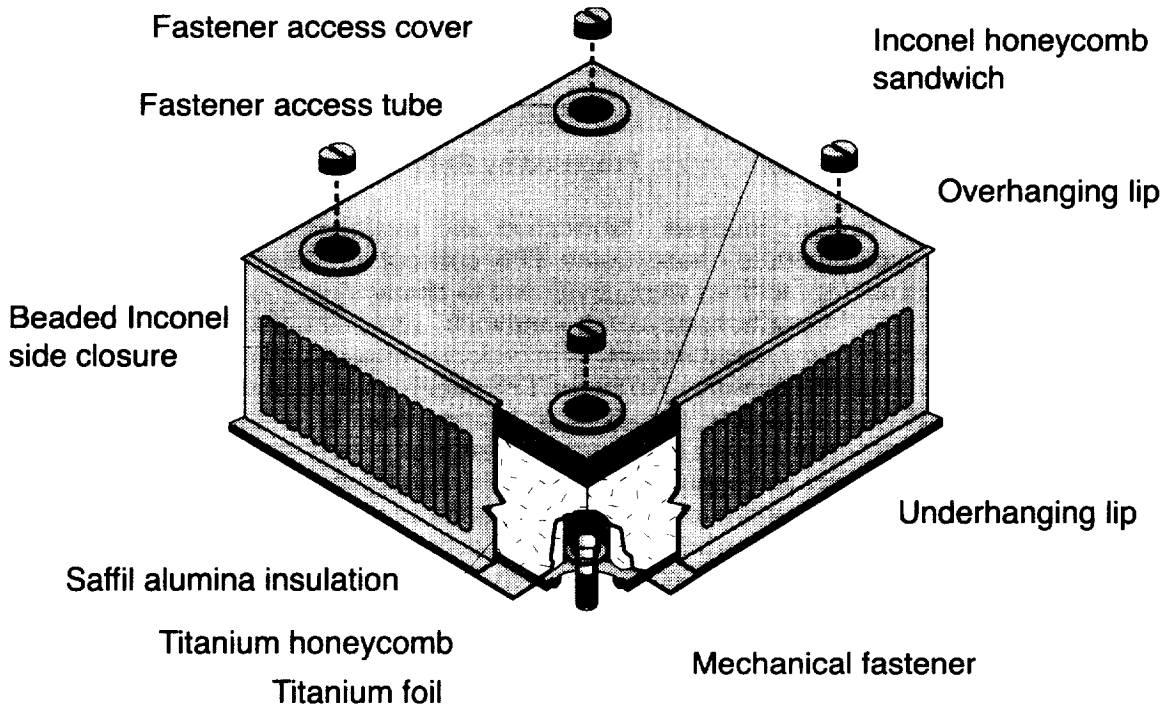
FIGURE 3. Prepackaged Superalloy Honeycomb TPS Panel.
