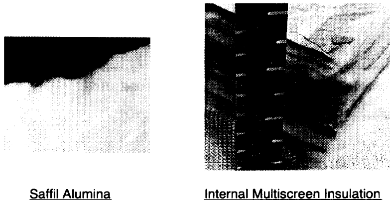
FIGURE 7. Internal Insulations for Metallic TPS.
