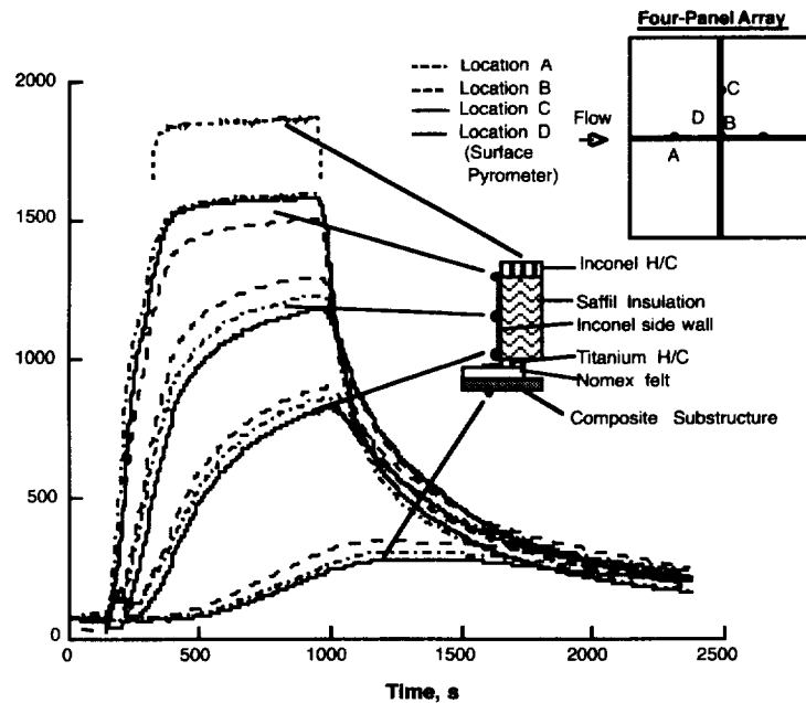
FIGURE 18. Temperature Histories Measure on Four Panel Array During Arcjet Test.
