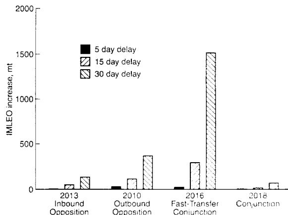
Fig. 2 Earth direct entry—Earth delay (chemical propulsion).
